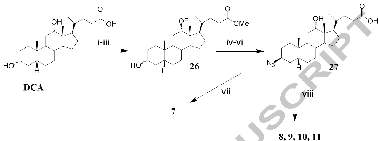
Scheme 2. Synthetic approaches to 7–11 from DCA
