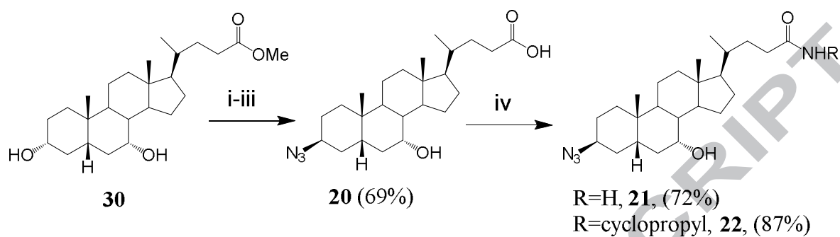
Scheme 5. Synthesis of 3-beta azido derivatives of CDCA 20 , 21 .
