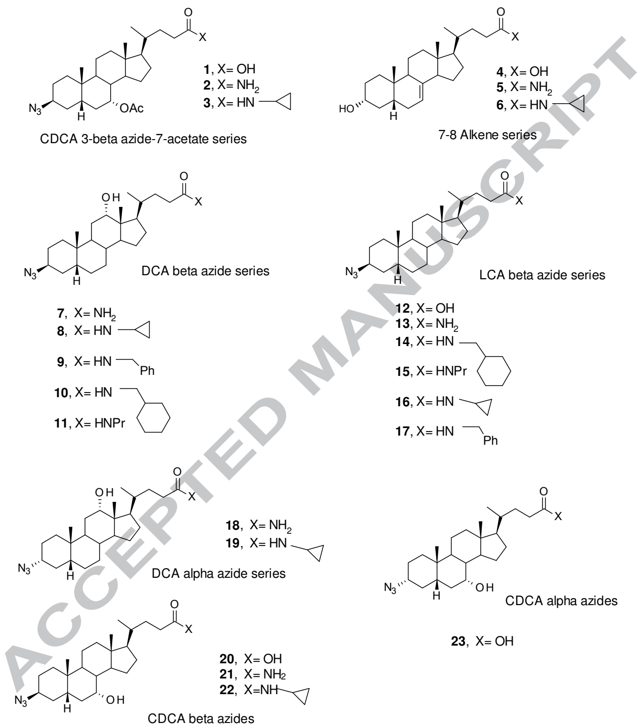
Figure 2. Structural formulae of the BA analogs studied
