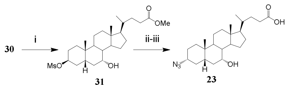
Scheme 6. Synthesis of 23 : PPh 3 , Et 3 N, MsOH, DIAD, anh THF, 0 °C, 2 d, 45 °C, 15%; (ii) NaN 3 , DMPU, 50 °C, 4 d, 79%, (iii) Aq 2M NaOH/MeOH (1:1), RT, 24 h, 88%
