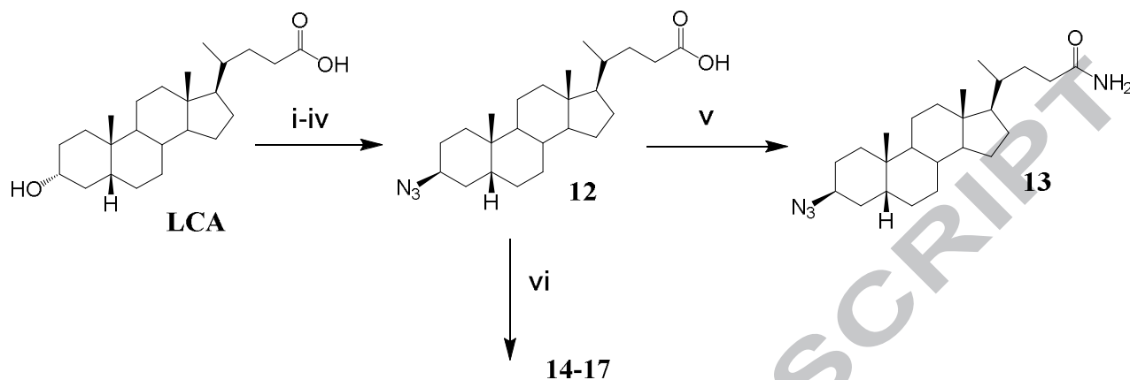
Scheme 3. Synthetic approaches to 12–17 from LCA
