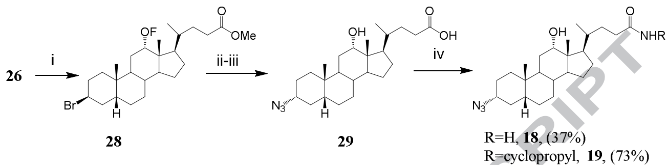
Scheme 4. Synthetic approaches to DCA 3 \alpha -azido amides 18 , 19 from 26
