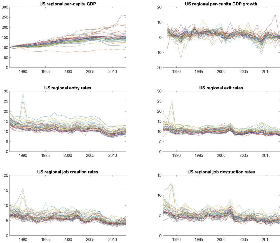
Figure 1: Regional US annual data for the 50 states and the District of Columbia, 1987-2013
