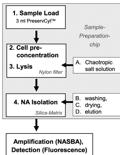
Fig. 3 Sample preparation assay implemented on chip.
