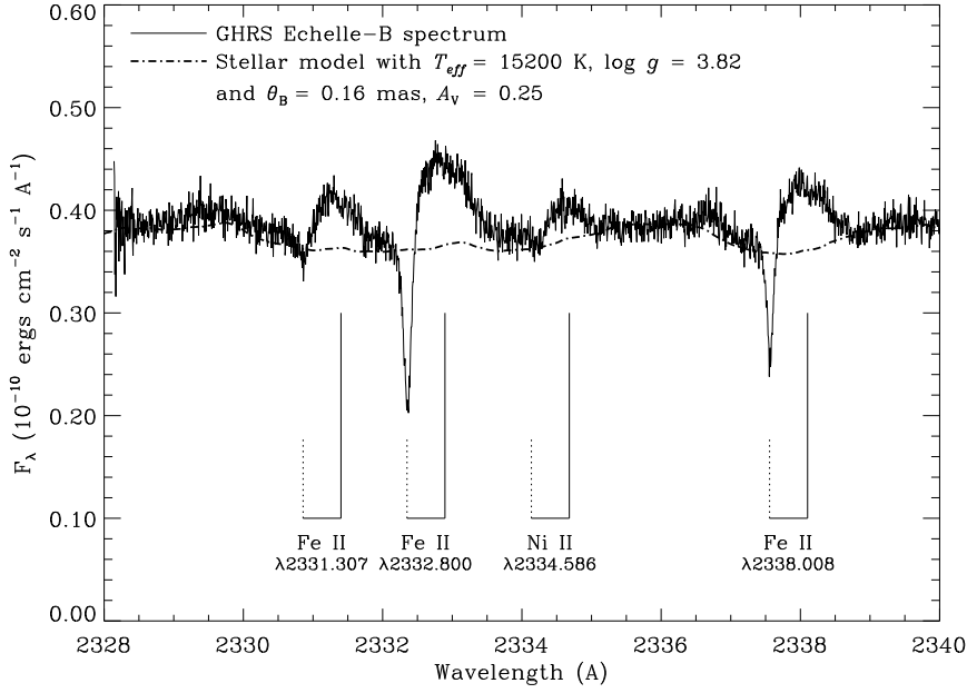
Figure 3. The spectrum of \zeta Aurigae B observed with the GHRB Ech-B at epoch 1. A synthetic spectrum of the photosphere of the B star has been superimposed to illustrate the extent of the emission in the wind lines of Fe II and Ni II. This spectrum was computed using the TLUSTY and SYNPEC codes of Hubeny (1988). The synthetic spectrum has been shifted by the radial velocity of the B star at epoch 1 ( +30.6 \text{ km s}^{-1} ). The lines of Fe II and Ni II are shown at the systemic velocity of the \zeta Aur system ( +12.2 \text{ km s}^{-1} , Griffin 1995) as a solid line, and at the terminal wind velocity of -70 \text{ km s}^{-1} relative to systemic as a dotted line.
