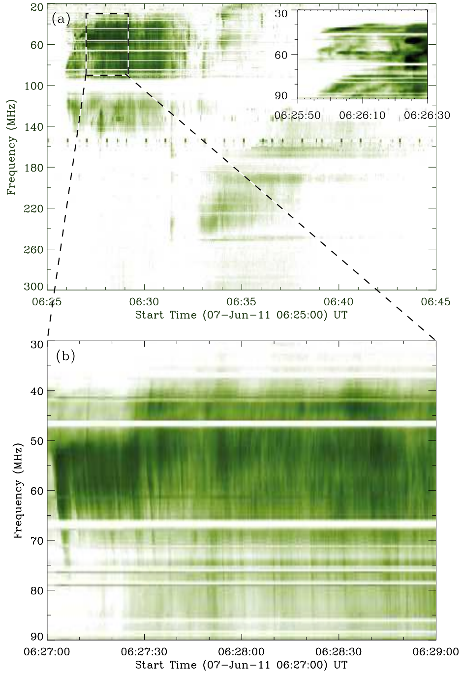
Figure 5. Dynamic spectrum of the 07 June 2011 Type II radio burst. In the inset of panel (a) a short-lived fundamental and harmonic backbones are visible. Multiple herringbone structure are visible at \sim 40 – 80 MHz in panel (b).
