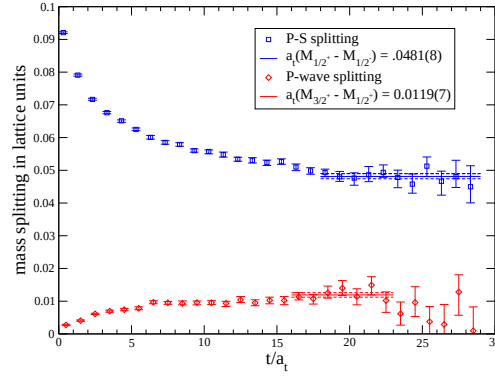
Figure 3: The mass-splitting between S and P wave states (blue points) and between the \frac{3}{2}^+ and \frac{1}{2}^+ P wave states (red points). The solid lines are best fits to the splittings (not the difference of fits to effective masses).
