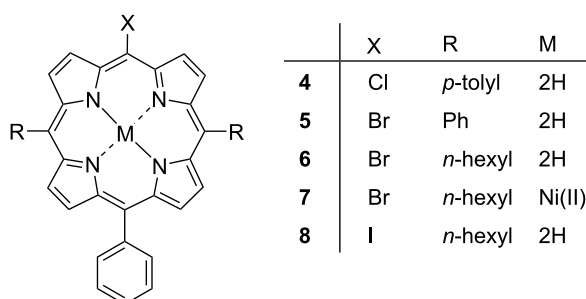
Figure 9: 5-Halo-15-phenyl-substituted porphyrins.
