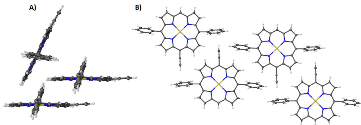
Figure 8: Expanded view (thermal ellipsoid plot) of compound 2A showing (A) the edge-on and stacking interaction between the porphyrin macrocycles and (B) layers of porphyrin with \uparrow \downarrow \uparrow \downarrow repeating pattern.
