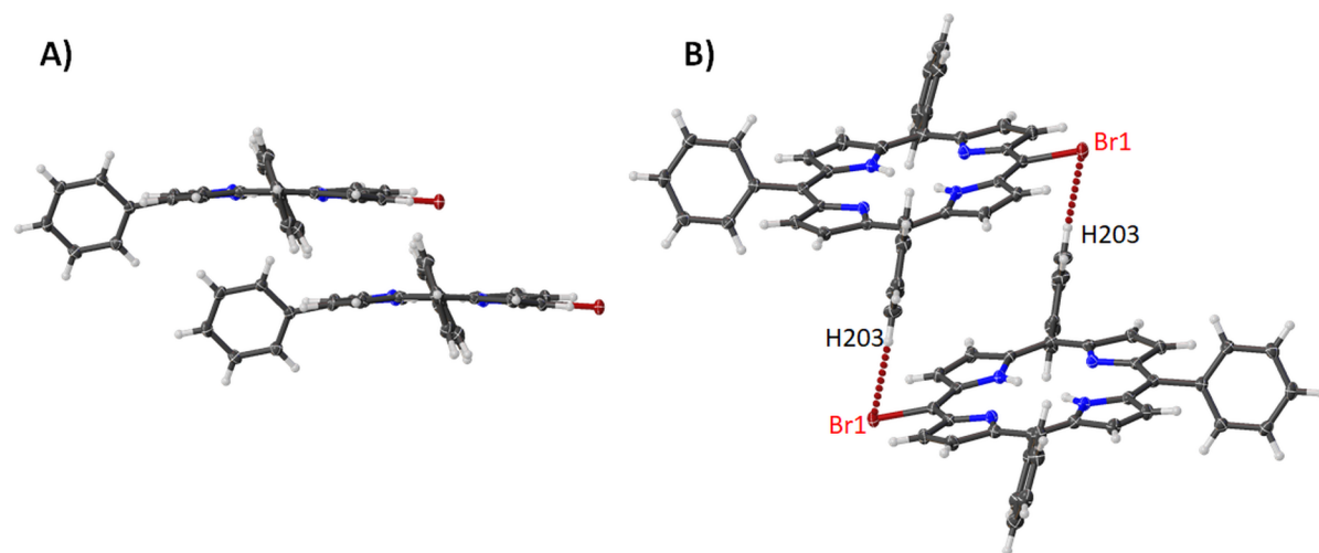
Figure 11: Expanded view (thermal ellipsoid plot) of compound 5 showing (A) porphyrin stacking and (B) Br...H interactions.
