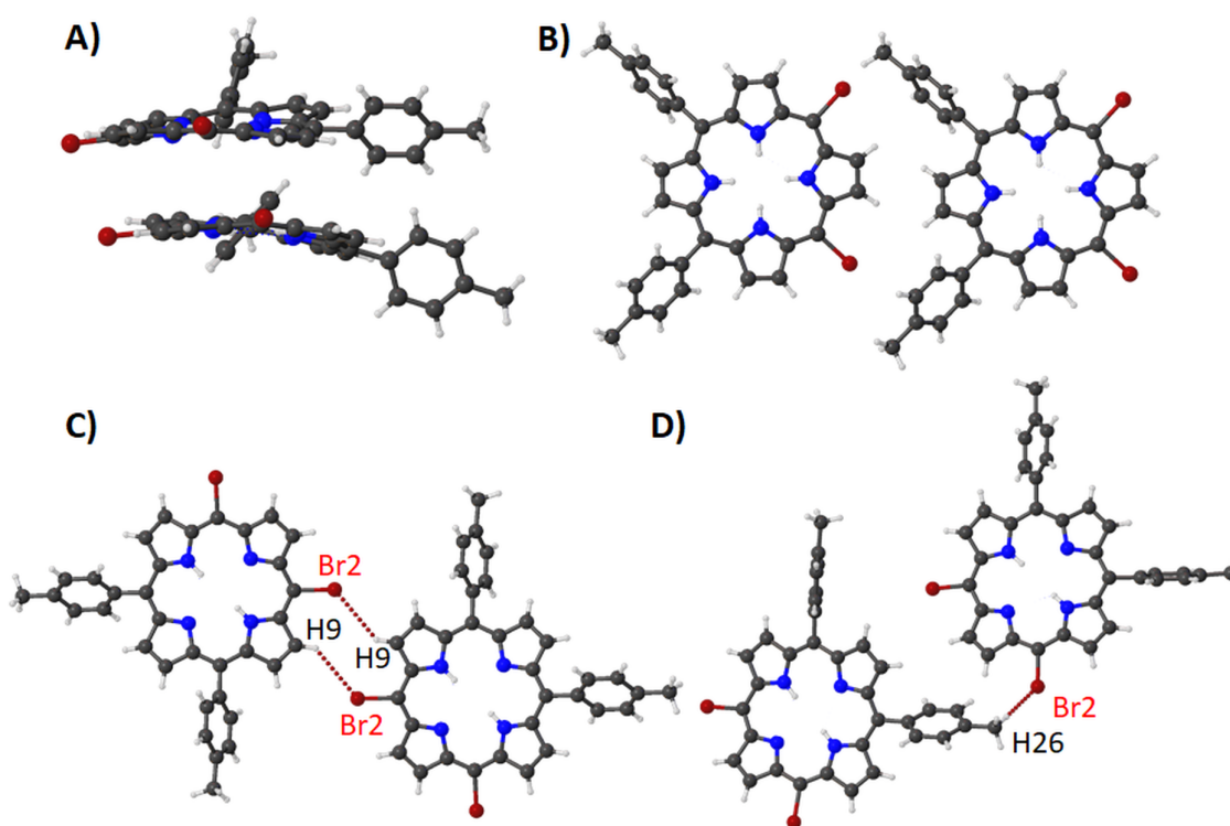
Figure 20: Expanded view (ball and stick) of compound 16 showing (A) stacking, (B) head-to-tail alignment, (C) Br...H interactions with pyrroles and (D) Br...H interactions with tolyl moiety.
