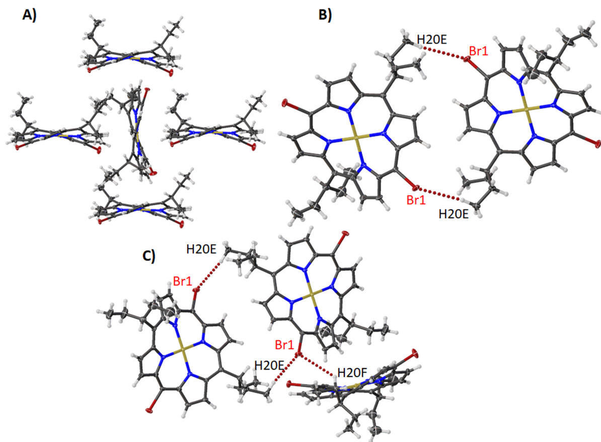
Figure 16: Expanded view (thermal ellipsoid plot) of compound 11 showing the (A) edge-on interactions, (B) edge-on Br \cdots H interactions and (C) Br \cdots Br contact.
