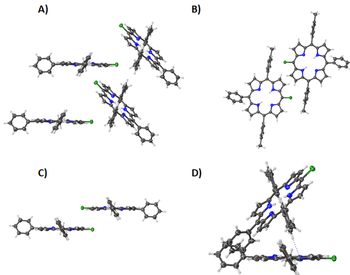
Figure 10: Expanded view (thermal ellipsoid plot) of compound 4 showing (A) tilted alignment of porphyrin rings, (B) chlorine atoms pointing towards the tolyl groups, (C) chlorine overlap and (D) phenyl overlap.
