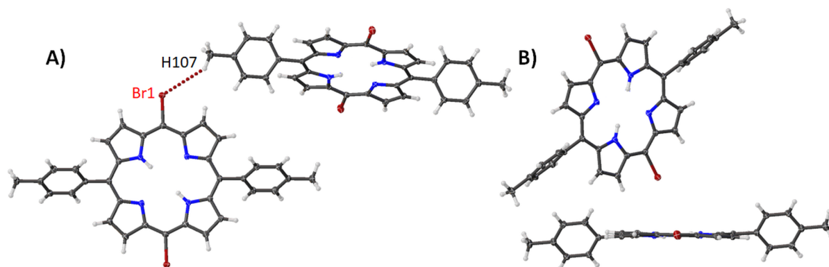
Figure 15: Expanded view (thermal ellipsoid plot) of compound 10 showing the (A) Br \cdots H interactions with tolyl moiety and (B) edge-on interaction between the porphyrin macrocycles.
