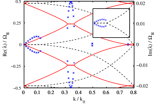
FIG. 1 (color online). Quasienergy spectrum of an oscillating polariton condensate. Lines (left axis) correspond to the real part of the quasienergy \lambda , and blue crosses to the nonzero imaginary parts (right axis). Modes with nonzero \text{Im}\lambda are unstable. The line colors indicate modes deriving from the phase mode or lower polariton (red solid) or the amplitude mode or upper polariton (black dashed). Inset: Spectrum of a weakly interacting Bose-Einstein condensate with attractive interactions, qualitatively reproducing the small-wave-vector behavior. The parameters are \omega_0 = -E = 0.4\Omega_R , \Delta(0) \approx 0.71 , and \phi(0) \approx 0.44 , implying a renormalized oscillation frequency \Omega \approx 0.48\Omega_R .
