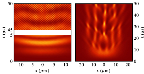
FIG. 2 (color online). Photon density from numerical simulations of Eq. (5), with resonant pumping of both upper and lower polaritons (left panel) and the upper polariton alone (right panel). The left panel shows the formation of a short-wavelength density modulation due to the wave-mixing instability, and the right the result of the attractive-gas instability. The pump field profile is a Gaussian at x = 0 with \sigma = 10 \mu\text{m} ; \Omega_R = 20 \text{ meV} ; E - \omega_0 = 4 \text{ meV} .
