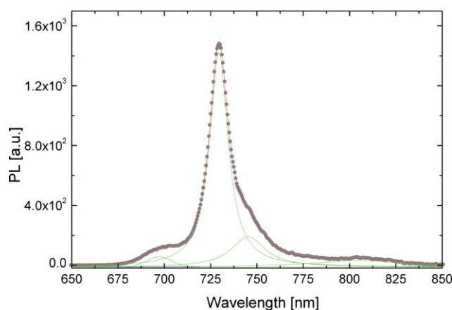
Fig. 2 Multiplex fitting of emission spectrum of an air saturated 100 mM phosphate buffer solution (pH = 7.4) of 45 \mu\text{M} [\text{Cr}(\text{phen})_2(\text{F}_2\text{dppz})](\text{CF}_3\text{SO}_3)_3 ( \lambda_{\text{exc}} = 308 \text{ nm} ). The lineshape and resulting fitting parameters are collected in Table S2 (ESI†).
