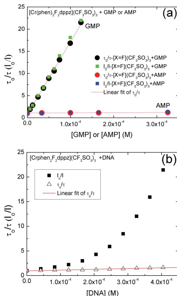
Fig. 5 Steady state and lifetime Stern–Volmer plots for emission quenching (at 730 nm) of an air saturated 100 mM phosphate buffer ( \text{pH} = 7.4 ) solution of [\text{Cr}(\text{phen})_2(\text{F}_2\text{dppz})](\text{CF}_3\text{SO}_3)_3 in the presence of increasing concentration of (a) GMP, [\text{Cr}] = 45 \mu\text{M} ; AMP, [\text{Cr}] = 36 \mu\text{M} and (b) CT-DNA, [\text{Cr}] = 80 \mu\text{M} ( \lambda_{\text{exc}} = 308 \text{ nm} ).
