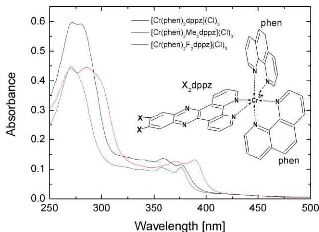
Fig. 1 Absorption spectra of 10 \mu\text{M} aqueous solutions of [\text{Cr}(\text{phen})_2(\text{X}_2\text{dppz})](\text{Cl})_3 {X = H, Me, or F}.
