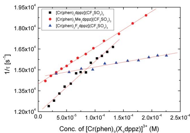
Fig. 3 Plot of 1/\tau as a function of [substrate] for an air-saturated aqueous solution of [Cr(phen) 2 (X 2 dppz)](CF 3 SO 3 ) 3 {X = H, Me, or F} ( \lambda_{\text{exc}} = 308 nm).
