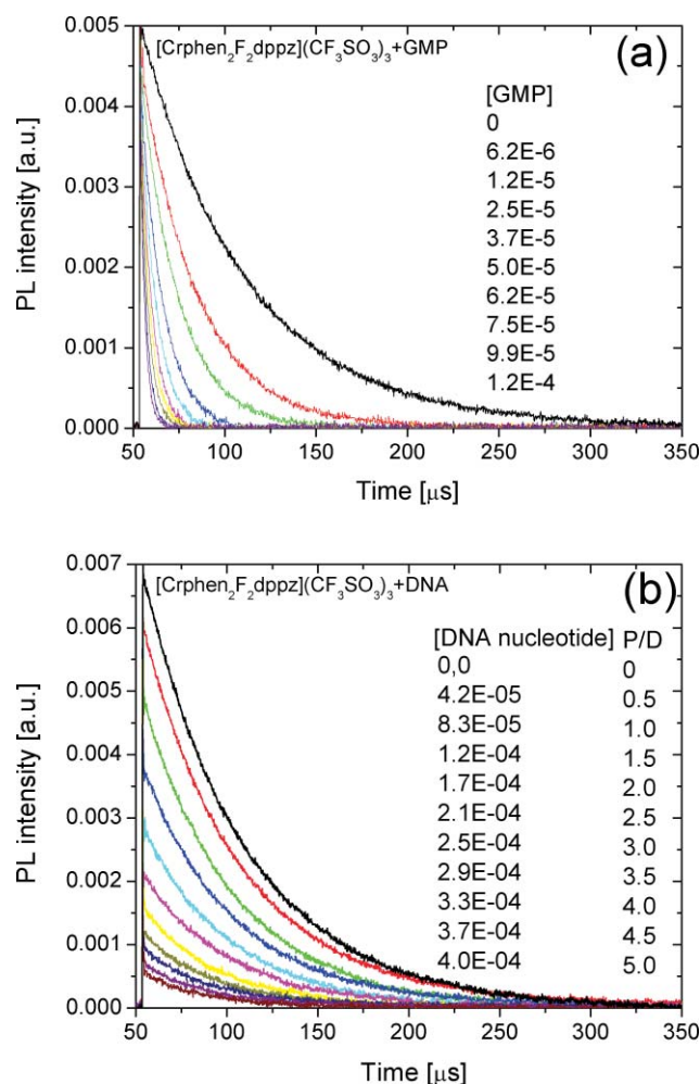
Fig. 4 Comparison of the phosphorescence lifetime quenching of an air saturated 100 mM phosphate buffer ( \text{pH} = 7.4 ) solution of [\text{Cr}(\text{phen})_2(\text{F}_2\text{dppz})](\text{CF}_3\text{SO}_3)_3 in the presence of increasing concentration of (a) GMP, [\text{Cr}] = 45 \mu\text{M} and (b) CT-DNA, [\text{Cr}] = 80 \mu\text{M} . P/D = nucleotide/Cr, \lambda_{\text{exc}} = 308 \text{ nm} .
