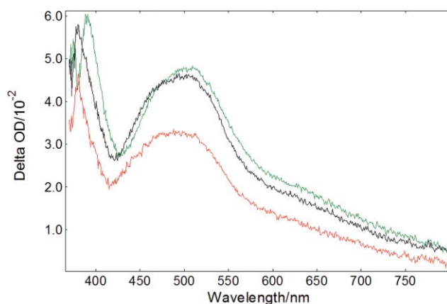
Fig. 6 Excited state absorption spectra recorded over the initial 3 \mu s (5 laser shots per spectrum) of 50 \mu M aerated aqueous solutions of [Cr(phen) 2 (X 2 dppz)](Cl) 3 , X = H (black), Me (green), or F (red).
