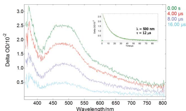
Fig. 7 Excited state absorption spectra of N_2 purged 10 mM phosphate buffer solution of 50 \mu\text{M} [\text{Cr}(\text{phen})_2(\text{dppz})](\text{Cl})_3 in the presence of 14 \mu\text{M} GMP recorded at 0, 4, 8 and 16 \mu\text{s} using an ICCD camera (gate width 4 \mu\text{s} , 5 laser shots per spectrum). Inset: Monoexponential fit (red line) of transient absorption band decay (green line) at 500 nm.
