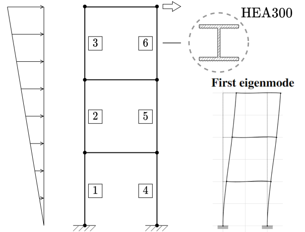
Figure 6: Three-storey plane frame
