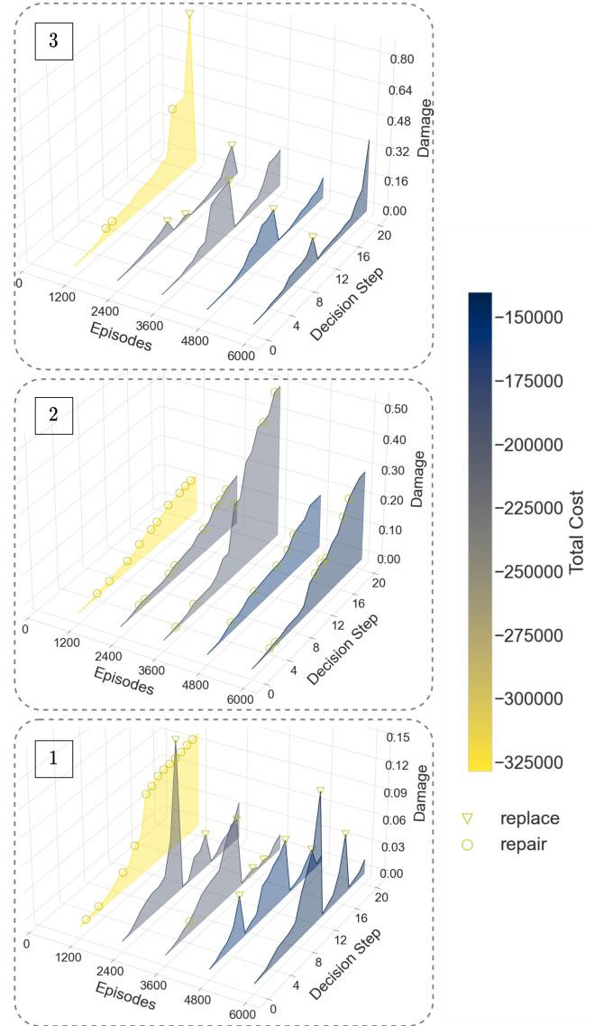
Figure 8: Policy realizations for all components for different training episodes
