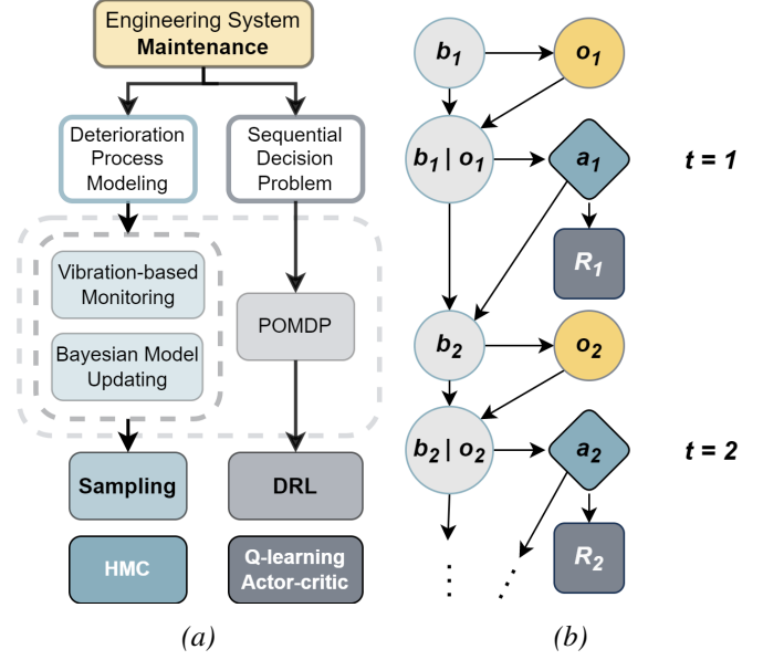
Figure 1: (a) Problem conceptual breakdown and (b) probabilistic POMDP decision graph.
