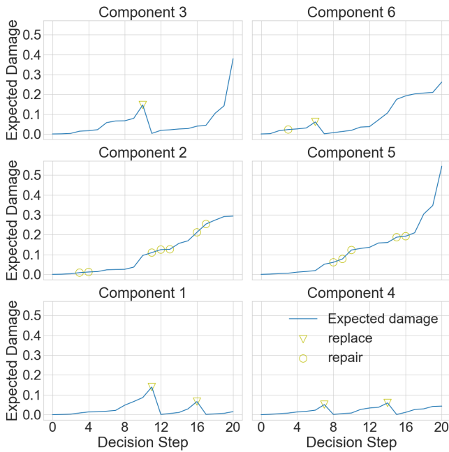
Figure 7: Policy realization for all components
