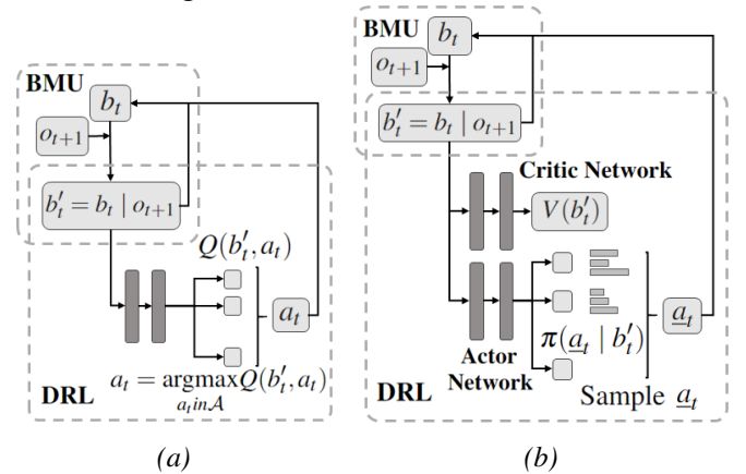
Figure 2: Neural network architectures for a single- and multi-component system (a) Q-function approximation for discrete action space (b) Actor-critic for centralized states and centralized discrete actions
