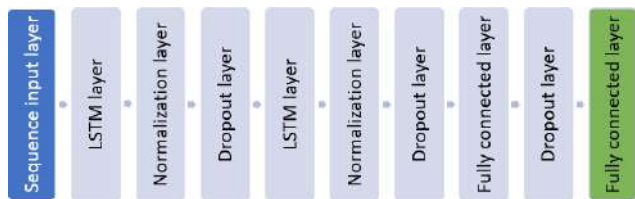
Figure 16. LSTM model architecture for predicting blade response.
