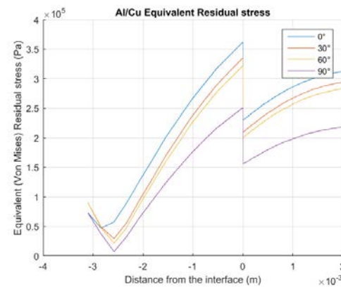
Figure 6: Through-thickness equivalent residual stress profiles for Al layers deposited on Cu substrate.
