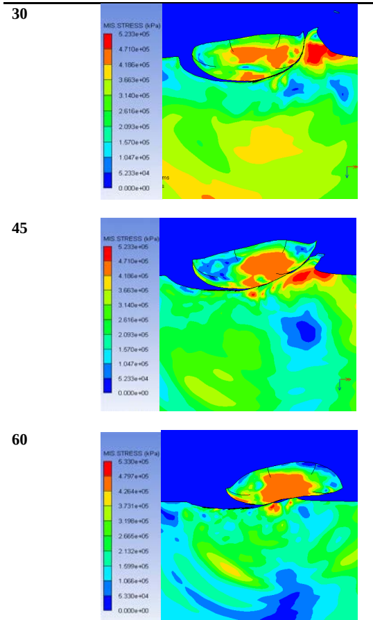
Figure 3: The simulation results for Von Mises stress in a single splat of Cu onto Al at 25°C, with friction coefficient of 0.3, particle velocity of 500 m/s and angle of impact: (a) 0°, (b) 15°, (c) 30°, (d) 45°, and (e) 60°.
