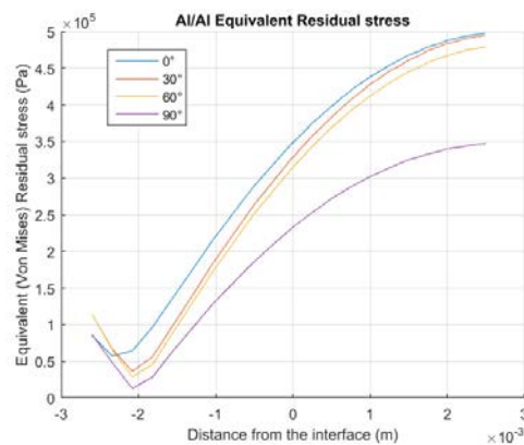
Figure 5: Through-thickness equivalent residual stress profiles for Al layers deposited on Al substrate.
