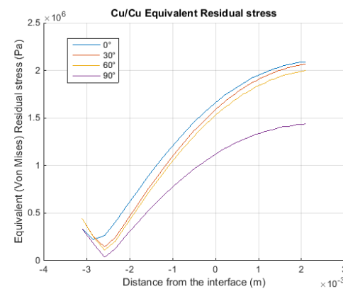
Figure 8: Through-thickness equivalent residual stress profiles for Cu layers deposited on Cu substrate.
