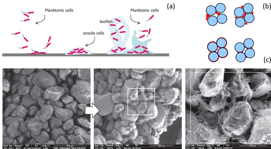
Fig. 15 a Bacterial life cycle and biofilm formation [95]; b possible forms of bacterial growth on soil particle surface [105—with permission from ASCE]; c clean Ottawa sand ( D_{50} = 120\mu\text{m} ) packed to a
