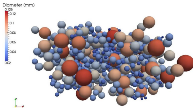
Fig. 3 Simulation of uniaxial compression of highly porous particulate matters through importing the “diffusion-limited aggregation” algorithm into 3D DEM software package PFC3D [11]
