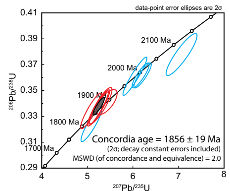
Figure 4. U-Pb concordia diagram for shocked zircon 13GGK029-Z25. Red ellipses represent analyses on neoblasts, and blue ellipses represent analyses on non-neoblastic, variably age-reset areas of host grain (see Fig. 2). Black ellipse is the weighted-mean-error ellipse calculated for the neoblast data shown in red. MSWD—mean square of weighted deviates.
