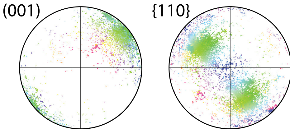
Figure 3. Pole figures showing crystallographic orientation data for shocked zircon 13GGK029-Z25. Each data point is colored using same inverse pole figure scale as used in Figure 2G; therefore the host grain, which is predominantly green in Figure 2G, is represented by cloud of green poles, and individual neoblasts, which have various colors in Figure 2G, are represented by myriad groups of poles scattered around this. There is no evidence for clustering of neoblasts into multiple orientations with distinct disorientation relationships. Plotted with equal area projection, showing only points in negative hemisphere.
