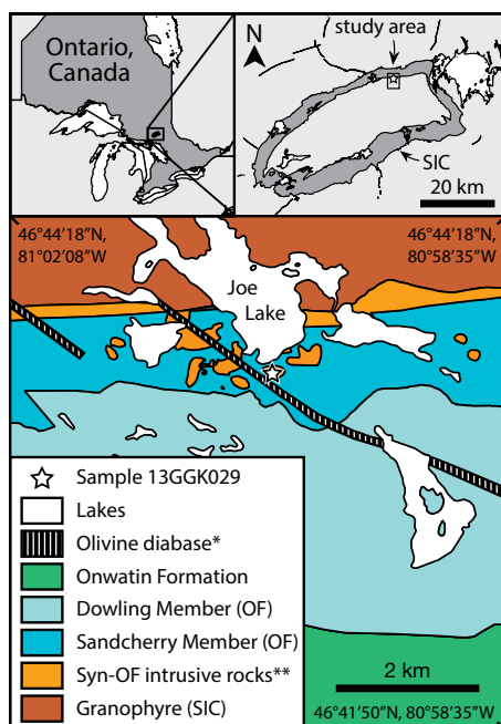
Figure 1. Map showing location of sample 13GGK029 at Sudbury impact crater (Ontario, Canada). Maps are modified after Ames et al. (2005). SIC—Sudbury Igneous Complex; OF—Onaping Formation. *—olivine diabase dikes belong to post-impact, ca. 1250 Ma Sudbury dike swarm. **—"syn-OF intrusive rocks" terminology of Ames et al. (2005); these include units previously mapped as "melt bodies" and Onaping intrusion, basal part of which has recently been reinterpreted as belong to SIC (see text, and Anders et al., 2015).
