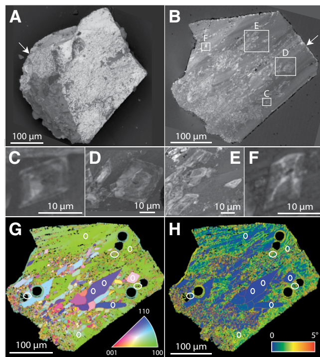
Figure 2. Imaging and electron backscatter diffraction analysis of granular shocked zircon 13GGK029-Z25 from Sudbury impact crater (Ontario, Canada). A: Backscattered electron image of grain exterior. Arrow points to surface on which polycrystalline nature of grain is readily visible. B: Cathodoluminescence (CL) image of polished grain interior. Arrow highlights CL-visible banding which may be original to grain prior to shock metamorphism. White boxes highlight areas shown in C–F. C, D: CL images of neoblasts appearing to show concentric internal structure. E: CL image showing internally complex neoblasts. F: CL image of neoblast appearing to show internal sector zoning. G: Map of zircon colored according to inverse pole figure scale, with all grain boundaries with misorientation >5^\circ shown in red. H: Map of zircon showing degree of local misorientation (kernel average misorientation; see full analytical methods for details) with grain boundaries shown in red. White ellipses in G and H show locations of secondary-ion mass spectrometry U-Pb analyses. Black circular features in G and H represent laser ablation pits for rare earth element analyses not reported here.
