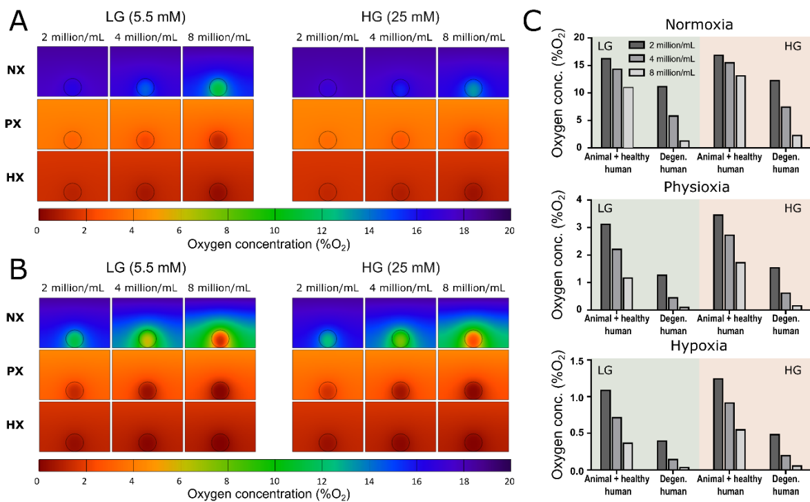
Figure 3. Investigating the effect of three different seeding densities on the oxygen concentration in a single 30µl alginate bead in 2 mL of low glucose (LG) or high glucose (HG) media (24-well) at normoxia (NX), physioxia (PX) and hypoxia (HX). (A) Oxygen contour plots for lower animal/healthy human metabolism. (B) Oxygen contour plots for a higher degenerated phenotype. (C) Minimum oxygen concentrations in the alginate bead at steady state for the different seeding densities, metabolic rates, and nutrient conditions.
