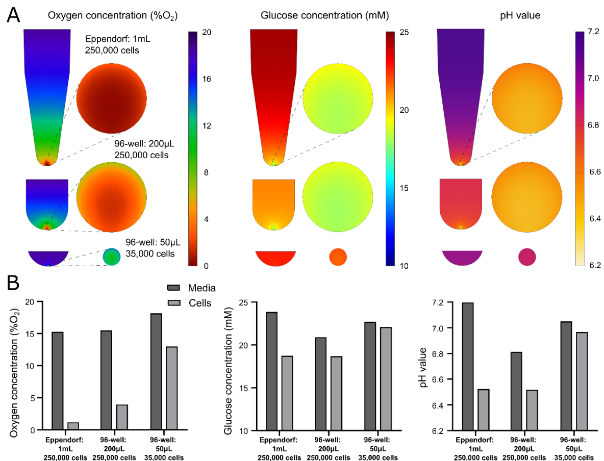
Figure 8. (A) Contour plots of oxygen, glucose and pH gradients through the culture media and cell aggregate of a 250,000-cell pellet in 1 mL (Eppendorf) or 200 \mu L (96-well) of media and a 35,000-cell microaggregate in 50 \mu L (96-well) of media. The presented values are predicted just prior to media refresh, under a twice weekly feeding regime. (B) Corresponding values for the average concentration of oxygen, glucose and pH in the media and the cell aggregate prior to a media exchange in each of the three culture configurations.
