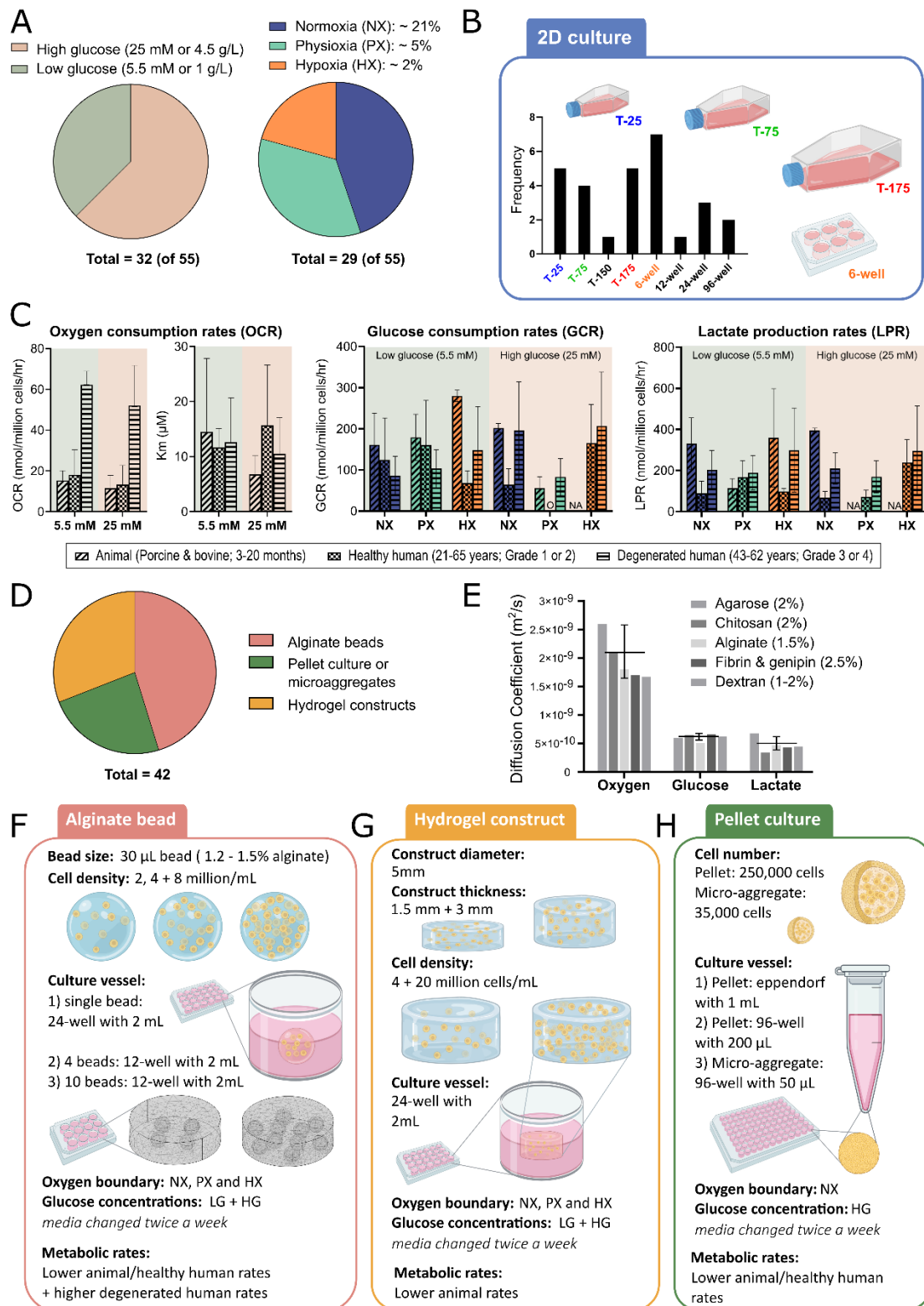
Figure 1. (A) The most used glucose concentrations and incubator oxygen levels across 55 reviewed studies. (B) The frequency of culture vessel used across these studies for 2D NP cell expansion and culture. (C) Compiled metabolic rates gathered from the literature and graphed according to glucose concentration and external oxygen concentration. (D) Most commonly used 3-D culture system for NP cells across 42 studies. (E) Effective diffusion coefficients for oxygen, glucose, and lactate through several relevant hydrogels at 37°C. (F-H) Most common configurations (geometrical dimensions, cell density, boundary concentrations and culture vessels) for alginate beads, cylindrical hydrogel constructs and pellet culture.
