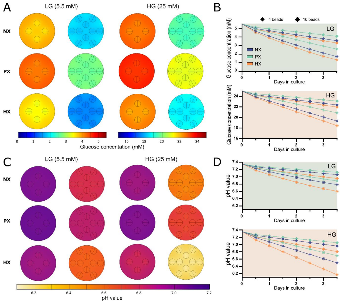
Figure 5. Investigating the effect of multiple alginate beads (4 or 10 beads of 4 million cells/mL) in a single culture vessel (12-well). (A) Contour plots showing the glucose concentration in a transverse plane through the centre of the bead in low glucose (LG) and high glucose (HG) media, just prior to a media exchange, at normoxia (NX), physioxia (PX) and hypoxia (HX). (B) Transient analysis of the minimum glucose concentration within an arbitrary bead within the 4 bead or 10 bead configurations up until the media exchange, for both LG and HG media. (C) Contour plots showing the pH in a transverse plane through the centre of the bead in LG and HG media, just prior to a media exchange, at NX, PX and HX. (D) Transient analysis of the minimum pH level within an arbitrary bead within the 4 bead or 10 bead configurations up until the media exchange, for both LG and HG media.
