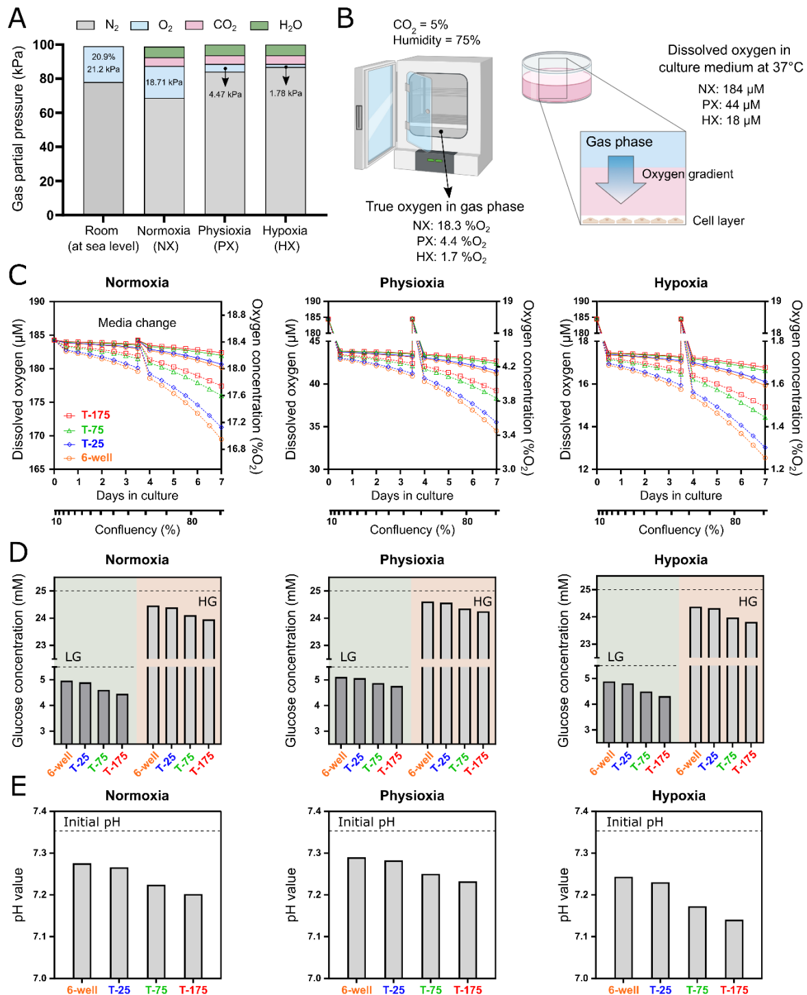
Figure 2. (A) The volume/volume ratio of oxygen to other gases in an incubator is decreased compared with that of dry air in a room. Values are shown for sea level. (B) As a result, the relative gas concentration in a normoxia (NX), physioxia (PX) or hypoxia (HX) incubator, with the addition of 5% CO 2 and 75% humidity, are lower than the conventional concentrations often cited. These incubator oxygen levels can then be converted to the concentration of dissolved oxygen by using an oxygen solubility coefficient in culture media at 37°C. (C) A temporal analysis of the oxygen concentration at the cell surface for cells proliferating over a 7-day period in either an NX, PX or HX incubator. Solid line indicates a lower animal/healthy human metabolism, dashed lines indicate a higher degenerated phenotype. (D) Glucose concentration of the media at 80% confluency for both low (5.5 mM) and high (25 mM) glucose media in a NX, PX and HX incubator. (E) pH concentration of the media at 80% confluency in a NX, PX and HX incubator.
