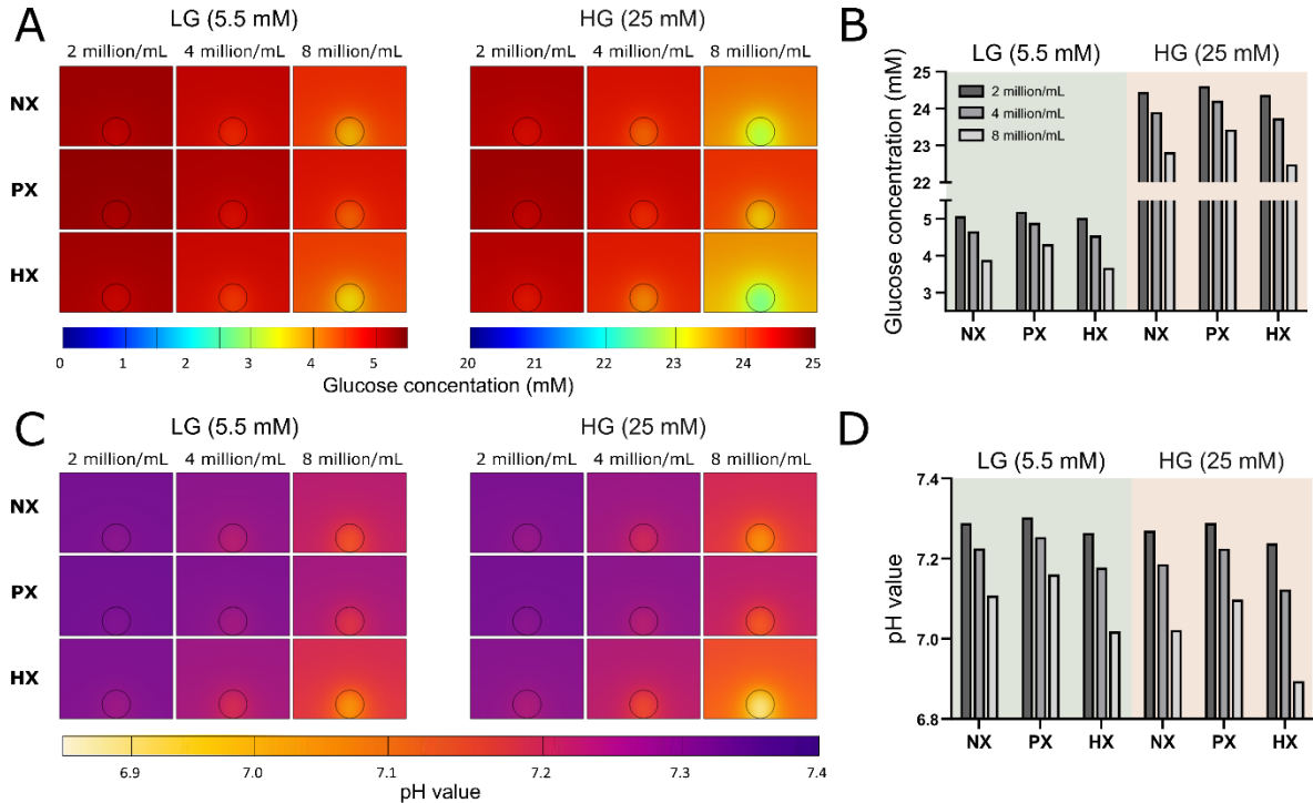
Figure 4. (A) Contour plots showing the glucose concentration in a single alginate bead of different seeding densities in low glucose (LG) and high glucose (HG) media, just prior to a media exchange, at normoxia (NX), physioxia (PX) and hypoxia (HX). (B) Corresponding minimum glucose concentrations within the alginate bead prior to media exchange. (C) Contour plots showing the pH level in a single alginate bead of different seeding densities in LG and HG media, just prior to a media exchange, at NX, PX and HX. (D) Corresponding minimum pH levels within the alginate bead prior to media exchange.
