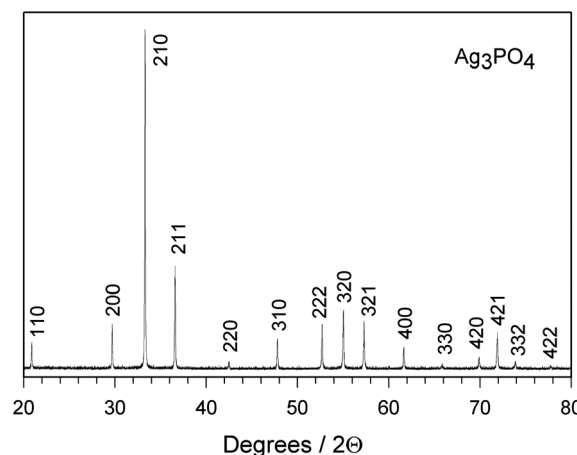
Fig. 1 An X-ray diffraction pattern of the \text{Ag}_3\text{PO}_4 powder after refluxing for 24 hours.
