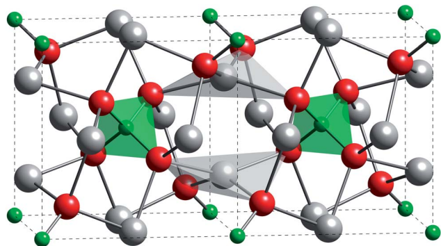
Fig. 2 The crystal structure of \text{Ag}_3\text{PO}_4 . The local coordination environments of P (tetrahedral) and Ag (distorted tetrahedral) are shown.
