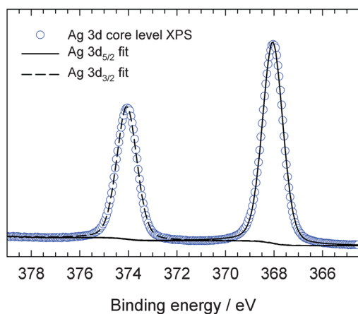
Fig. 3 The Ag 3d core level region of the photoelectron spectrum fitted using a single symmetric Gaussian–Lorentzian lineshape per peak.
