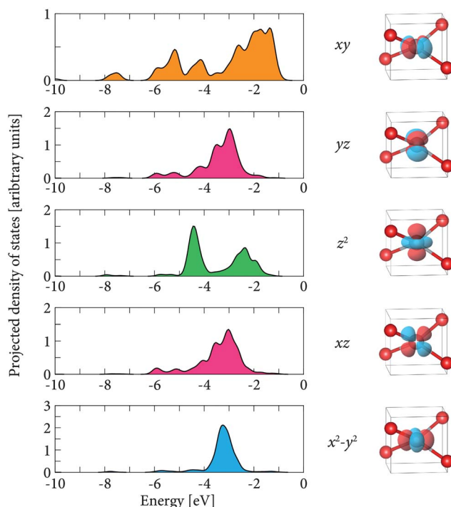
Fig. 8 Projected densities of states for the individual Ag 4d components.
