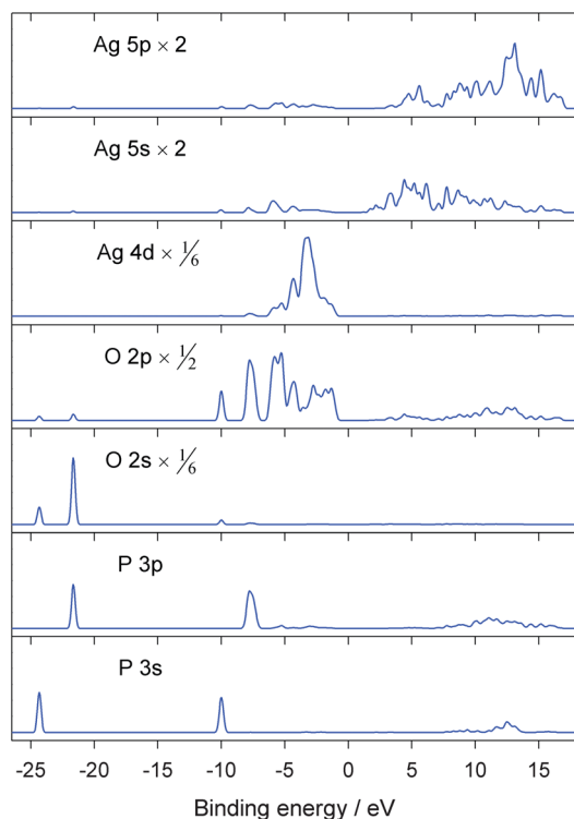
Fig. 7 Projected densities of states for the Ag 5p, 5s and 4d, O 2p and 2s, and P 3p and 3s orbitals.
