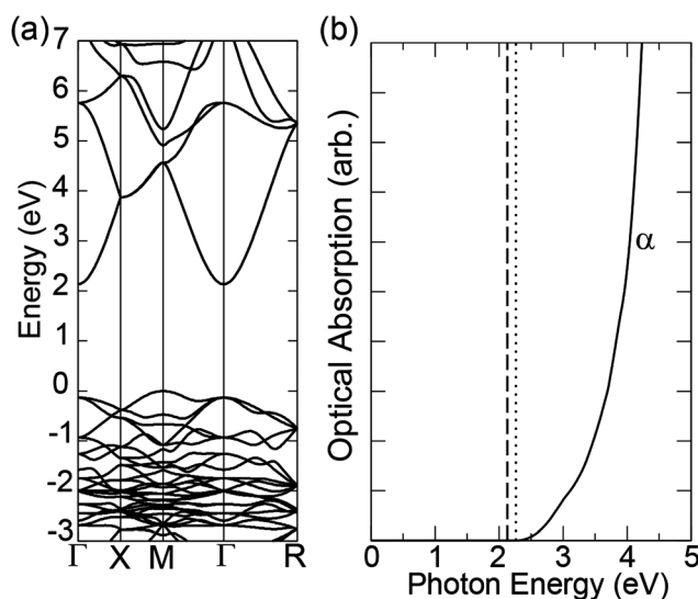
Fig. 5 (a) A band dispersion diagram for \text{Ag}_3\text{PO}_4 (b) The optical absorption edge of \text{Ag}_3\text{PO}_4 calculated using the transversal approximation and PAW method.
