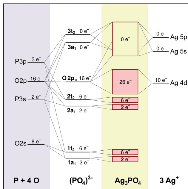
Fig. 6 A molecular orbital (MO) diagram of \text{Ag}_3\text{PO}_4 .
