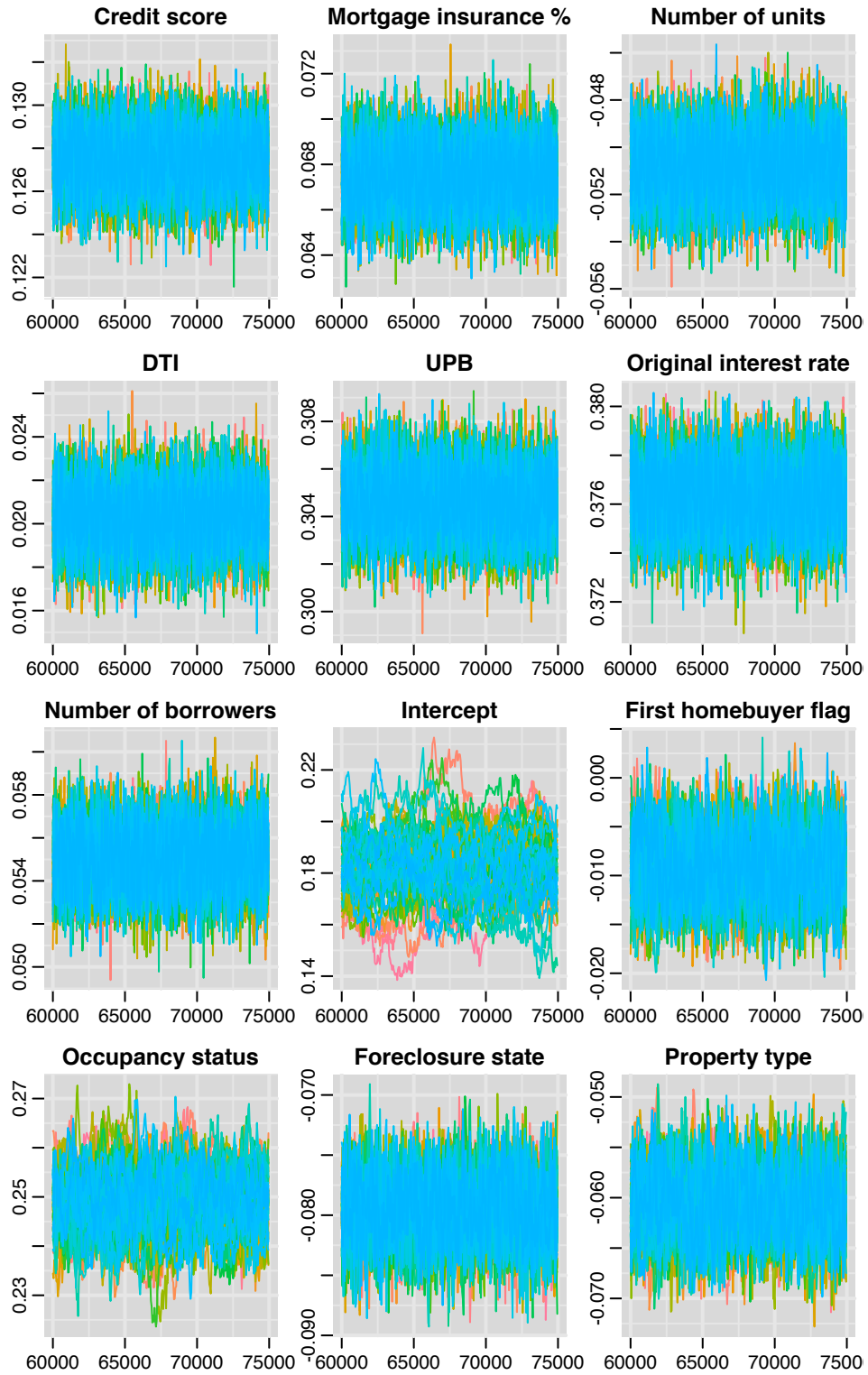
Figure .10: Trace plot of all parameters associated with covariates for prepaid category.
