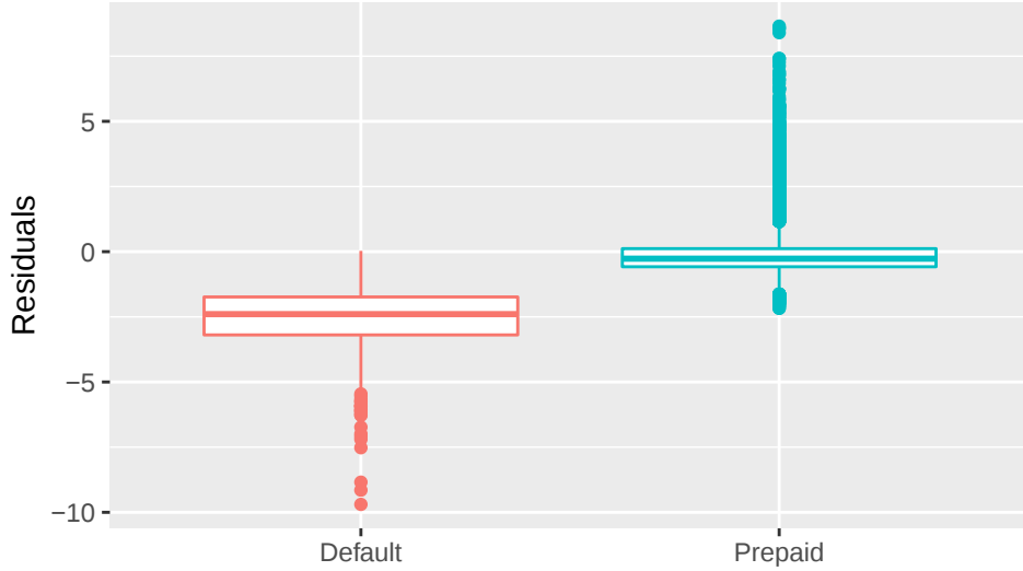
Figure 6: Separate box plots of residuals corresponding to default and prepay mortgages. The residuals for default mortgages show clear bias below 0.
