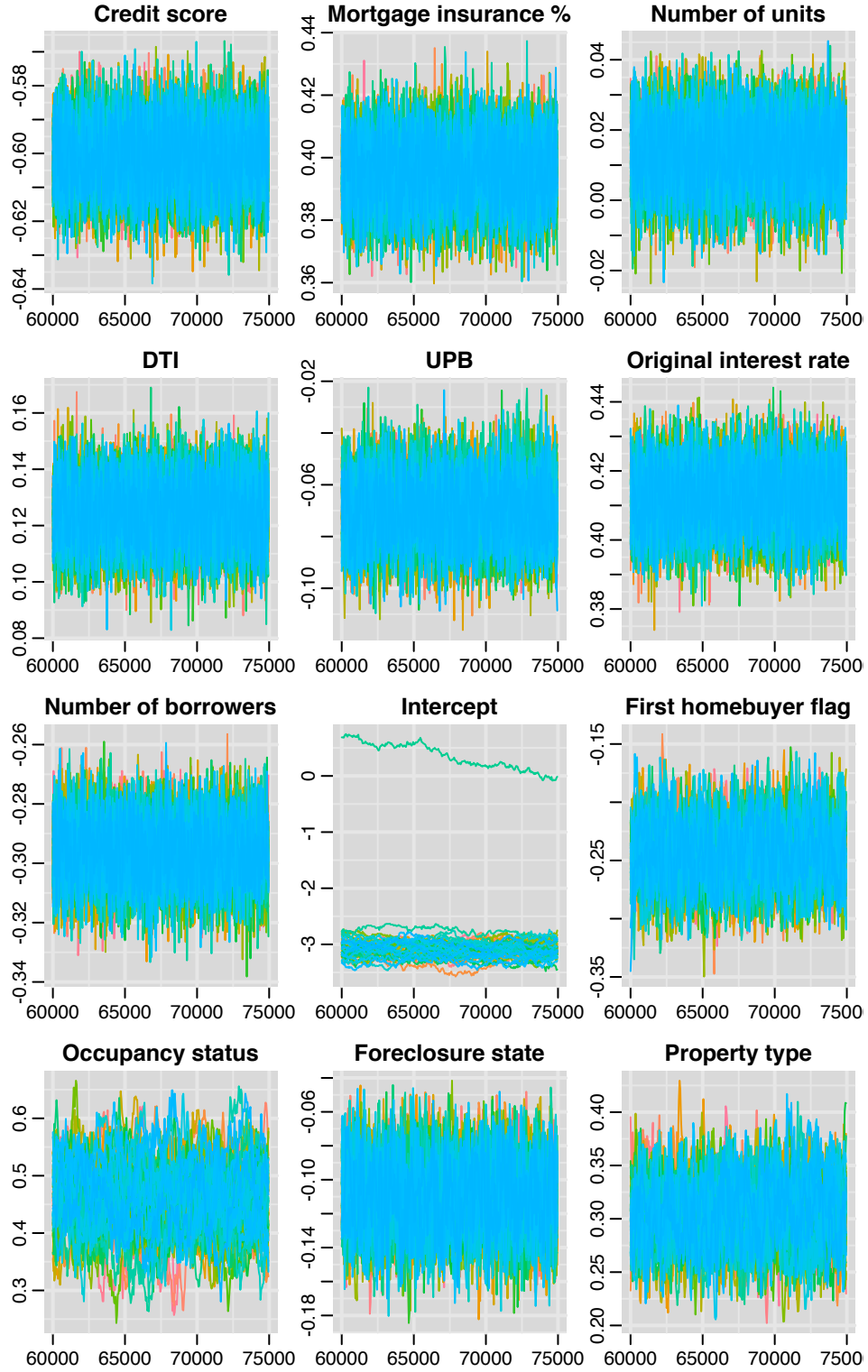
Figure .9: Trace plot of all parameters associated with covariates for default category. A single chain for intercept parameter is found to converge much more slowly than the others.
