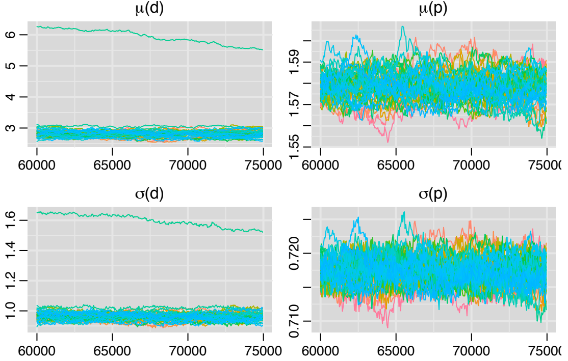
Figure .8: Trace plot of all distributional parameters. For parameters in default category, the single slow converging chain is visible here as well.
