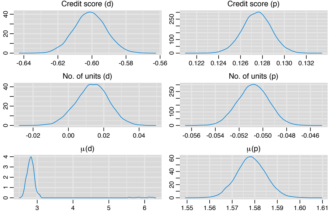
Figure 3: Density plot of combined samples from merging all the chains for credit score, number of units and \mu , both for default (d) and prepaid (p) times. The long tail corresponding to \mu(d) can be attributed to a single chain which is slow in converging.
