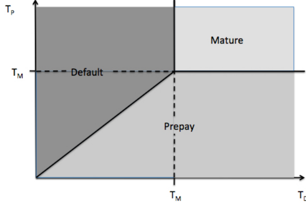
Figure 1: Competing risk representation of a mortgage that can default, prepay or mature at time T_M .
