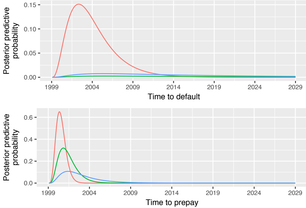
Figure 4: The two panels provide posterior predictive distributions of time to default and prepay respectively. The flat posterior predictive distribution of time to default is very common in almost all mortgages, while for prepay the shape of the distributions are quite varying. Note that some of the distributions are truncated at 2029, the year the mortgages end.
