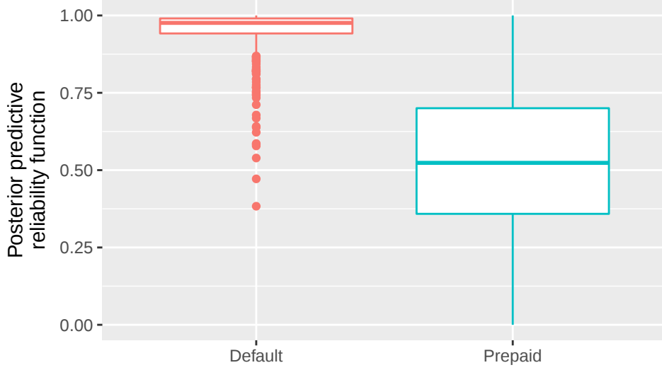
Figure 7: Box plots of posterior predictive reliability function computed for mortgages at time to default and prepay.
