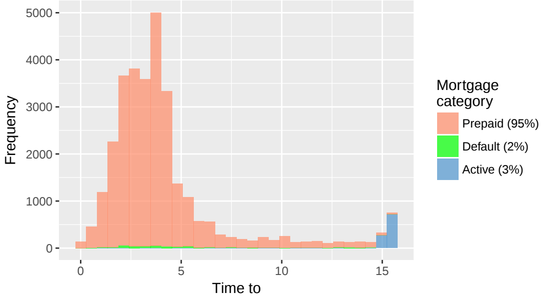
Figure 2: Histogram of time to default, prepaid and active times for each category.
