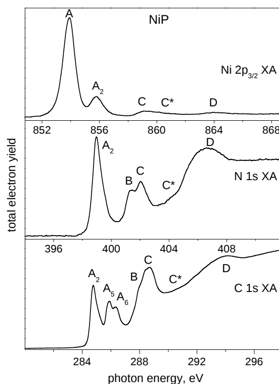
Figure 5. X-ray absorption spectra of NiP. The energy scales of the spectra are aligned using the measured differences between the core levels \Delta E(\text{Ni } 2p_{3/2} - \text{C } 1s) = 570.8 \text{ eV} and \Delta E(\text{N } 1s - \text{C } 1s) = 114.3 \text{ eV} .
