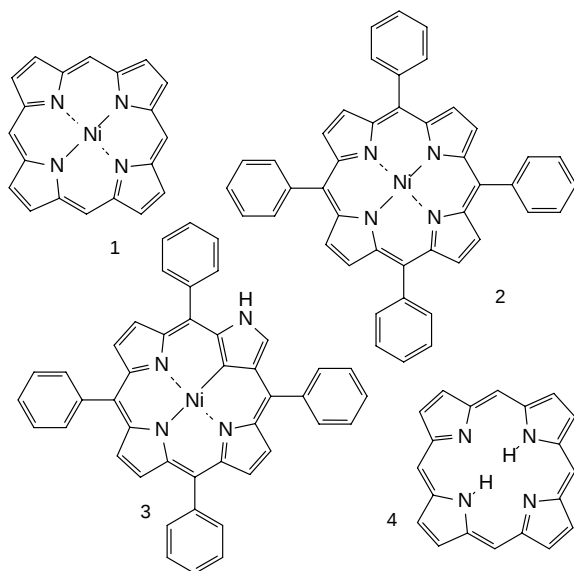
Figure 1. Structural formulas of the NiP (1), NiTPP (2), NiNCTPP (3) and H 2 P (4).
