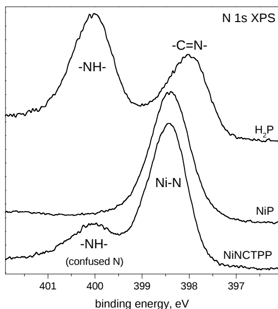
Figure 6. N 1s XPS spectra of the NiP, NiNCTPP and free-base porphine ( H_2P ).
