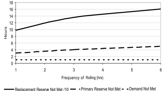
Fig. 8. Number of hours demand and reserve requirements not met over simulated year for different frequencies of rolling for stochastic mode. Note replacement reserve is divided by 10
