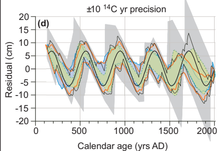
Simulation 4 - detrended curves - Confidence interval OxCal Bacon Clam Bchron
