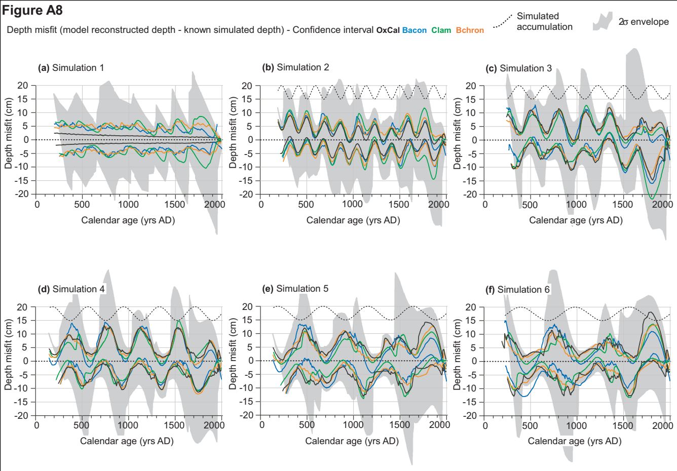
(a-f) Depth misfit (model reconstructed depth - known simulated depth, \pm 15 ^{14}\text{C} yr precision) for \pm 95\% confidence interval (CI) model results grouped to compare model success at constraining linear (a Simulation 1) and nonlinear (b-f Simulation 2 to 6) palaeommarsh surface (PMS) accumulation. NOTE - when any CI envelope crosses the zero line (black dashed) it has no longer successfully constrained the simulated age-depth sequence. Black line dashed line represents simulated accumulation; age-depth envelope (grey shade, Y-axis not scaled to fit these due to excessive space requirements) encompasses individually calibrated ^{14}\text{C} only, Bacon (blue lines, mean of 3 runs), Clam (green lines, 100,000 iterations using spline width 0.3), Bchron (orange lines, mean of 3 standard runs), OxCal (black lines, mean of 3 runs, P_Sequence K=2 auto, General outlier model). Bacon results are represented by the 95% probability intervals (PI) with step size of 10 cm for ^{14}\text{C} precision of 35 yrs ( \pm 1\sigma ), Clam by the 95% confidence intervals (CI), Bchron by the 95% highest posterior density region (HDR defined between 2.5% and 97.5%), OxCal by the 95% highest probability density range (HPD defined between from and to 95.4%).
