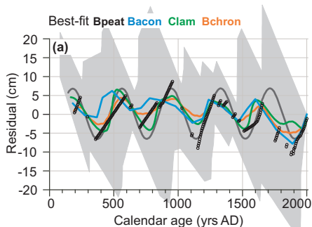
Simulation 4 - depth misfit (model reconstructed depth - known simulated depth)
