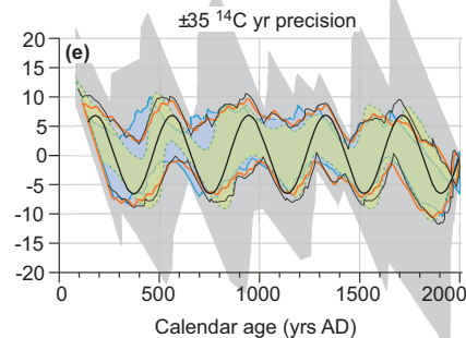
Simulation 4 - detrended curves - Confidence interval OxCal Bacon Clam Bchron
