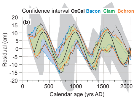
Simulation 6 - depth misfit (model reconstructed depth - known simulated depth)
