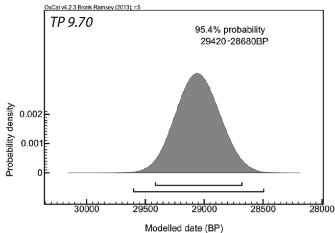
Fig. 8. Posterior probability density function generated for TP 9.70, the Tenaghi Philippon cryptotephra layer. The brackets at the base of the distribution represent the 95.4% and 99.7% probability ranges.
