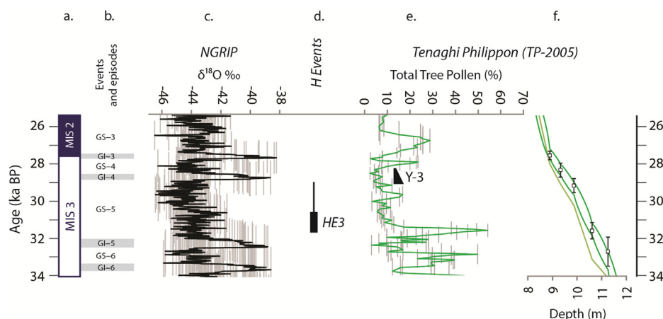
Fig. 9. Climatostratigraphic context of the Y-3 tephra at Tenaghi Philippon, NE Greece. Shown from left to right: (a) Marine Isotope Stage (Svensson et al., 2006, 2008); (b) The INTIMATE event stratigraphy (Lowe et al., 2008; Blockley et al., 2012). (c) The NGRIP oxygen isotope record based upon the GICC05 timescale from Andersen et al. (2006) and Svensson et al. (2006). (d) Calibrated age ranges for Heinrich Event 3 from western European records (Bard et al., 2000; de Abreu et al., 2003) (thin line) and calculated ages (Thouveny et al., 2000) (black box). (e) Tenaghi Philippon (TP-2005) total tree pollen percentage curve and the stratigraphic position of the Y-3 cryptotephra. (f) The age–depth model (at 95.4% probability range) and radiocarbon ages on which it is based are also shown (green) alongside the original Müller et al. (2011) chronology (grey green line). Note all data have been adjusted to a yrs BP (1950) timescale. (For interpretation of the references to colour in this figure legend, the reader is referred to the web version of this article.)
