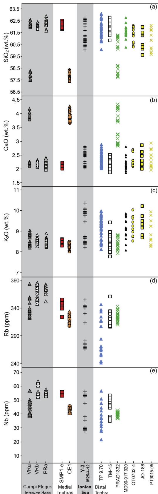
Fig. 5. Major and trace element compositional variation of glasses from the Y-3 tephra recorded in the Ionian Sea compared to potential proximal, medial and distal tephra correlatives. The Ionian Sea Y-3 glasses are dominated by two compositional end-members, whilst the Tenaghi Philippon tephra spans the full compositional range. Refer to Fig. 3 figure caption for published data references.
