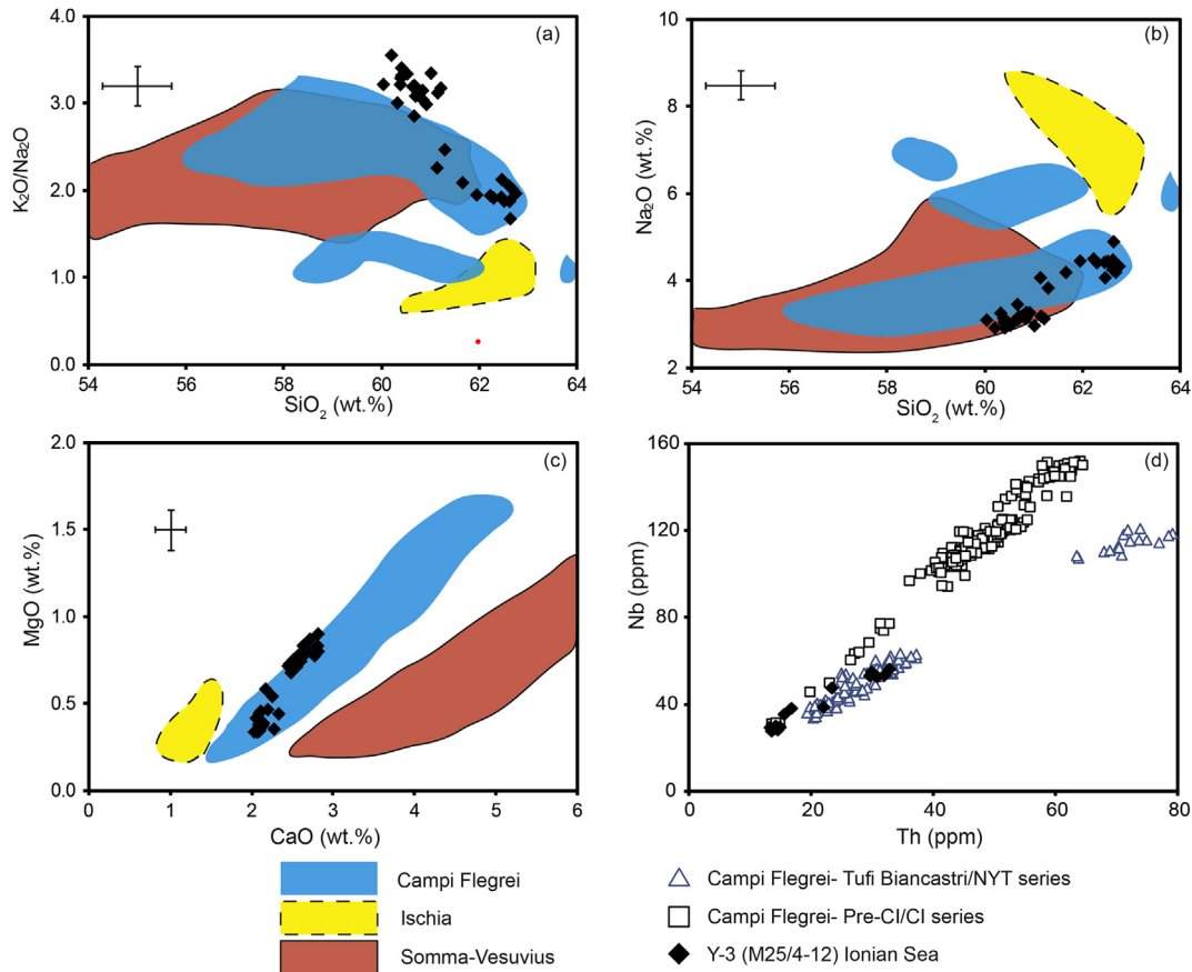
Fig. 4. Major and trace element glass compositions of the Ionian Sea Y-3 tephra (M25/4-12) compared to proximal Campi Flegrei (Tomlinson et al., 2012), Somma-Vesuvius (Tomlinson et al. unpublished 1 ) and Ischia (Tomlinson et al., submitted for publication) tephra deposits. (a–c) Y-3 glasses compared to the glass compositional fields of the Neapolitan volcanic centres; and (d) Y-3 glass compositions plotted against those of the pre- and post-Campanian Ignimbrite series (Tomlinson et al., 2012). Error bars represent 2 standard deviations of repeat analyses of the StHs6/80-G reference glass. 1 Vesuvius glass data used to evaluate potential geochemical links and to generate this compositional field is available on the RESET database ( https://c14.arch.ox.ac.uk/login/login.php?Location=/resetdb/db.php ).
