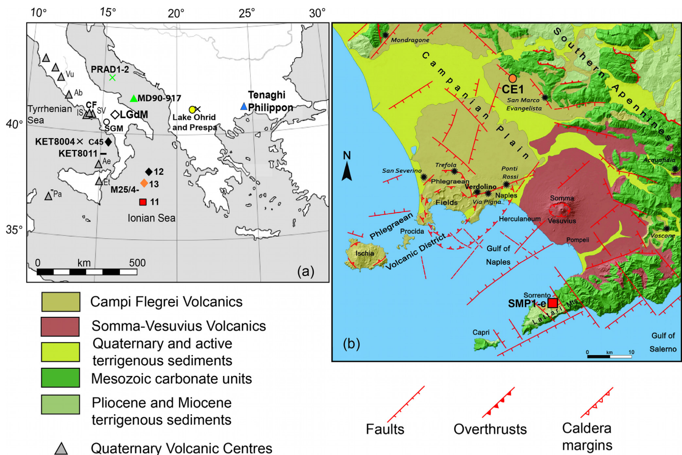
Fig. 1. (a) A map of the central and eastern Mediterranean showing the location of the M25/4-12 core from which the type locality Y-3 tephra was investigated. The localities of other archives where proposed 'Y-3' tephra correlatives have been reported (listed in Table 1). The main volcanic centres active during the Last Glacial (CF, Campi Flegrei; SV, Somma-Vesuvius; IS, Ischia, Ae, Aeolian Islands; Et, Mount Etna; Pa, Pantelleria) are marked. (b) The volcanoes in the Neapolitan volcanic region, Campi Flegrei, Somma-Vesuvius and Ischia (adapted from Tomlinson et al., 2012), and the localities of extra-caldera (SMP1-e and CE1) samples.
