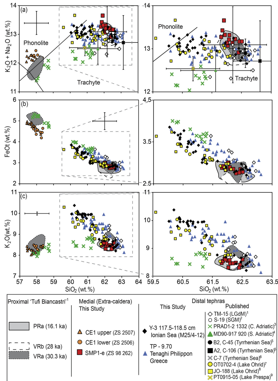
Fig. 3. Major element bi-plots showing the glass compositions of Ionian Sea Y-3 tephra (M25/4-12) compared to those of proximal intra-caldera Tufi Biancastri (Tomlinson et al., 2012) and extra-caldera deposits (SMP1-e, CE1; this Study) from Campi Flegrei. Glass data from cryptotephra TP 9.70 layer in Tenaghi Philippon, NE Greece (This study). Published glass compositions of distal layers (Table 1) are also presented to assess distal–distal tephra correlations: References are as follows; (1) Tomlinson et al. (2012); (2) Munno and Petrosino, 2007; (3) Bourne et al. (2010)*; (4) Zanchetta et al. (2008); (5) Munno and Petrosino (2004); (6) Paternò et al. (1988), Zanchetta et al. (2008); (7) Vogel et al. (2010); (8) Caron et al. (2010); (9) Damaschke et al. (2013). Error bars represent 2 standard deviations of repeat analyses of the StHs6/80-G MPI-DING reference glass. (a) TAS classification after Le Bas et al. (1986). *Water-free major element data for PRAD1332 (Bourne et al., 2010) was calculating assuming a 0.4 wt.% Cl prior to normalisation.
