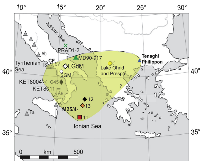
Fig. 7. The revised known dispersal and distribution of the Y-3 tephra.
