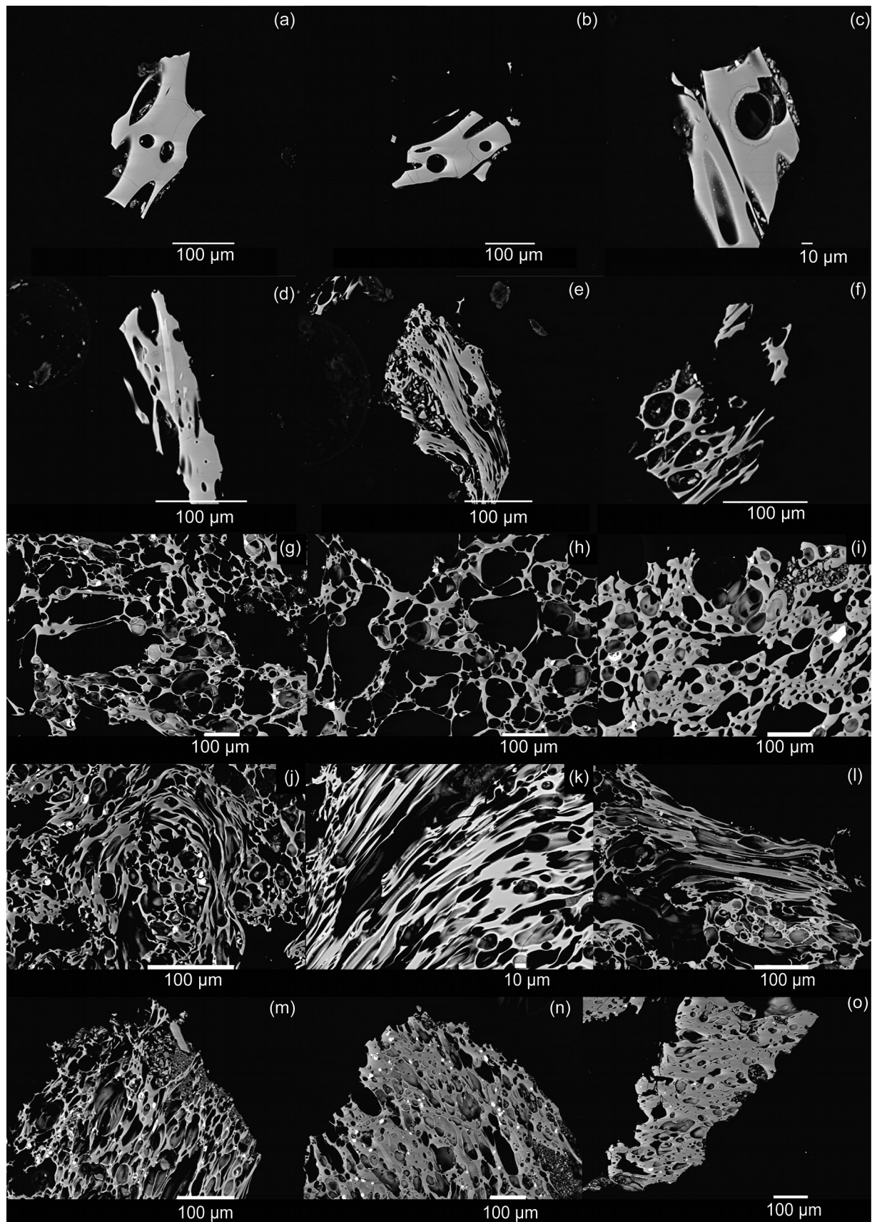
Fig. 2. SEM images of the distal and proximal tephtras. Y-3 tephra recovered from M25/4-12 in the Ionian Sea (a–f); (a) shard 40D, a 20 \mu\text{m} ablation pit is observed left of a vesicle; (b) shard 29C, with two laser ablation pits (34 and 20 \mu\text{m} diameter); (c) shard 50E showing a 34 \mu\text{m} ablation pit; (d) shard 32D, a thin microlite is observed running through the glass shard, which demonstrates the benefit of preliminary SEM investigations prior to LA-ICP-MS analysis; (e) shard 51E; (f) shard 42D showing two ablation pits (34 and 20 \mu\text{m} ); (g–h) the lower VRa, highly vesiculated white pumices (i) the upper VRa, less vesiculated, darker pumice; (j–l) SMP1-e (ZS 98262), highly vesicular and stretched pumices; (m) lower CE1 (ZS 2506) pumice, vesicular and stretched glasses; (n–o) upper CE1 (ZS 2507) pumices that are less vesiculated than the stratigraphically lower CE1 pumices.
