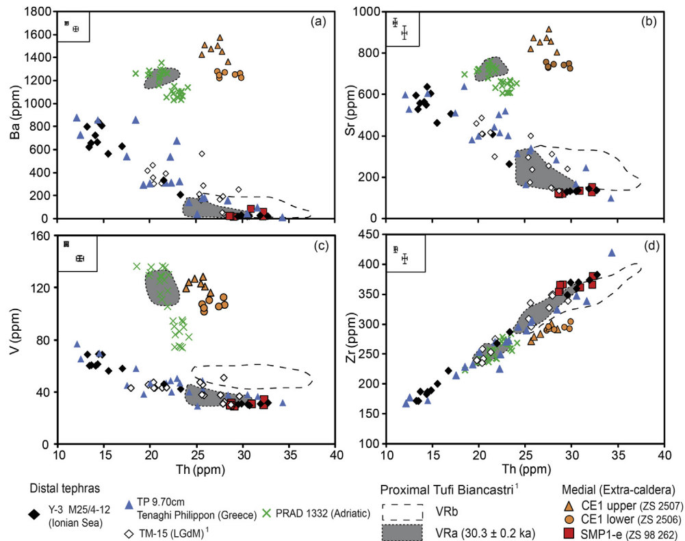
Fig. 6. Trace element glass compositions of the Ionian Sea Y-3 tephra (M25/4-12) compared to those of proximal intra-caldera Tufi Biancastri (Tomlinson et al., 2012) and extra-caldera deposits (SMP1-e, CE1; this study) from Campi Flegrei. The glass compositions of distal tephra layers TP 9.70, PRAD 1332 (this study), and LGdM TM-15 (Tomlinson et al., 2012). Error bars represent 2 standard deviations of repeat analyses of both the StHs6/-80G and ATHO-1G reference glasses.
