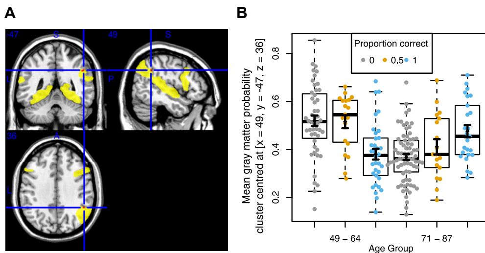
Fig. 1. A) Significant age group by accuracy (in 230 ms “Post” condition) interaction in the right AG (red) overlaid on the ROI mask (yellow) B) Mean gray matter probability for extracted cluster in each group. Boxplots illustrate interquartile range and median. Black diamonds with error bars indicate group means and standard errors. (For interpretation of the references to color in this figure legend, the reader is referred to the online version of this article.)
