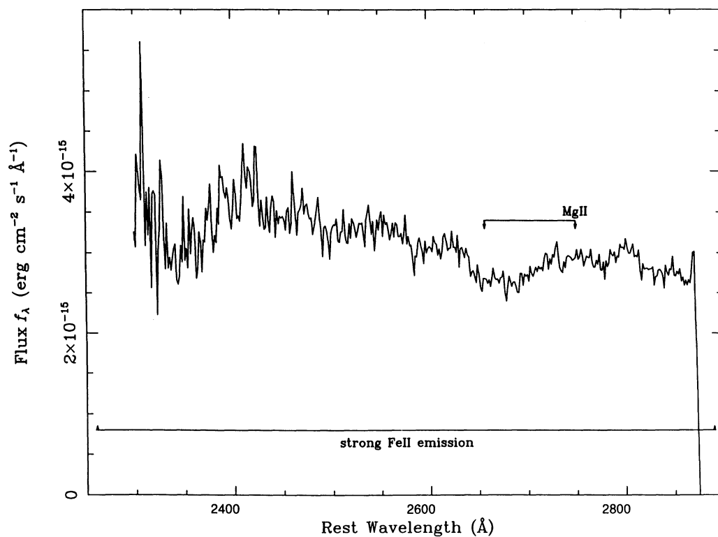
FIG. 2.—Rest frame spectrum of PG 0043+039 obtained with the KPNO RC spectrograph from 3250 to 4000 Å at a spectral resolution of \sim 130 km s -1 . The predicted position of a possible Mg II BAL (see Fig. 1) is labeled.
