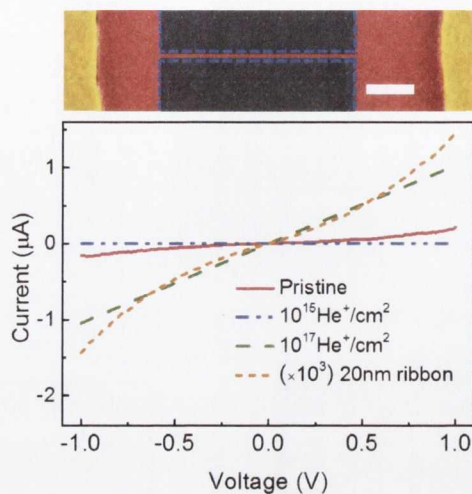
Figure 6.13: Electrical characterization of He + manufactured 20 nm nanoribbon.
