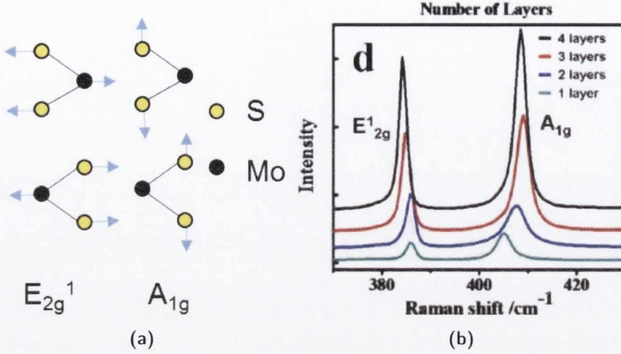
Figure 2.8: Vibrational modes and Raman spectroscopy for the differentiation of the number of MoS 2 layers thinned by plasma [12, 13]. (a) shows the vibrational modes giving rise to both peaks in the part of the Raman spectra shown in (b).
