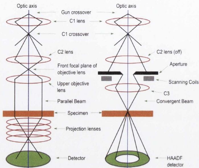
Figure 4.5: Outline of a transmission electron microscope (left) and a scanning transmission electron microscope (right) [184].
