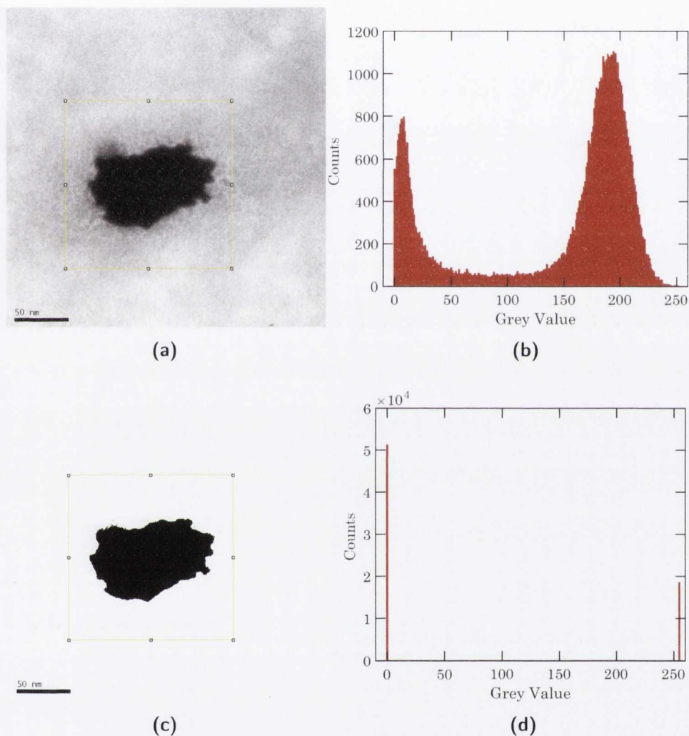
Figure B.4: Measuring nanopore sizes from TEM images with Imagej. (a) is a TEM image of a nanopore with a 150 nm \times 150 nm box drawn around it in Imagej. (b) is a bimodal histogram of gray values extracted from the yellow box. (c) is (a) after applying a threshold in Imagej. (d) is the histogram of (c). The ratio of dark and bright counts allows the calculation of etched area.
