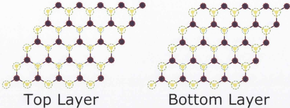
Figure 3.3: Displacement cross sections of atoms in \text{MoS}_2 with 30 keV \text{He}^+ . Mo atoms are shown in purple and S atoms are shown in yellow. The size of the circles shown in dotted lines represents the sputtering cross sections of the respective atoms.
