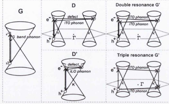
Figure 2.3: Double and triple resonance in Raman spectra of graphene. (Left) first-order G band process and (center) one-phonon second-order double-resonance process for the D band (intervalley process) (top) and for the D' band (intravalley process) (bottom). (Right) two-phonon second-order resonance Raman spectral processes (top) for the double-resonance G' process, and (bottom) for the triple resonance G' band process triple resonance (TR) for monolayer graphene [68]. For one-phonon, second-order transitions, one of the two scattering events is an elastic scattering event. Resonance points are shown as open circles near the K point (left) and the K' point (right) [63].
