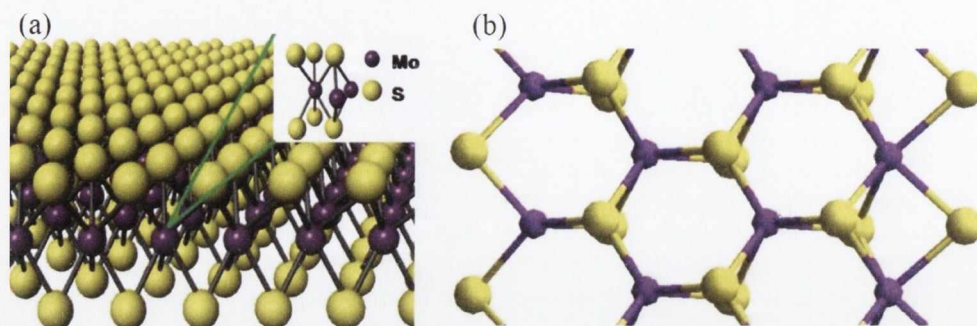
Figure 2.7: The crystal structure of monolayer \text{MoS}_2 . A schematic diagram of the atomic structure of monolayer \text{MoS}_2 [97]. Mo atoms are shown in purple and S atoms are shown in yellow.
