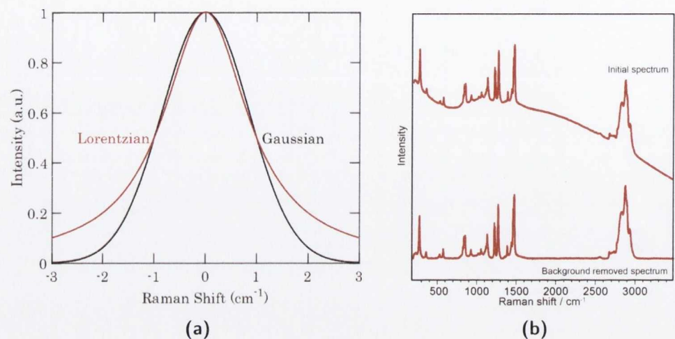
Figure 4.2: Data treatment in Raman spectroscopy. (a) shows both Lorentzian (red) and Gaussian (black) distributions with the same height, centre and FWHM. (b) shows a sample Raman spectrum as initially acquired and after the removal of the broad fluorescence background. The remaining spectrum is flat in the absence of local peaks and is easily analysed by fitting peaks to it [170].
