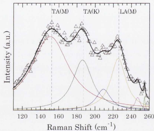
Figure D.1: Raman spectra of MoS 2 irradiated with 2.5 \times 10^{15} \text{ He}^+ \text{ cm}^{-2} . The range shown includes the LA(M) mode at \sim 226 \text{ cm}^{-1} which is highlighted with the dashed vertical line. This region was fitted with Lorentzians as shown in a range of colours, the sum of which is shown in the thicker black line.
