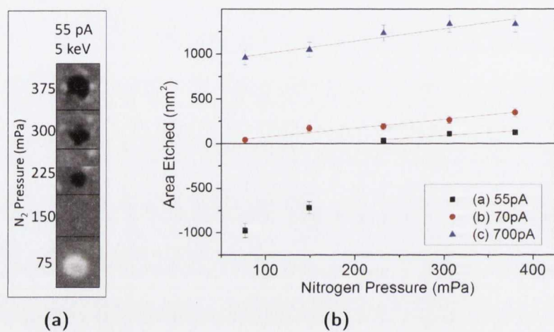
Figure 5.3: Etching and deposition rates as a function of beam current. (a) An example of the deposition and etching observed at 55 pA beam current is shown. (b) At the lowest beam current (55pA, black squares) hydrocarbon contamination was initially observed. Upon increasing the nitrogen gas pressure the deposition was observed to be suppressed and etching then began to dominate. The etching rate was observed to be increased at higher beam currents of 70 pA and 700 pA. In all cases the rate of etching grows with higher gas pressure.
