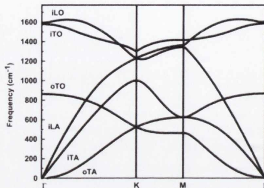
Figure 2.2: The calculated phonon dispersion relation of graphene [62, 63]. The iLO, iTO, oTO, iLA, iTA and oTA phonon branches are shown.
