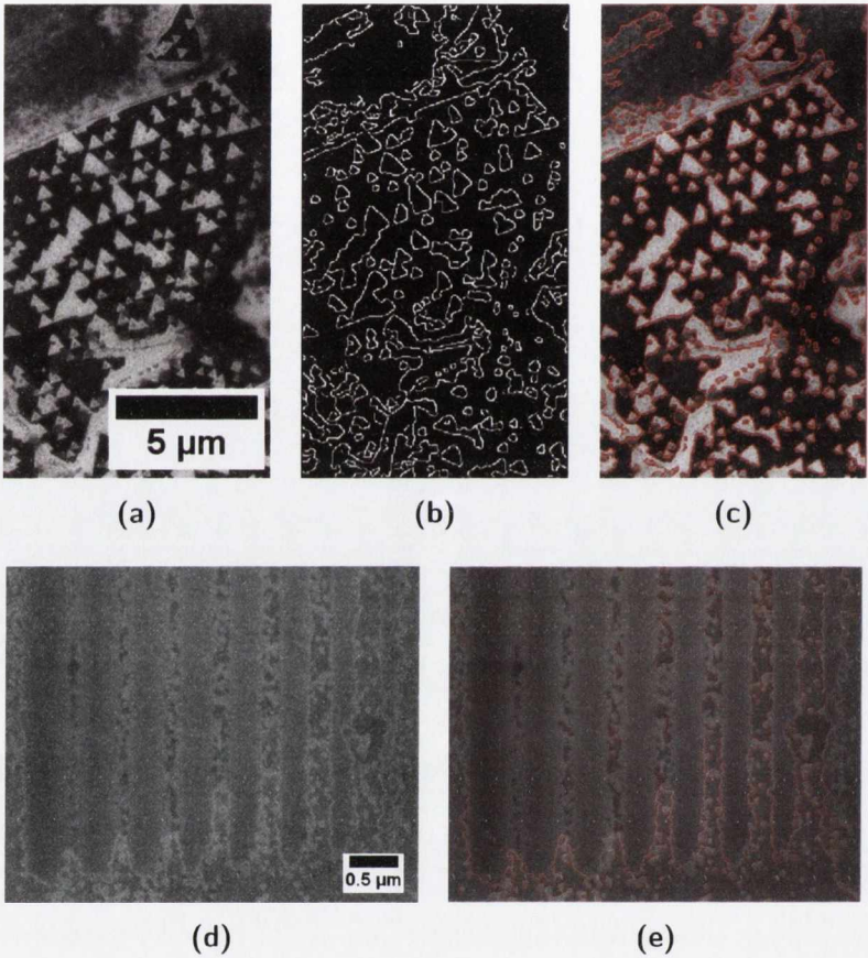
Figure G.1: Meshes of CVD-grown MoS 2 produced by oxidation. (a) SEM image (inLens, 10 keV) of MoS 2 etched at native defect sites. (b) The same image after passing through edge detection in matlab . (c) Overlay of the edge detection image (now in red) on the original image. (d) Another SEM image (inLens, 10 keV) of MoS 2 etched at ion-induced defect sites in an array of lines of progressively higher doses. (e) Same image repeated with edge detection.
