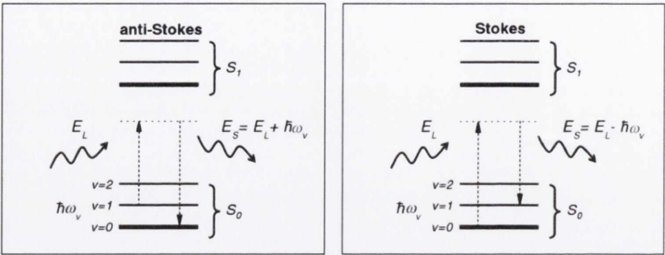
Figure 4.1: Jablonski diagram illustrating Stokes and anti-Stokes shifts [164].
