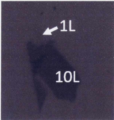
Figure B.2: Optical image of single and ten layer MoS 2 on a 300 nm SiO 2 layer on Si.
