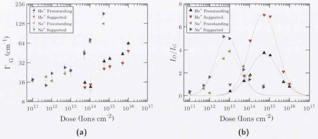
Figure 5.8: Evolution of full width at half maximum of the G peak and intensity ratio in graphene. (a) Evolution of FWHM of Lorentzian fits to the G peak, \Gamma_G , as a function of dose for He^+ and Ne^+ for both freestanding and supported graphene. (b) The evolution of the I_D/I_G ratio of graphene with irradiation dose. A Gaussian function has been fitted to each of the four data sets in this graph for illustrative purposes only.
