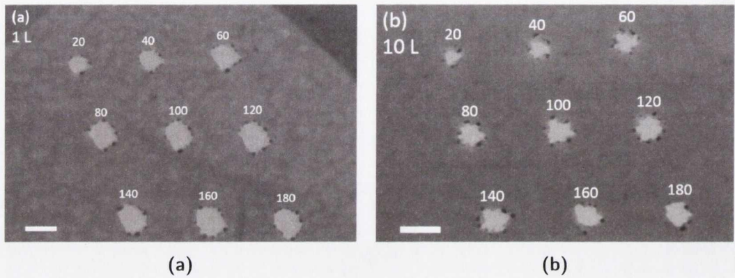
Figure B.1: (a) Monolayer graphene sample etched with nine different dwell times. (b) Ten layer graphene sample also etched with nine different dwell times. Scale bars are 100 nm.
