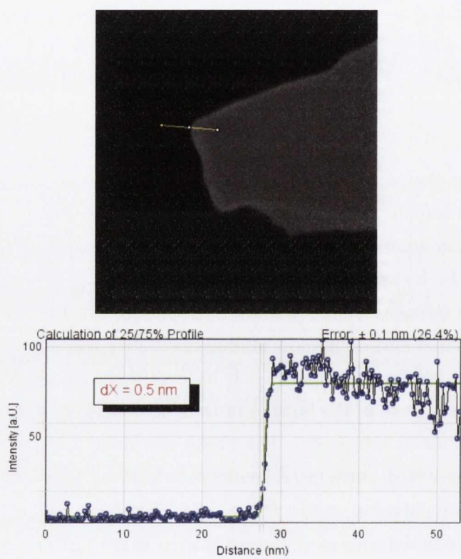
Figure E.1: Measuring probe size from a GIM image. Measuring probe size from a He^+ image in ImageJ . [190]
