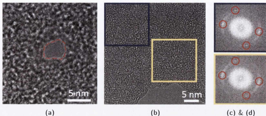
Figure 5.2: TEM images of electron beam-assisted nitrogen etched graphene. (a) TEM image of an etched pore with an average diameter of just 4.5 nm. (b) TEM image of the area beside an etched nanopore. (c) The FFT of the top left area in the blue box in (b). The spots showing the good crystal structure are circled. (d) The FFT of the bottom right area in the yellow box in (b). The spots were not observed in this image.
