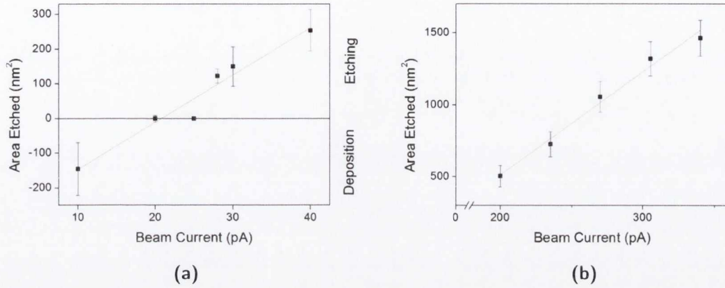
Figure 5.5: Nitrogen etching rate as a function of beam current (a) The transition from deposition to etching at higher beam current is observed. (b) A higher rate of etching occurs with increasing beam current.
