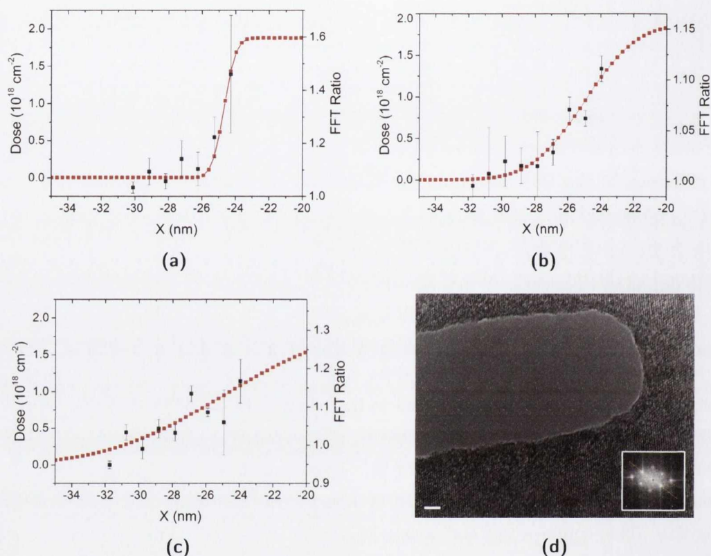
Figure 6.9: Graph of simulated ion distribution at Nanostructure edges with ratio of FFTs. The red data points show the extension of the \text{He}^+ dose from the simulation. The black data points represent the ratio of spots in local FFTs taken periodically from the milled edge out towards pristine material. (a), (b) and (c) correspond to \text{He}^+ probe sizes of 1.7, 6 and 12 nm respectively. (d) shows a feature milled with the 1.7 nm probe size with an inset of a local FFT acquired far from the edges of the feature. The FFT has a yellow line indicating the spots measured in imageJ where the values were extracted from. Uncertainties are the standard deviation of three measurements.
