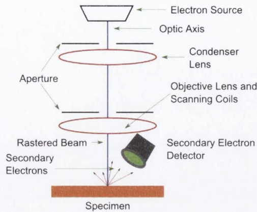
Figure 4.4: Outline of a scanning electron microscope
