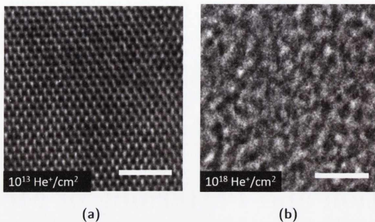
Figure 6.1: Modification of few layer mechanically exfoliated MoS 2 crystal structure with He^+ imaged in TEM. (a) and (b) show TEM images of irradiated MoS 2 with low ( 1 \times 10^{13} He^+ cm^{-2} ) and high ( 1 \times 10^{18} He^+ cm^{-2} ) doses respectively. The scale bars are 2 nm in length.
