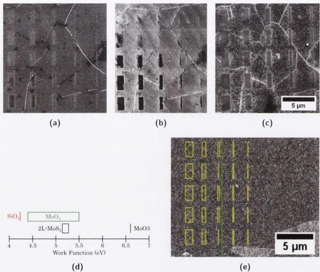
Figure 7.3: Scanning electron microscopy analysis of etching bilayer \text{MoS}_2 in a cumulative heating experiment. (a) to (c) is a selection of SEM micrographs at various steps of the cumulative heating process. (a) is after irradiation but before any heating. (b) is after heating to 305^\circ\text{C} . (c) is after heating to 330^\circ\text{C} . (d) shows the work functions of relevant materials. (e) is a low dose helium ion image overlaid with the patterns for irradiation.
