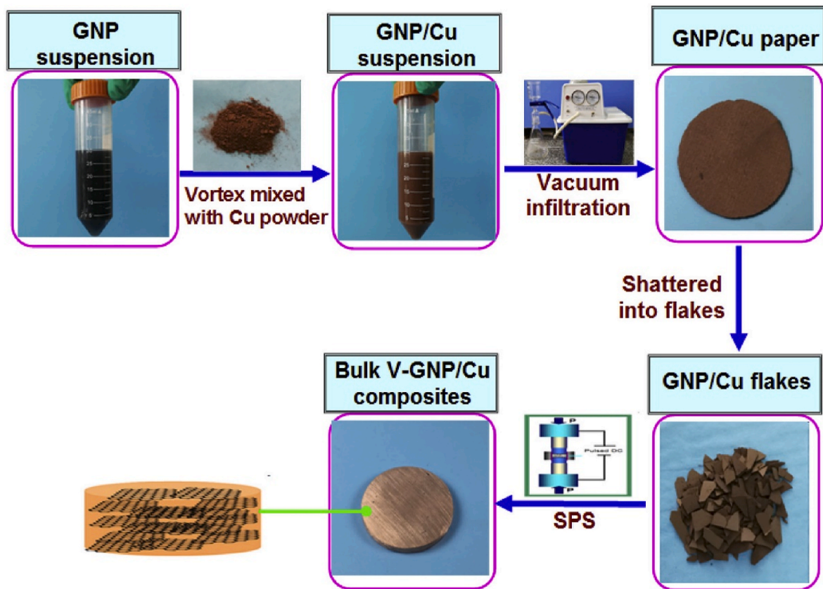
Fig. 17. Enhancing the copper powder with GNP suspension [49].
