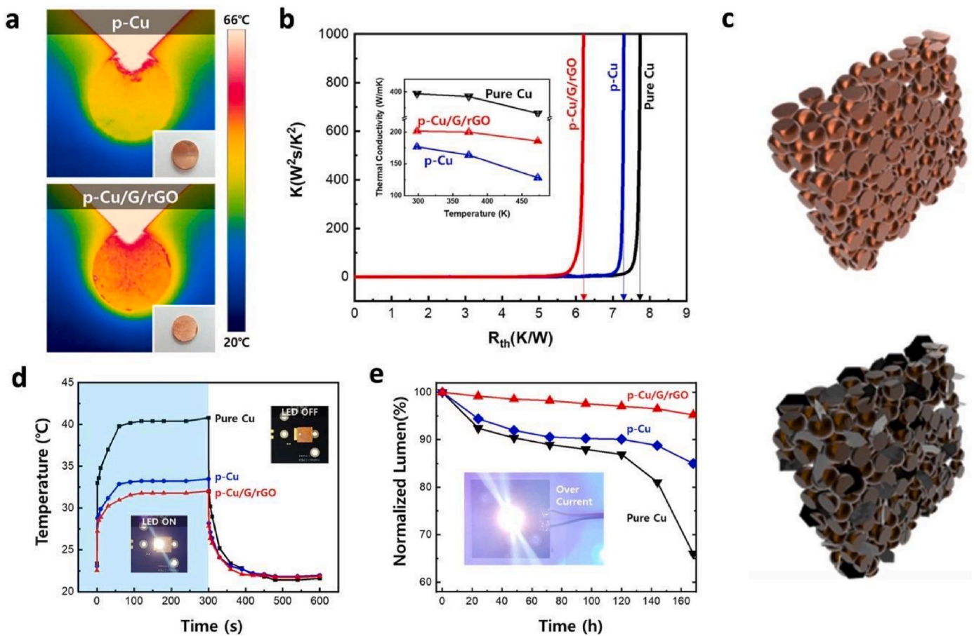
Fig. 30. Heat sink applications of copper-graphene porous structure for microelectronics cooling, processed by chemical vapour deposition and sintering: (a) Thermal infrared images of porous copper and porous copper-graphene, (b) Thermal resistance of LED device with porous heat sink, (c) Schematic images of porous copper (top) and porous copper-graphene (bottom), (d) Temperature distribution of LED devices with heat sinks under on- and off-state LED, (e) LED stability tests with heat sink based on light intensity measurements over time [393].
