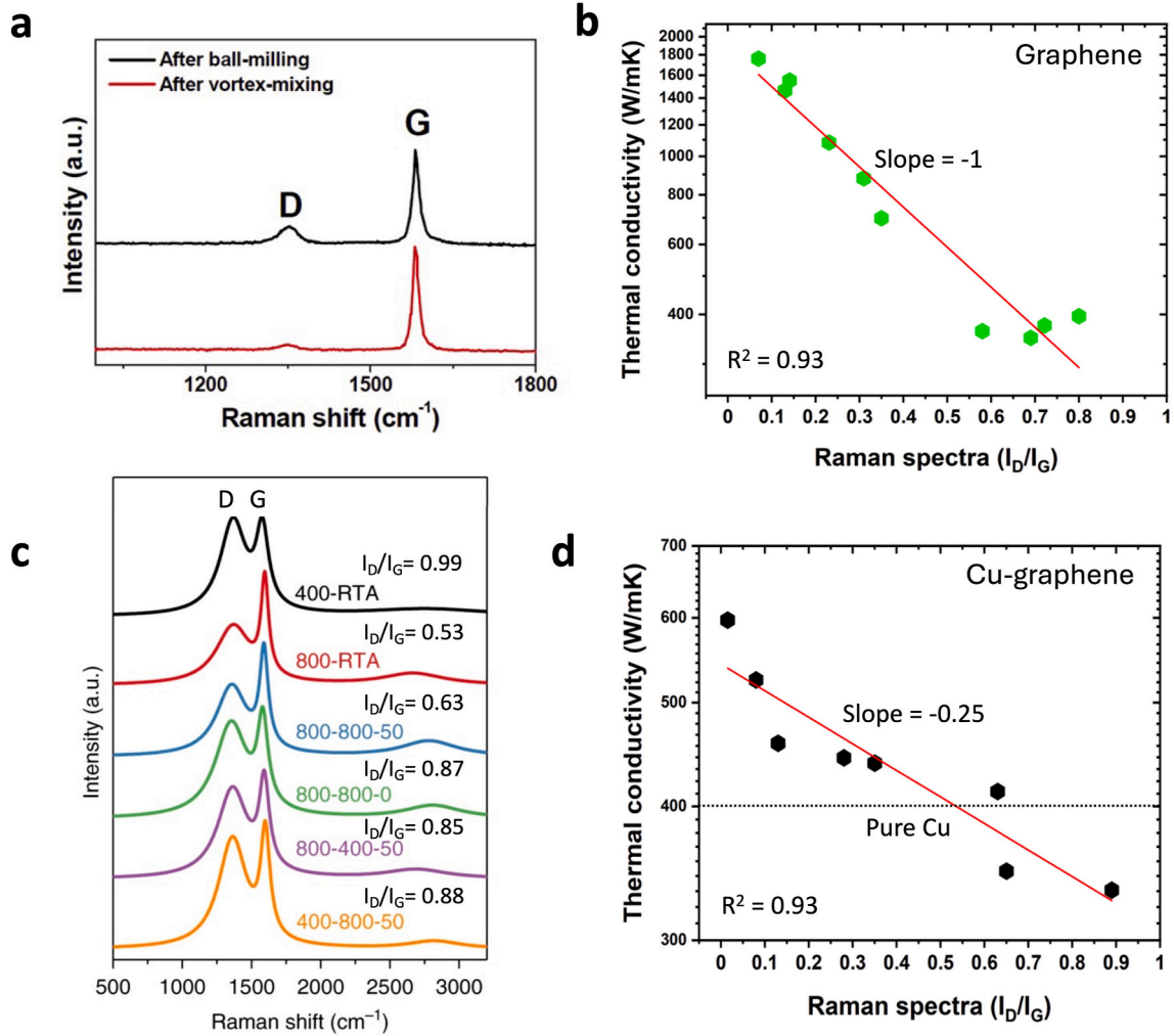
Fig. 25. (a) Raman spectra of graphene after different preparation methods, (b) Thermal conductivity as a function of I_D/I_G taken from the Raman spectrum, (c) Raman spectra of copper-graphene 2DMMC according to their fabrication conditions. The number in the first, second, and third positions presents the experimental condition for thermal annealing temperature, hot-pressing temperature in °C, and hot-pressing pressure in MPa. (d) Thermal conductivity values of copper-graphene as a function of the Raman ratio I_D/I_G taken from the Raman spectrum [49,64,66,327,330,336,338,339,350].
