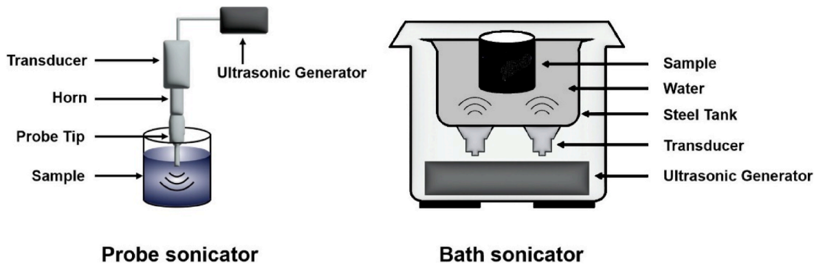
Fig. 12. Probe and bath sonicator as the two main tools for the sonication/shearing liquid exfoliation [155].
