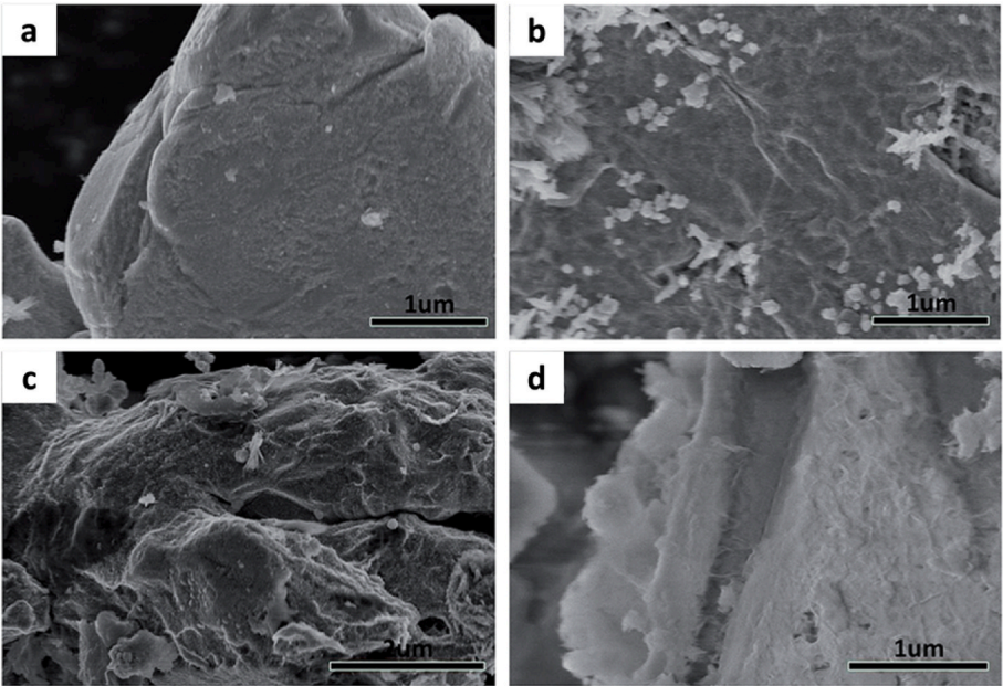
Fig. 14. SEM micrographs showing the morphology of copper powder coated with high-quality graphene throughout the ball milling process. (a) Initial copper powder before milling; (b and c) the surfaces of copper powder after being coated with high quality graphene through milling; (d) the edge of the copper powder coated with high quality graphene after milling [168].
