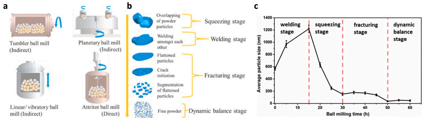
Fig. 2. (a) Schematic diagram illustrating ball milling processes including three indirect and one direct ball milling method, with the key components labelled [86, 87], (b) mechanism of powder particle size evolution and reduction in ball milling process, (c) correlation between milling duration and mean diameter of particles during the planetary ball milling process [98,99].
