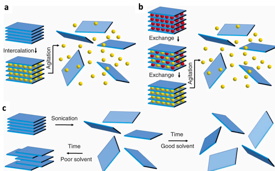
Fig. 11. The main liquid exfoliation mechanisms. a) ion intercalation, where ions inserted between layers swell the crystal and, agitation (shear, ultrasonication, thermal etc) separates the them into an exfoliated dispersion; b) ion exchange, where compounds change the surface charge and these ions are exchanged by larger ones, leading to exfoliation through agitation; c) sonication assisted exfoliation, where sonication in a solvent results in an exfoliation and nanosheet formation – the good solvents with appropriate surface energy provide efficient exfoliations, while the bad solvents cause reaggregation and sedimentation [124].
