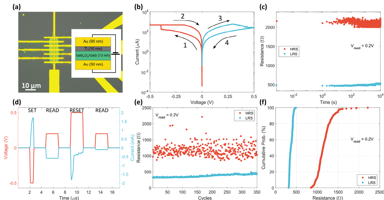
Figure 5. Oxidized GaS ReRAM element electrical characterization. a) Optical image of ReRAM element showing common bottom electrode with multiple top electrodes. Inset is a schematic of the vertical stack ReRAM. b) Typical DC switch cycle of ReRAM device where the device switches from HRS to LRS in the negative voltage regime and from LRS to HRS when voltage polarity changes. c) Resistance state retention over time measured at 0.2 V showing stable separation between HRS and LRS for 10^4 s. d) Representative single PVS SET and RESET measurement cycle of voltage and current showing a SET step followed by READ, and a RESET step followed by another READ. e, f) Endurance measurement and corresponding CDF plots read at 0.2 V.
