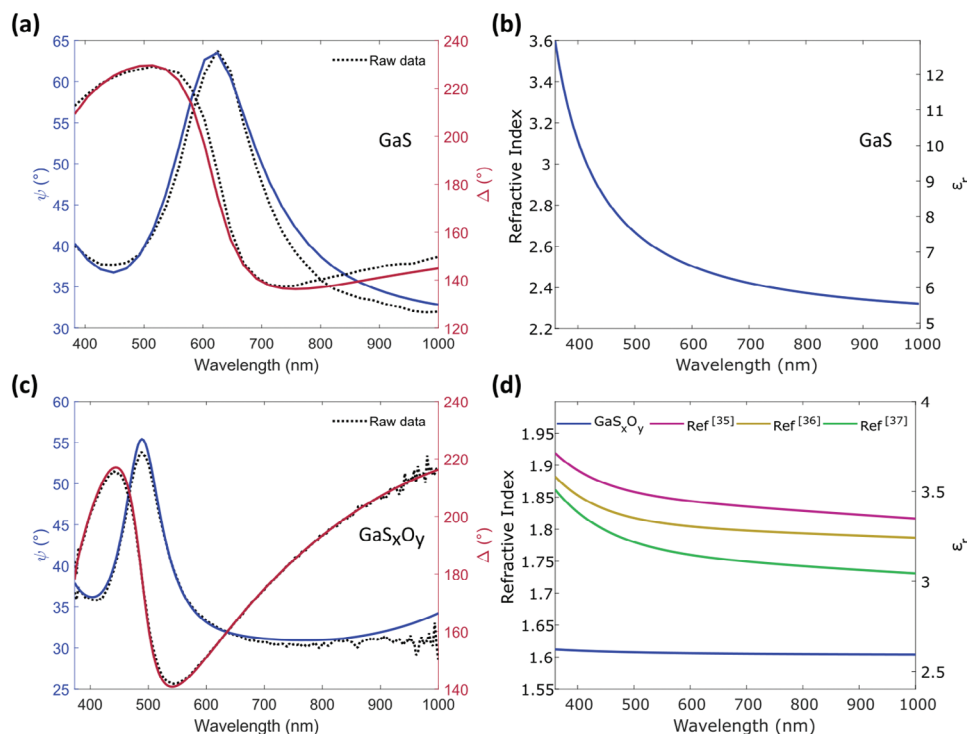
Figure 2. Spectroscopic imaging ellipsometry (SIE) of GaS and \text{GaS}_x\text{O}_y . a) \psi and \Delta spectra fitted using the Tauc–Lorentz oscillator model ( A = 94.3 \pm 17.2 eV, E_0 = 4.133 \pm 0.004 eV, E_g = 2.44 \pm 0.15 eV, and \Gamma = 0.05 \pm 1 eV). b) Corresponding refractive index and real part of the dielectric response. c) \psi and \Delta spectra of \text{GaS}_x\text{O}_y fitted using the Cauchy dispersion model ( A = 1.603 \pm 0.005 , B = 1177 \pm 1327 nm 2 , C = 0 \pm 1 nm 4 ). d) Refractive index and the corresponding real part of the dielectric response of the \text{GaS}_x\text{O}_y . Previously reported refractive index of amorphous \text{Ga}_2\text{O}_3 are included for comparison. [35–37]
