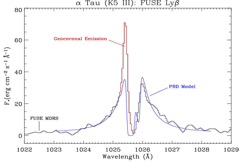
Figure 2. H Ly \beta profile of \alpha Tau and a partial redistribution (PRD) profile (Sim 1999) computed from the chromospheric model of McMurry (1999). The stellar PRD profile includes an ISM and wind+ISM model and is scaled by \times 1.15 to match the observed wings.
