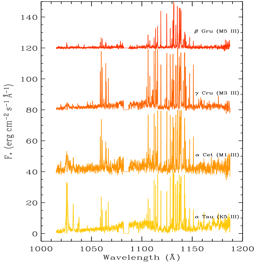
Figure 1. FUSE orbital night LiF spectra for the K and M giants, plotted as surface fluxes (each offset by 40). The break in data near 1080Å is from the space between the detector segments. The strongest fluorescent Fe II emission lines between 1106-1150Å have been clipped for clarity. These lines and the Cr II lines near 1060Å are pumped by H Ly \alpha from excited levels, and hence appear shortward of 1215Å. The rise shortward of C I continuum edge at 1100Å is clearly seen.
