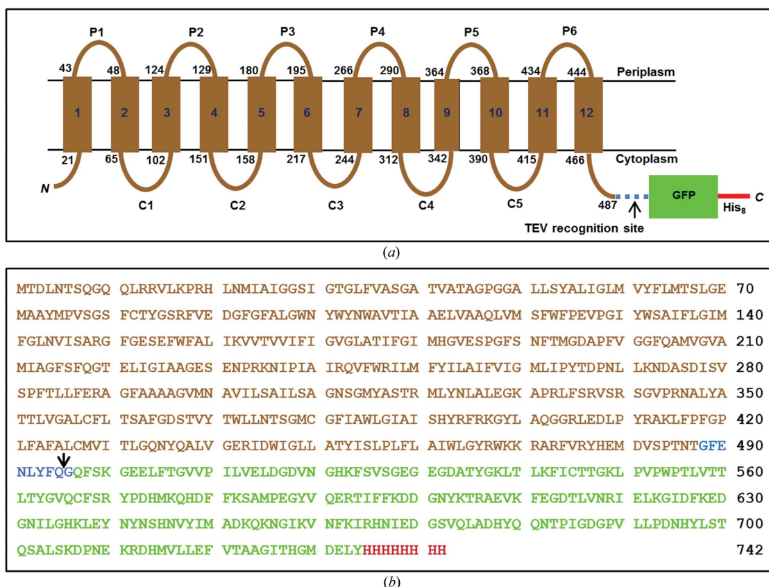
Figure 1 Schematic representation of the LysP-GFP 8His fusion construct. (a) The topology of LysP predicted by the TMHMM online server ( http://www.cbs.dtu.dk/services/TMHMM-2.0/ ) shows 12 transmembrane helices (numbered rectangles). The start and end residue numbers for each transmembrane helix are shown at the membrane boundary (black lines). P1–P6 and C1–C5 designate the periplasmic and cytoplasmic loops, respectively. The C-terminal GFP 8His fused to LysP via a linker that has a TEV protease recognition site (blue dashed line) is shown as a green box with the extension as a red line. The C m topology ensures that the GFP resides in the reducing environment of the cytoplasm, which is necessary for proper folding of this β-barrel reporter. (b) The deduced amino-acid sequence of the LysP-GFP 8His construct. Sequences corresponding to LysP, the TEV protease-containing linker, the GFP and the His tag are shown in brown, blue, green and red, respectively. The arrow marks the TEV protease cut site.
