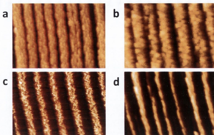
FIGURE 3.20: Fe nanowires with varying deposition angle
