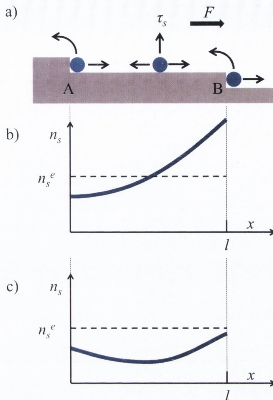
FIGURE 3.7: Schematic of adatom gradient effect on terrace of atomic step
