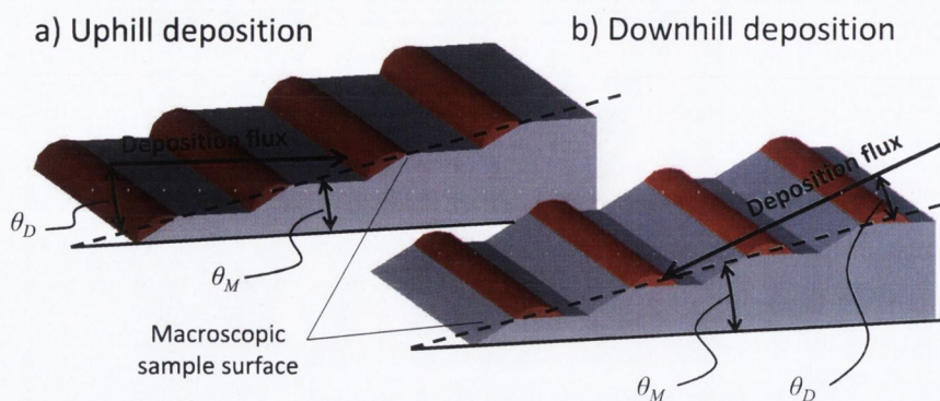
FIGURE 3.17: Glancing Angle Deposition Schematic
