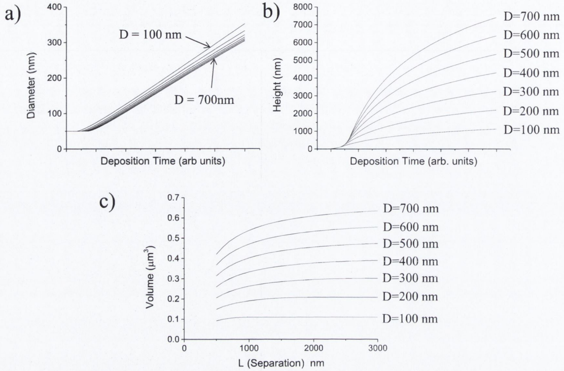
FIGURE B.2: Effect of varying values for the diffusion length ( D )
