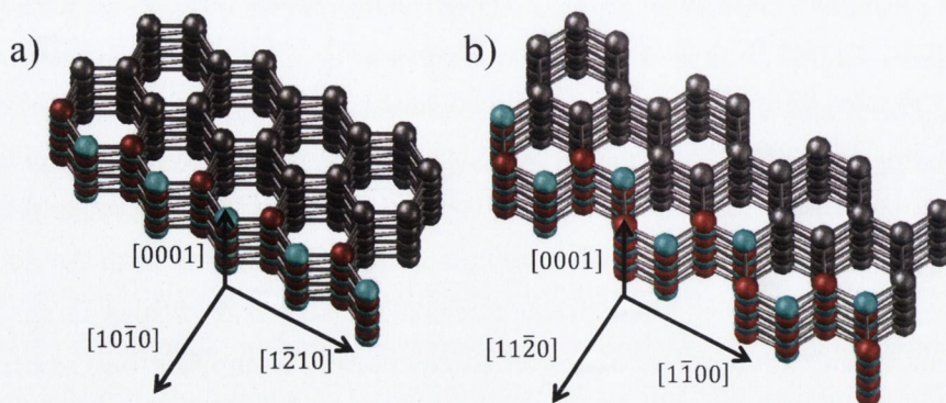
FIGURE 5.6: Two possible facets of wurtzite GaAs nanowire sidewalls.
