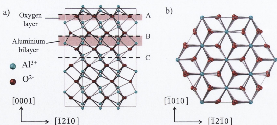
FIGURE 3.14: Side profile and C-plane of \text{Al}_2\text{O}_3
