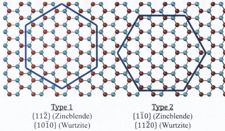
FIGURE 5.3: Different Hexagonal Facet Groups for Zincblende and Wurtzite Structures.
