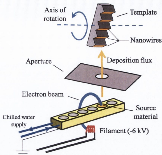
FIGURE 2.2: Glancing angle deposition schematic
