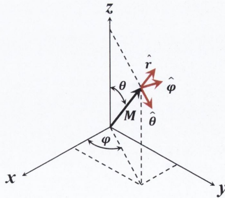
FIGURE A.1: Spherical co-ordinate system used in FMR
