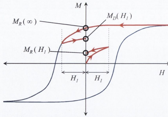
FIGURE 2.7: Schematic for finding M_R(H) and M_D(H) .
