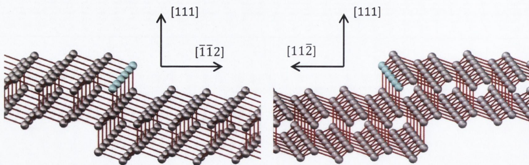
FIGURE 3.4: Single atomic steps on Si (111)
