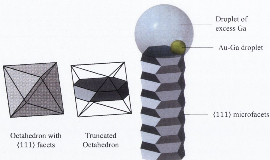
FIGURE 5.24: Schematic of nanowire with microfacets
