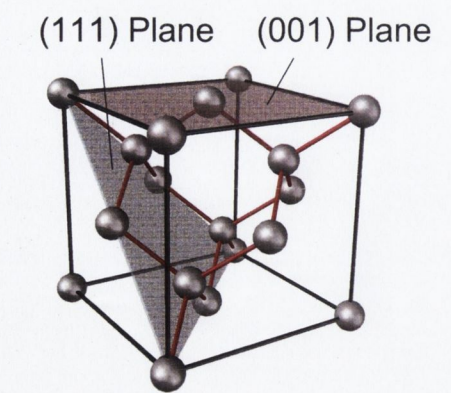
FIGURE 3.1: Unit cell of Si.
