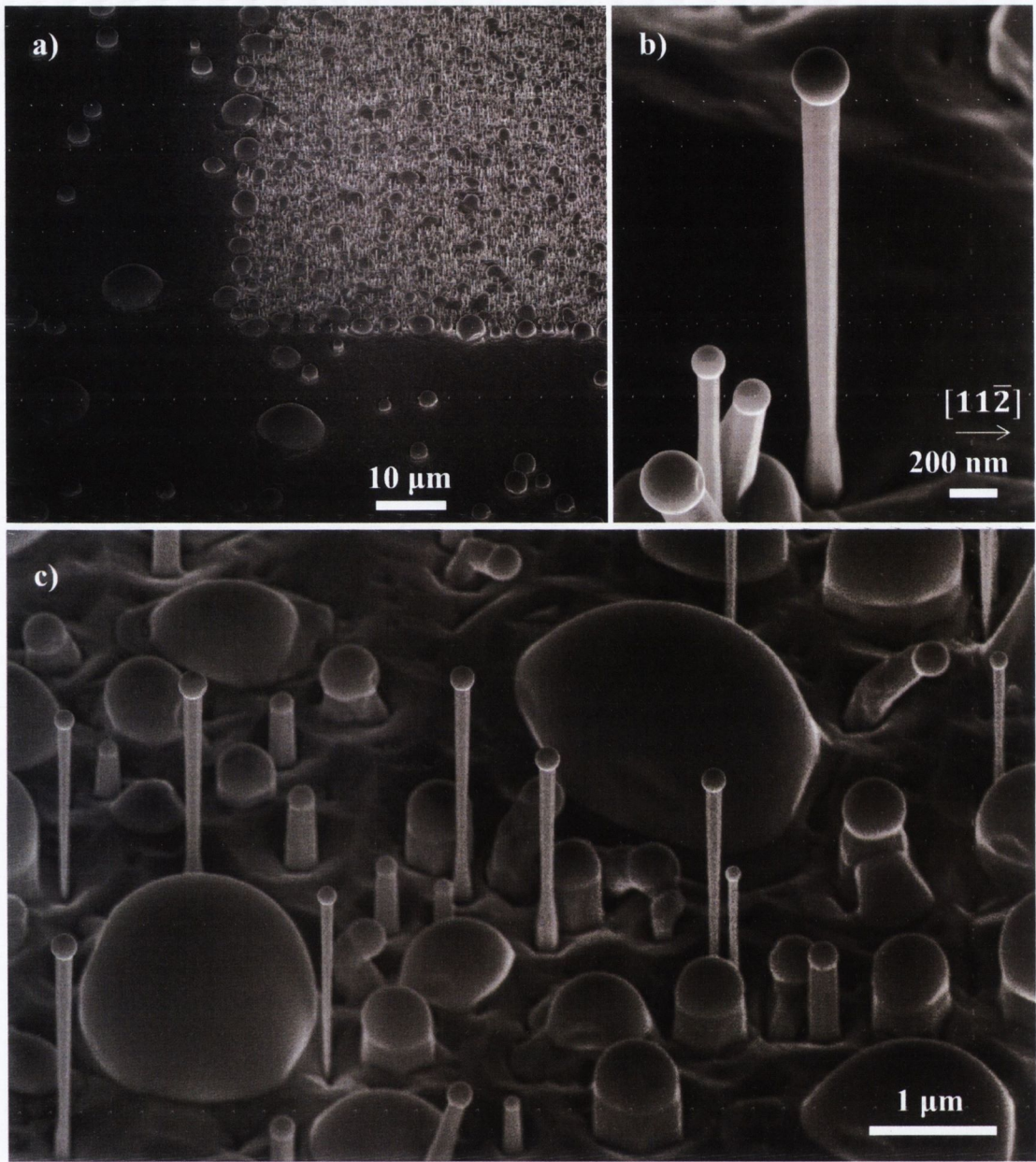
FIGURE 5.19: Nanowires grown from patterned arrays in As-limited regime
