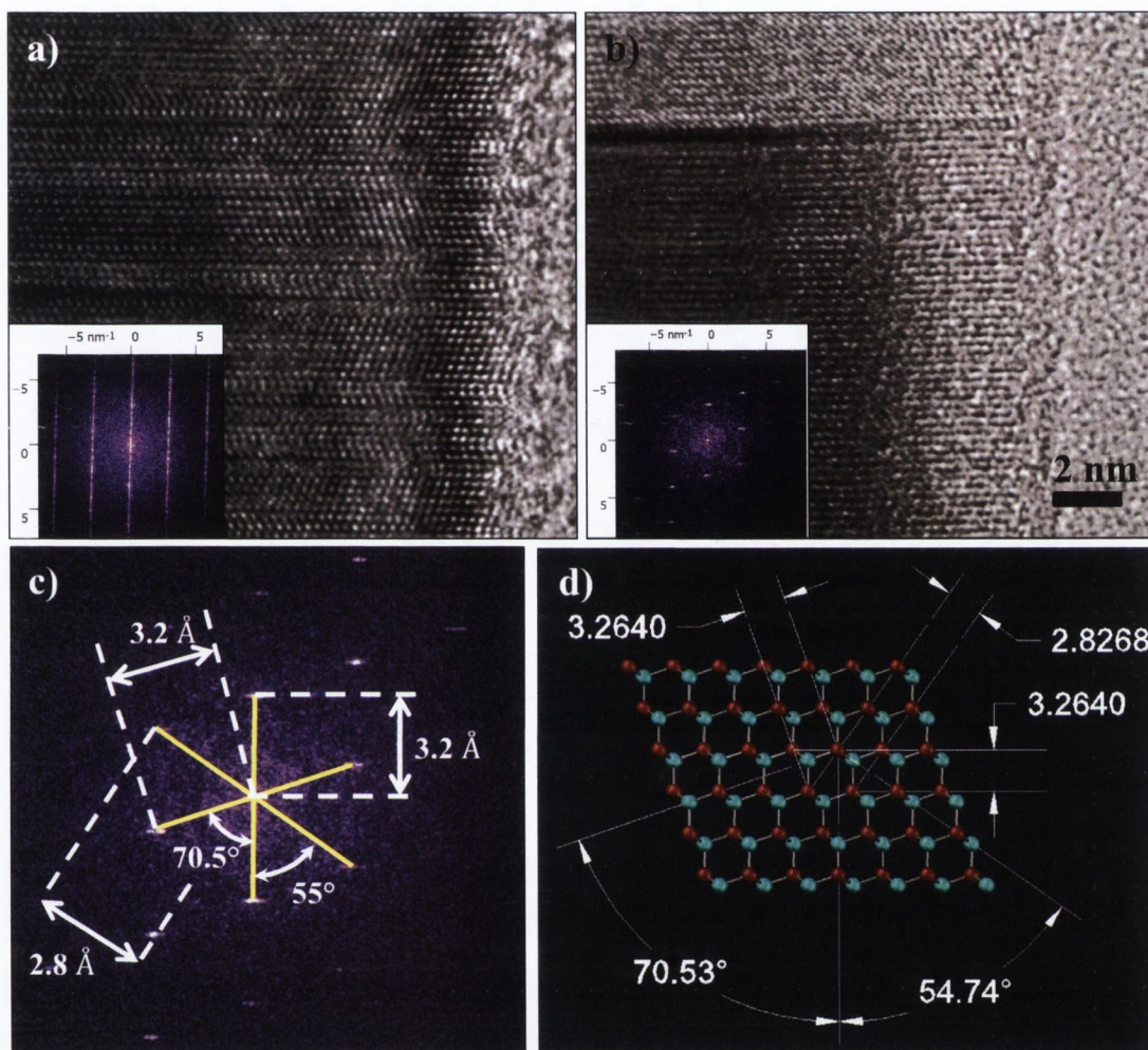
FIGURE 5.23: High resolution TEM images taken of a nanowire grown in As-limited conditions.
