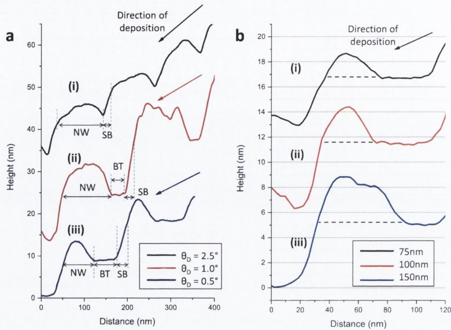
FIGURE 3.21: Height profiles across nanowires with varying deposition angle and thickness
