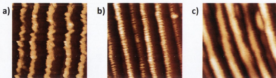
FIGURE 3.25: AFM data from arrays of nanowires composed of Co, Fe and Ni deposited in the uphill direction
