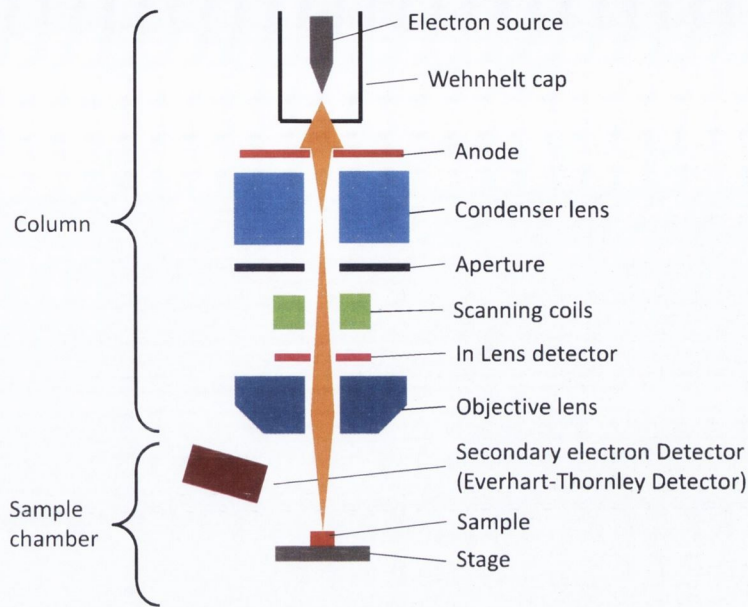
FIGURE 2.4: SEM Schematic
