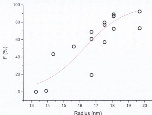
FIGURE 5.16: Probability of Nanodot initiating Wire Growth vs. Radius of Nanodot.
