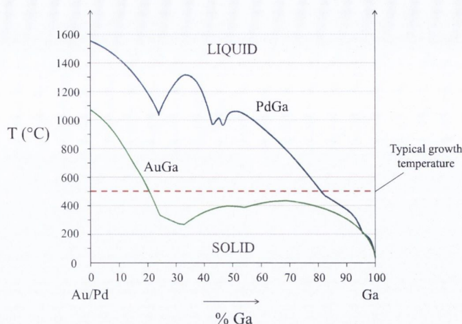
FIGURE 5.7: Liquid-solid phase boundaries for AuGa and PdGa alloys.
