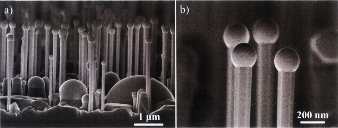
FIGURE 5.17: Nanowires grown in As-limited regime
