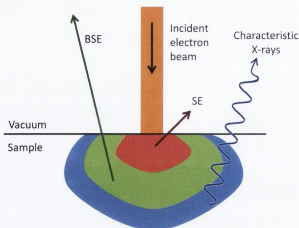
FIGURE 2.5: SEM Interaction Volume
