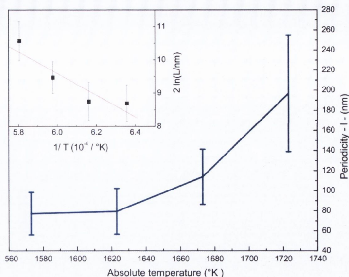
FIGURE 3.15: Dependence of periodicity of annealed \text{Al}_2\text{O}_3 substrates on temperature
