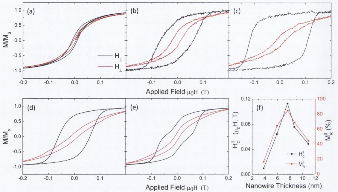
FIGURE 4.3: Shape Anisotropy of Fe nanowire arrays of varying thickness.
