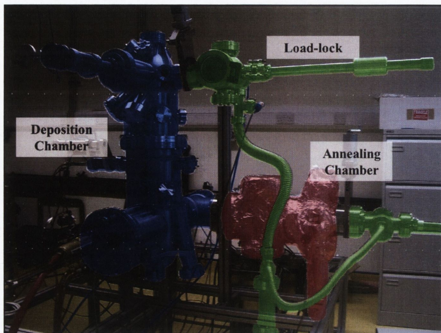
FIGURE 2.1: Chamber for glancing angle deposition and Si annealing
