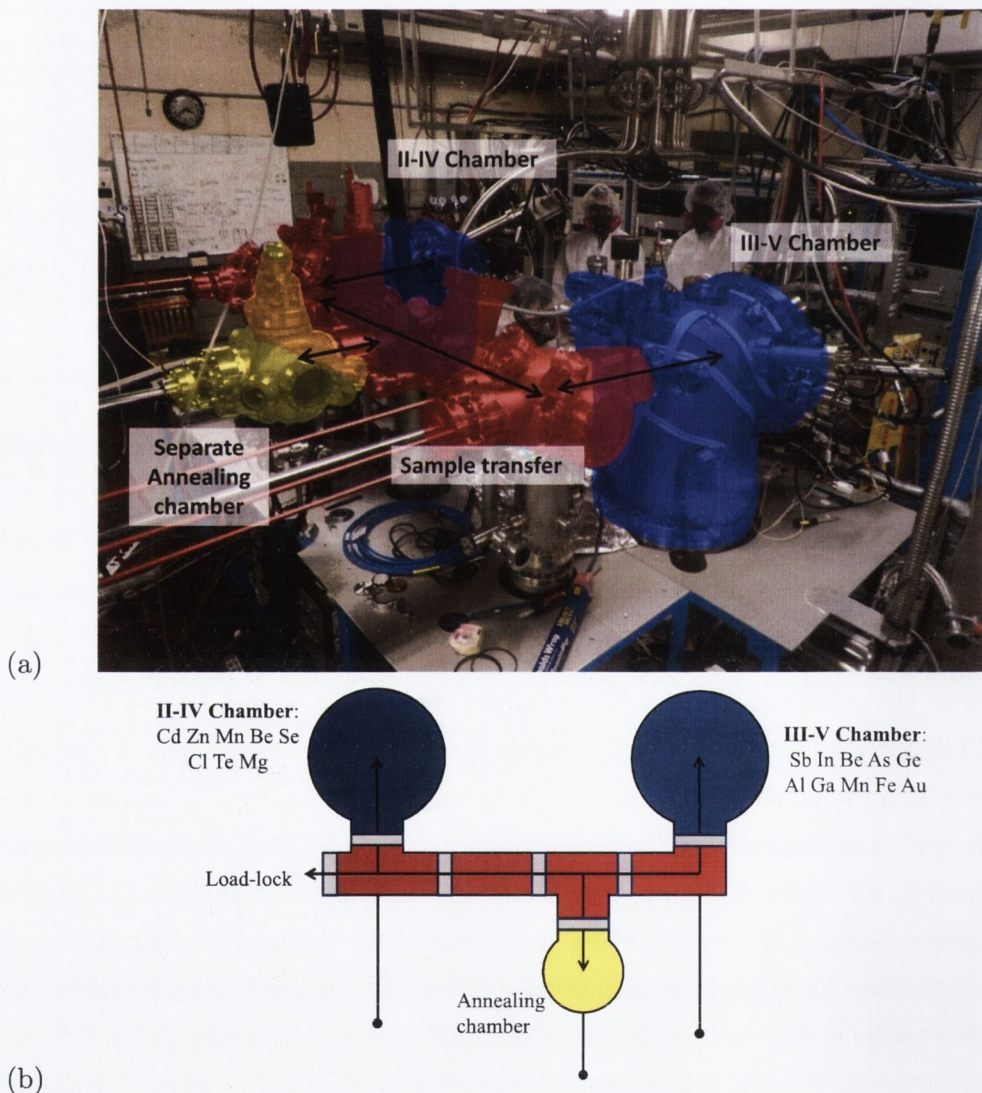
FIGURE 2.3: VLS Chamber
