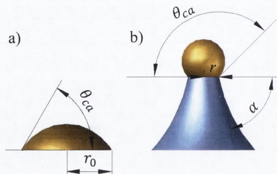
FIGURE 5.4: Schematic of contact angle and angle of inclination of sidewalls.
