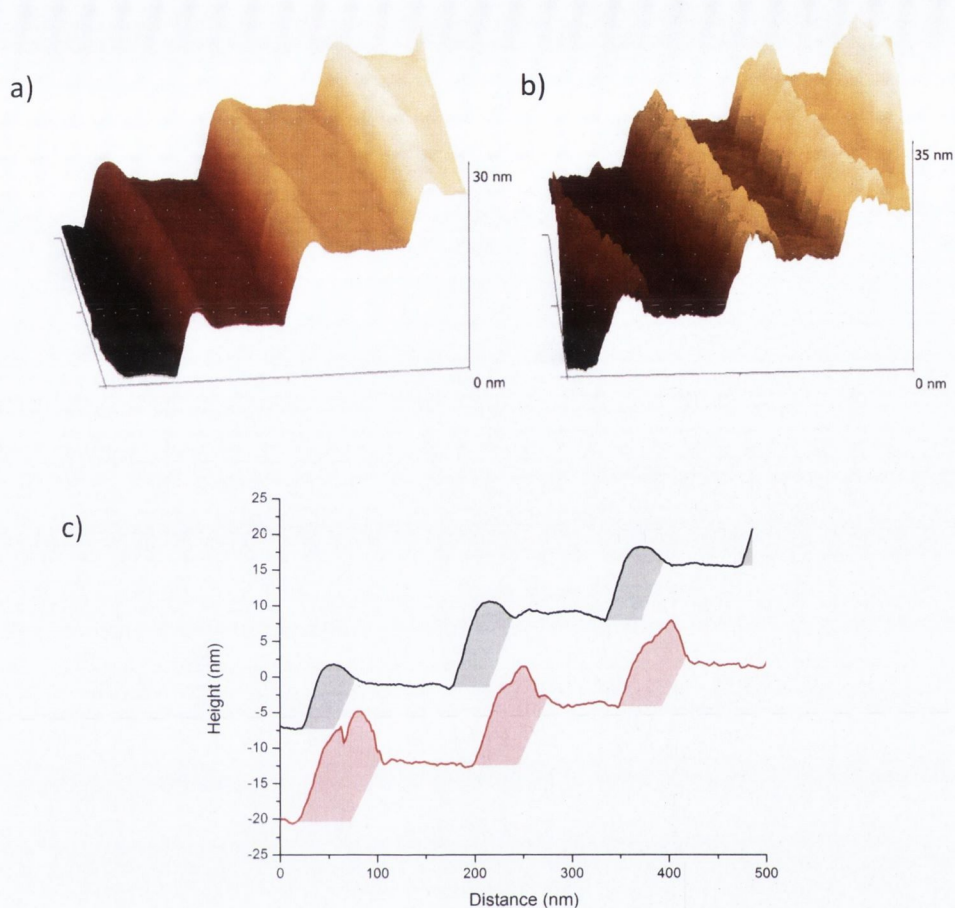
FIGURE 3.24: AFM data from Ni nanowire arrays with varying thickness
