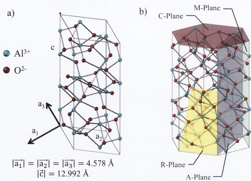
FIGURE 3.13: Crystal structure of \text{Al}_2\text{O}_3
