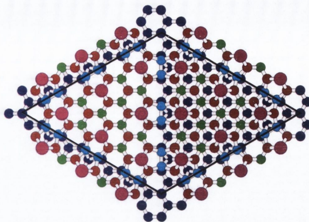
FIGURE 3.5: Si 7\times 7 reconstructed surface unit cell
