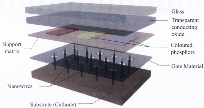
FIGURE 1.1: Typical FED design incorporating nanowire array
