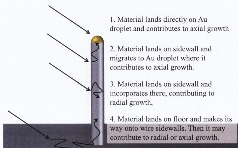
FIGURE 5.1: Routes of Ga to growth interface
