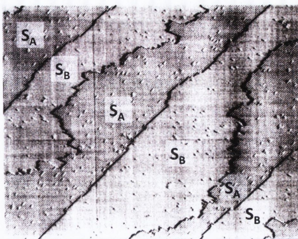
FIGURE 3.2: Atomic steps on Si(001)
