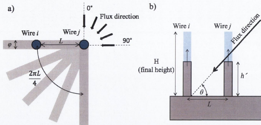
FIGURE B.1: Schematic of shadowing considerations
