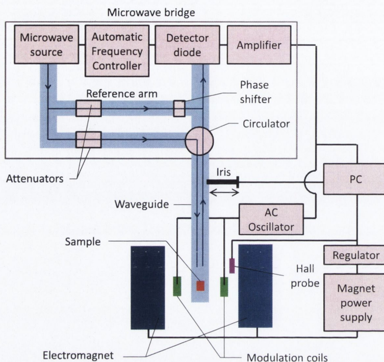
FIGURE 2.9: FMR Setup Schematic
