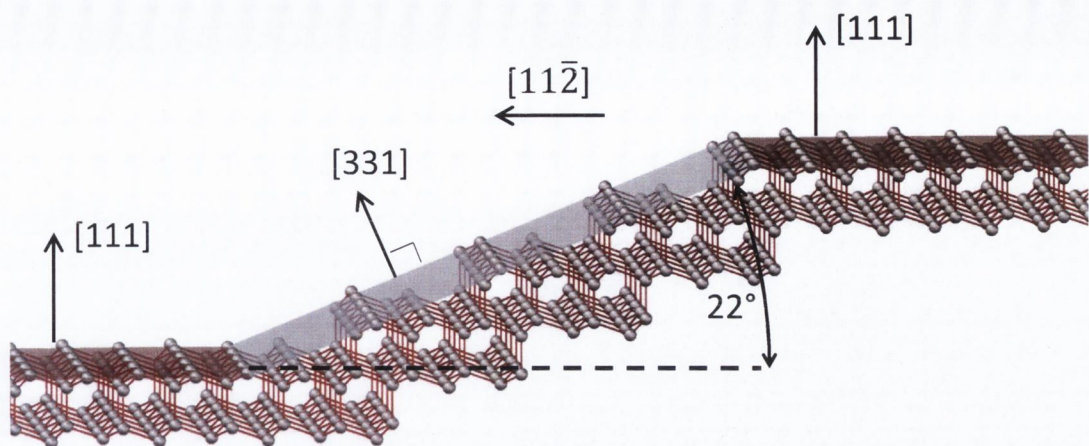
FIGURE 3.8: Two Si (111) terraces separated by a (331) facet
