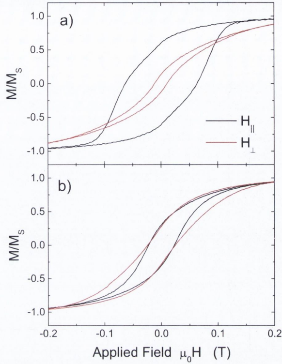
FIGURE 4.8: M - H loops for samples in Henkel analysis.
