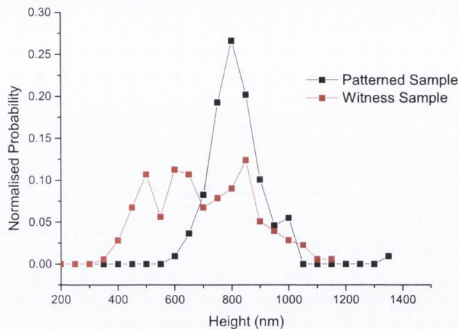
FIGURE 5.9: Height Distributions for Ordered and Random Nanowire Arrays.
