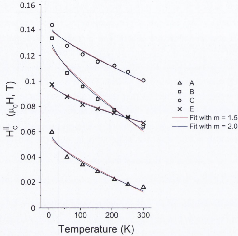
FIGURE 4.6: Dependency of coercivity of Fe nanowire arrays as a function of temperature
