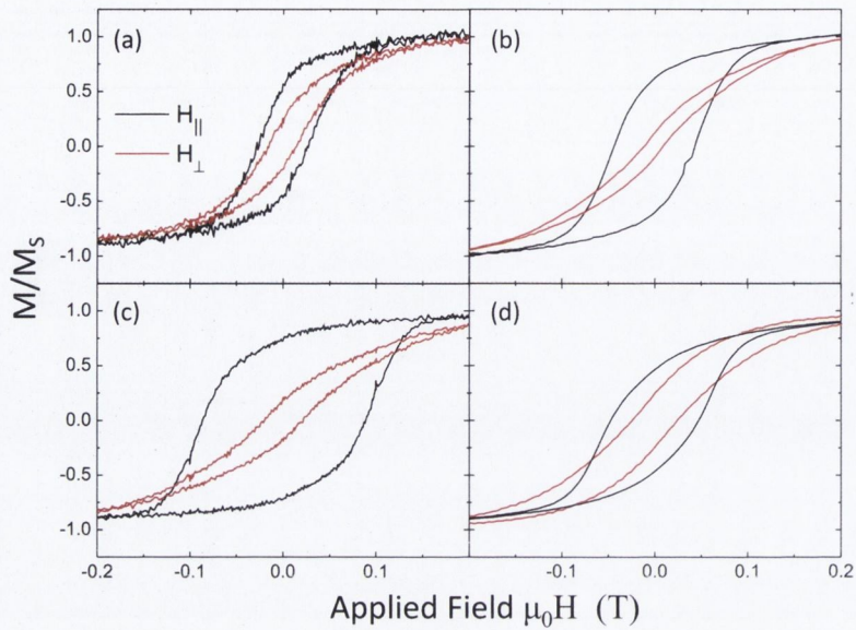
FIGURE 4.5: Shape Anisotropy of Co nanowire arrays of varying thickness.
