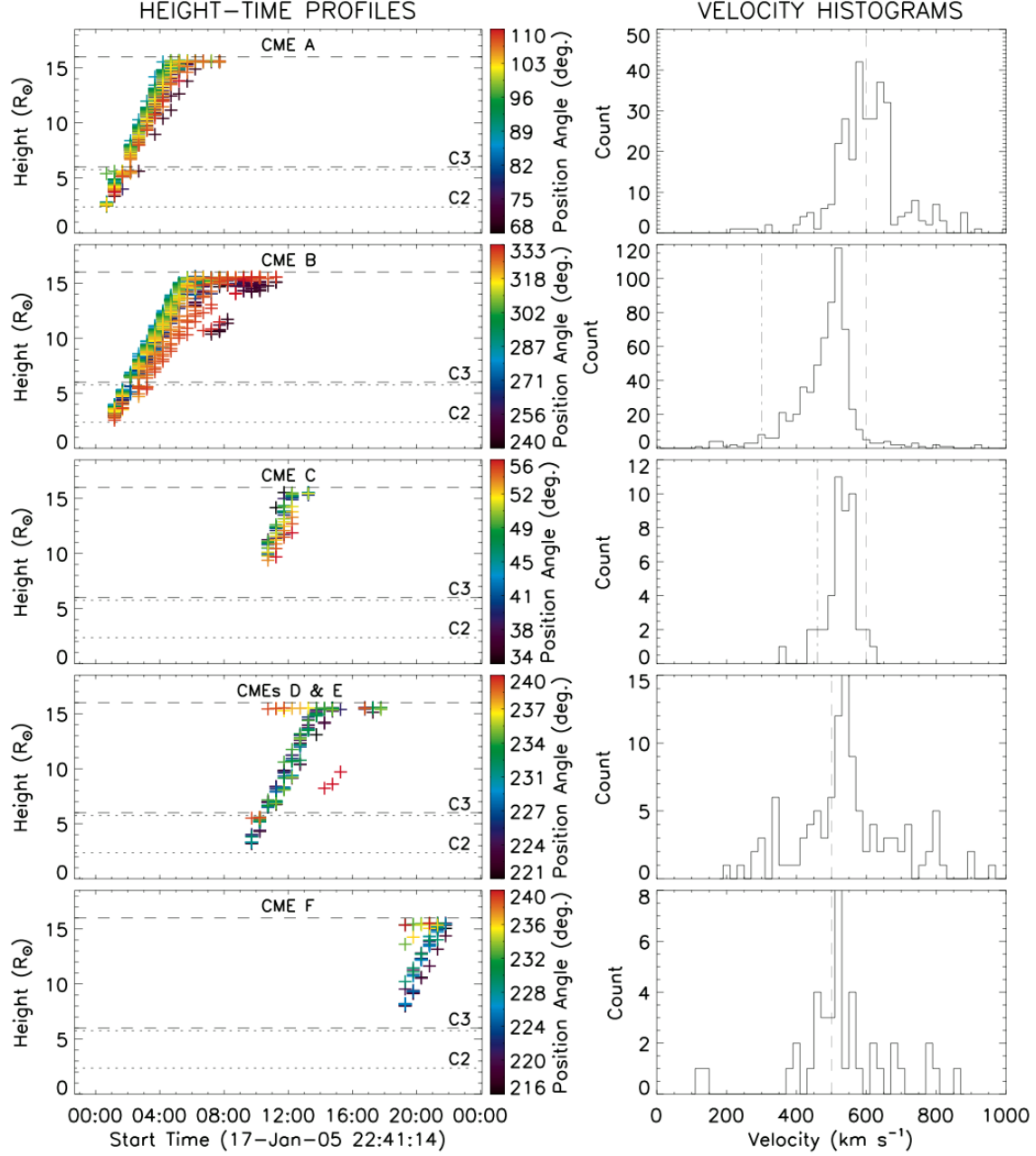
Fig. 9.— Left: The height-time profiles resulting from the regions in the model detection stack (Fig. 7) corresponding to CMEs A through F, where the detection of CME E is not distinguishable from CME D. The position angle corresponding to each height measurement is indicated by the associated colorbar. Right: The derived velocities, displayed in bins of 20 \text{km s}^{-1} , where the dashed lines indicate the model velocities of 500 and 600 \text{km s}^{-1} , and dot-dashed lines for CMEs B and C indicate the limit of apparent velocity deviation due to projection effects (300 and 460 \text{km s}^{-1} respectively).
