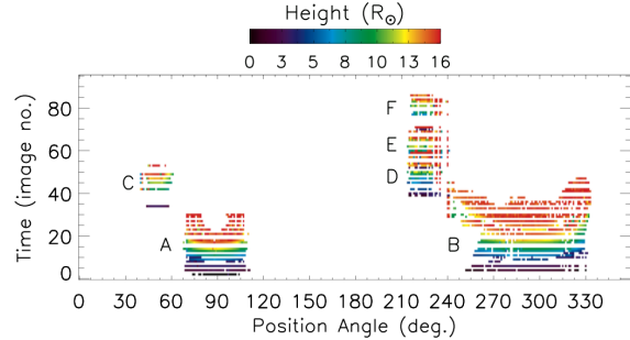
Fig. 7.— The model CME detection stack, plotted in time, i.e., image number, against position angle measured counter-clockwise from solar north. The intensity corresponds to the height of the outermost points in the detection relative to Sun-center.
