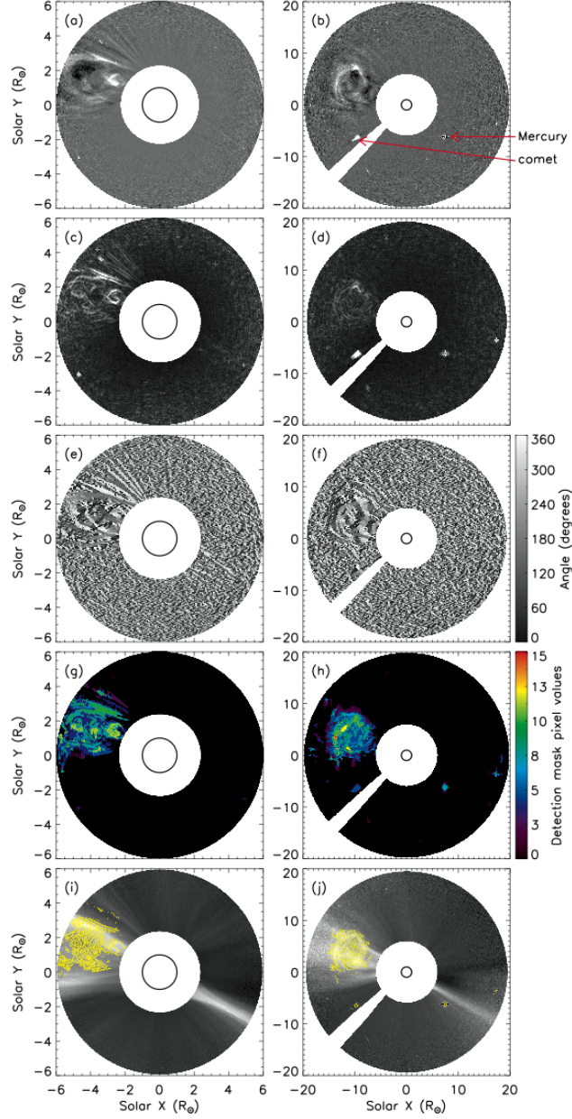
Fig. 1.— Output of the CORIMP automated techniques applied to images of a CME on 2010 March 12 from the LASCO/C2 (a) and C3 (b) coronagraphs at times 05:06 and 11:42 UT respectively. The images have been processed using the NRGF and quiescent background separation technique outlined in Paper I to isolate the dynamic coronal structure. A comet and the planet Mercury are also observed in the C3 field-of-view. (c) and (d) show the magnitude information (edge strength), and (e) and (f) show the angular information, at a particular scale of the multiscale decomposition outlined in Section 2.1. (g) and (h) show the resulting CME detection masks following the scoring system outlined in Section 2.2. (i) and (j) show the final CME structure detection overlaid in yellow on the C2 and C3 images (with reduced intensity scaling to better view the overlaid edges). The edges were determined using a pixel-chaining algorithm on the magnitude and angular information of the multiscale decomposition.
