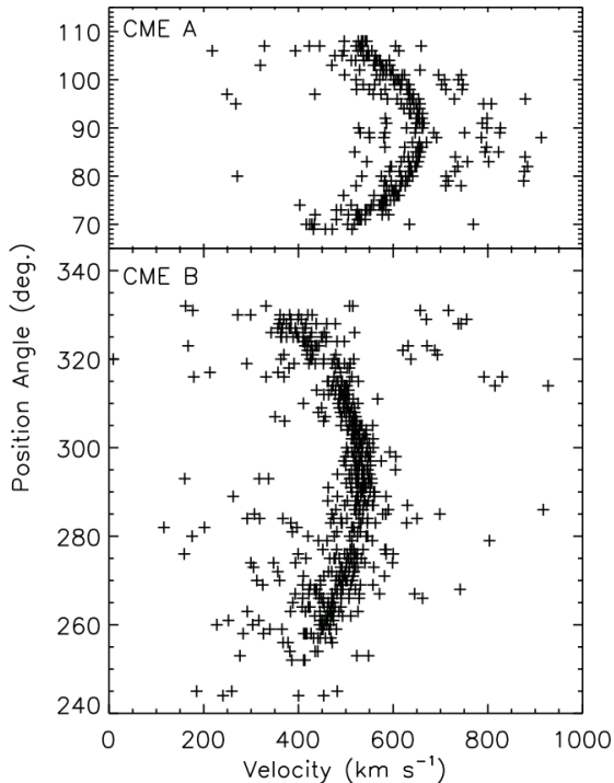
Fig. 8.— The derived velocities of CMEs A (top) and B (bottom) for each position angle of the corresponding detections displayed in Figure 7. The velocities are shown to cluster in such a manner as to indicate an appreciable expansion of each CME, with the flanks moving slower than the apex in both cases. This is an important characteristic when considering the forces acting on a CME as it propagates.
