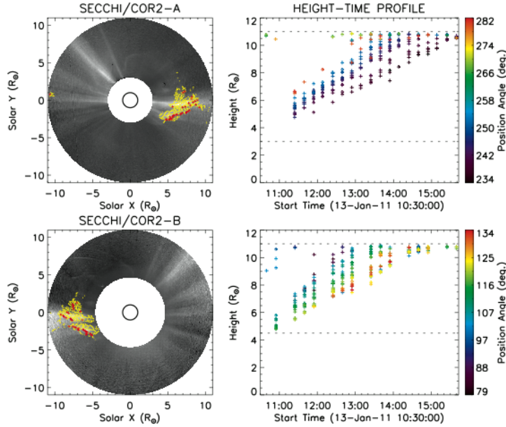
Fig. 4.— A sample output of the CORIMP automatic CME detection and tracking technique applied to SECCHI/COR2 A and B images for 2011 January 13. The CME appears as a partial halo in the STEREO observations, and parts of its front are too faint to be fully detected in the images. A corresponding animation of this event is shown in the online material.
