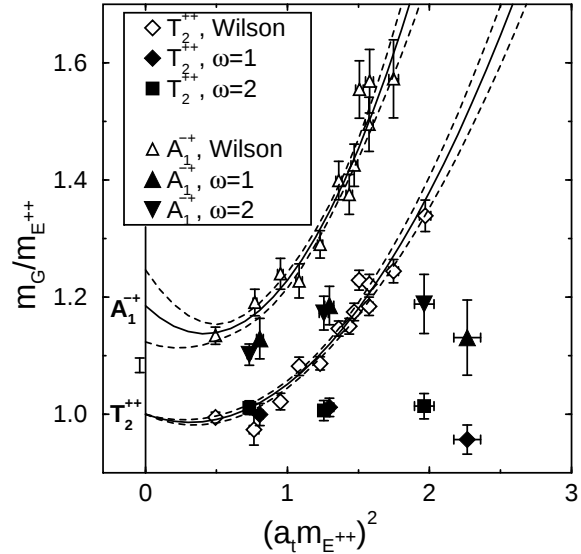
Figure 4. Scaling properties of the T_2^{++} and A_1^{-+} irreps. Filled symbols indicate S_\omega data.
