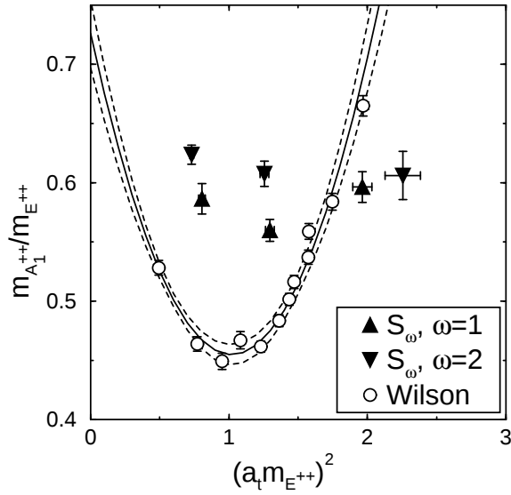
Figure 3. Scaling properties of the scalar of S_\omega .
