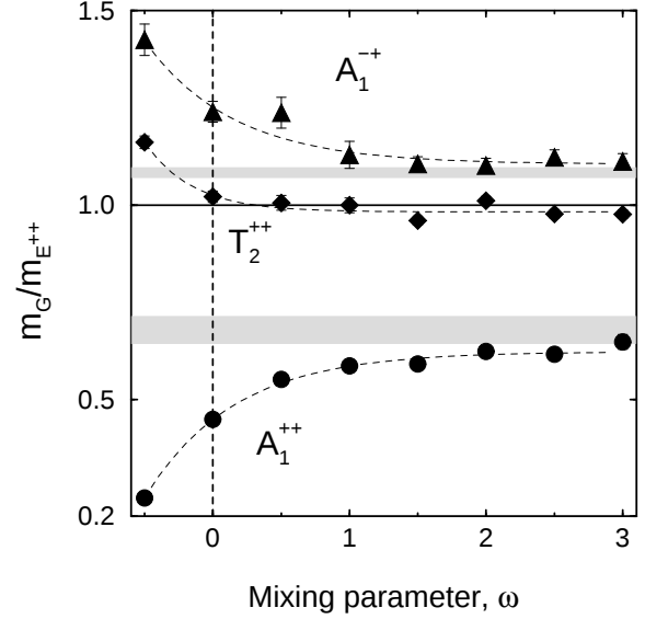
Figure 2. Glueball mass ratio dependence on the two-plaquette mixing parameter \omega for the A_1^{++}, T_2^{++} and A_1^{-+} irreps at fixed \beta . The horizontal bands indicate the continuum limit. Dashed lines guide the eye.
