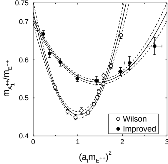
Figure 1. The effect of Symanzik improvement on the scalar glueball.
