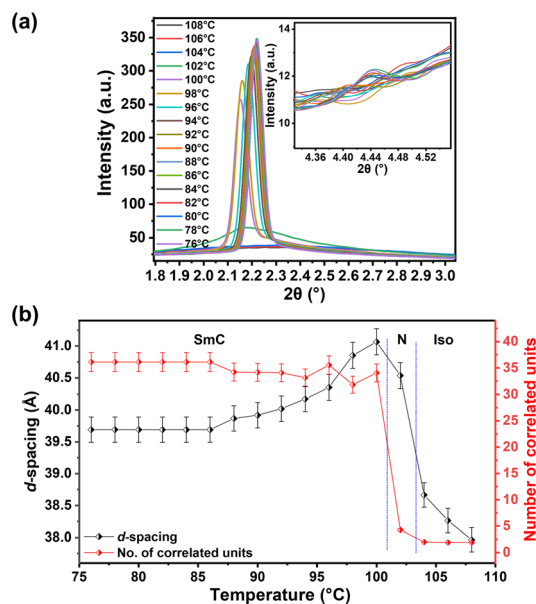
Fig. 5 (a) Temperature-dependent SAXS data for F4-16a . The inset shows an additional small-angle peak confirming the periodic layered structure of the SmC phase. (b) Variation of d -spacing and the number of correlated units with respect to temperature for F4-16a .
