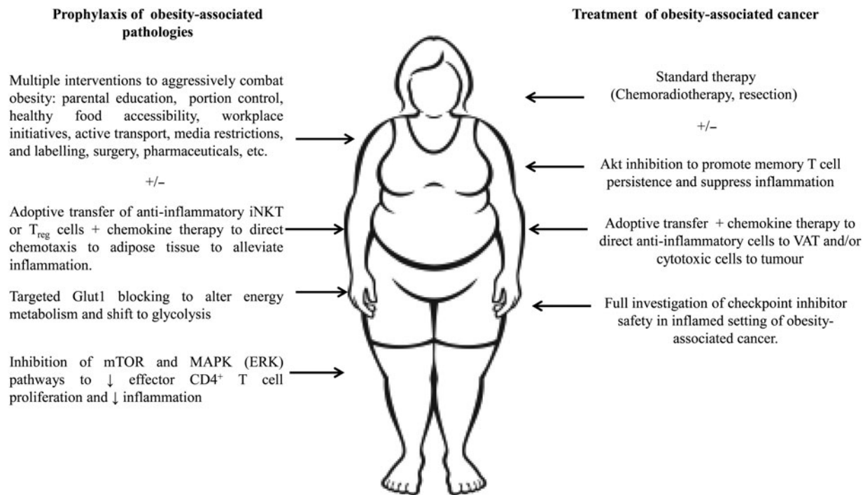
Fig. 1. Future approaches for the prevention and treatment of obesity-associated cancer (10,11,139). iNKT, invariant natural killer T cells; T_{reg} , regulatory T cells; mTOR, mammalian target of rapamycin; MAPK (ERK), mitogen-activated protein kinase (extracellular signal-regulated kinase); VAT, visceral adipose tissue.
