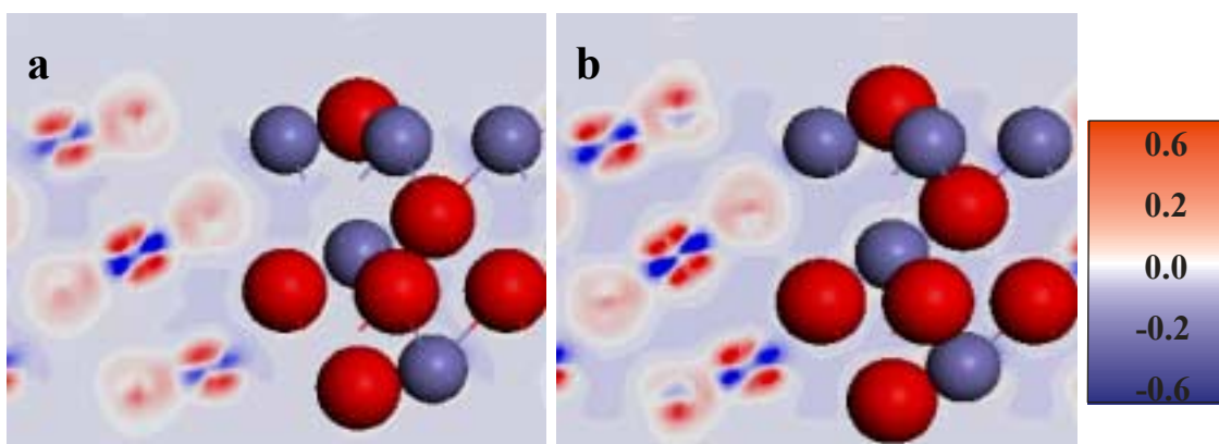
Fig.3. Cross-sectional view of the FeO vacuum slab and charge density difference distribution for stretched (a) and compressed (b) FeO, corresponding to in-plane lattice constants of 3.1 Å and 2.8 Å, respectively.
