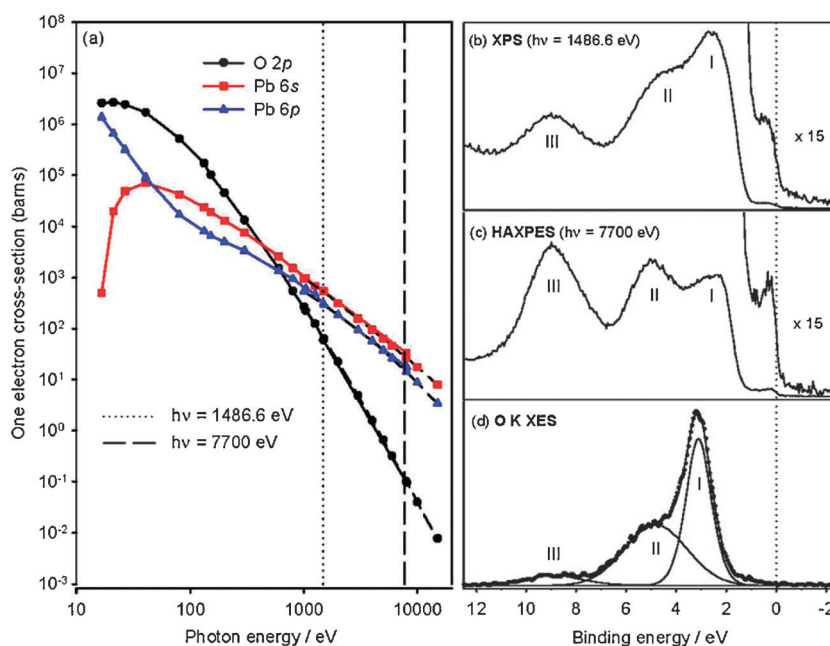
Fig. 5 (a) One electron photoionisation cross-sections of Pb 6s (squares), Pb 6p (triangles) and O 2p (circles) orbitals as a function of photon energy. Valence and conduction band photoelectron spectra of PbO 2 measured at (b) h\nu = 1486.6 eV and (c) h\nu = 7700 eV. (d) O K shell X-ray emission spectrum.
