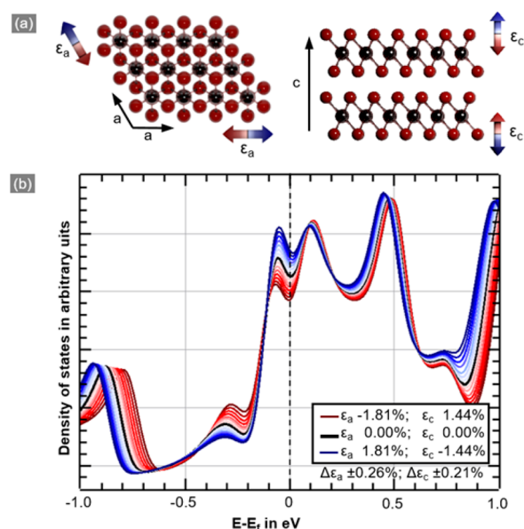
Figure 5. (a) Top and side view of the PtSe 2 bulk shown with the in-plane, a , and out-of-plane, c , lattice vectors, and the direction of the applied strain ( \epsilon_a and \epsilon_c ). (b) Density of states close to the Fermi level (shifted to zero) under applied tensile strain and compression.
