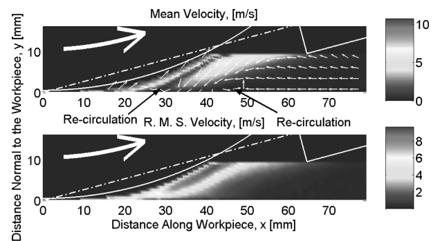
(a) Velocity Flow Fields; V_{\text{wheel}} = 10 m/s; V_{\text{jet}} = 10 m/s
