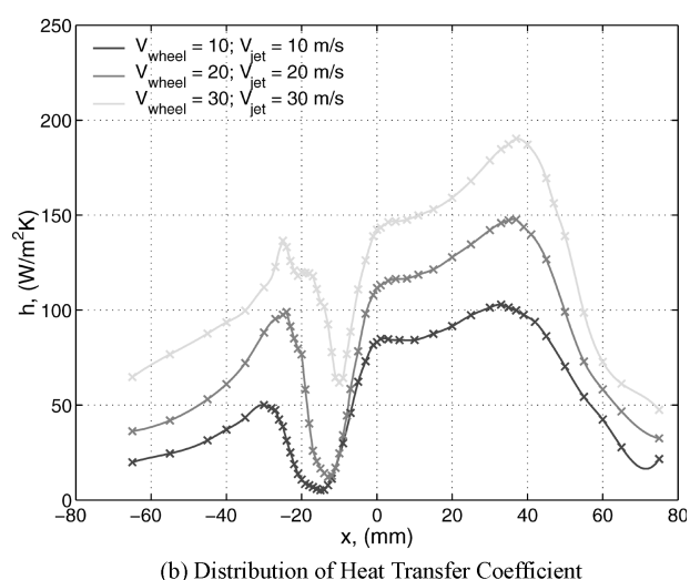
Fig. 6 Fluid flow and heat transfer due to jet cooling of a grinding process: \alpha = 15^\circ and H = 101 mm
