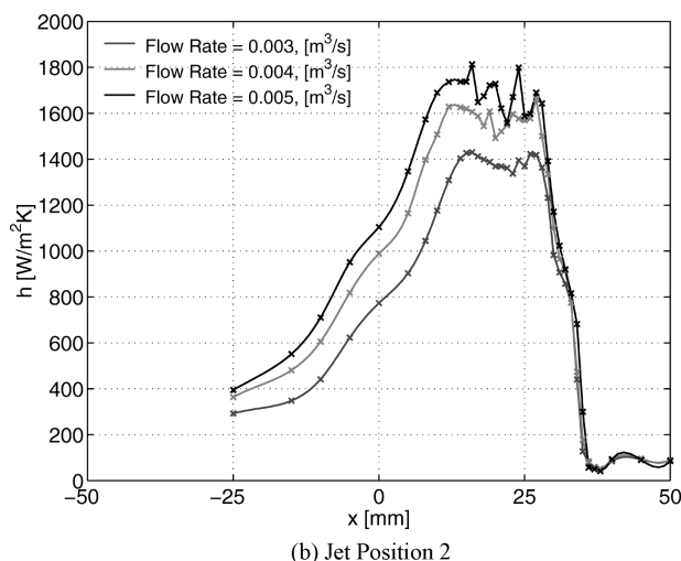
Fig. 9 Wheel and high-speed impinging jet heat transfer distributions
