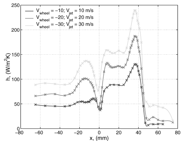
(b) Distribution of Heat Transfer Coefficient
