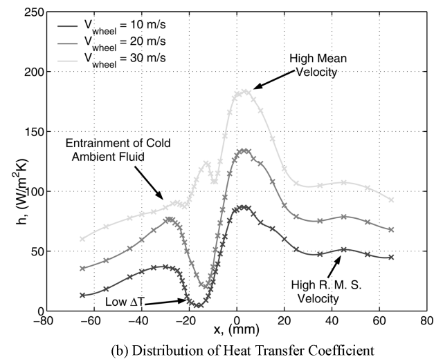
Fig. 4 Fluid flow and heat transfer due to rotating grinding wheel
