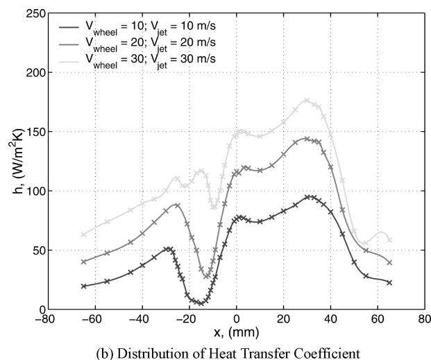
Fig. 5 Fluid flow and heat transfer due to jet cooling with rotating grinding wheel: \alpha = 30^\circ and H = 101 mm
