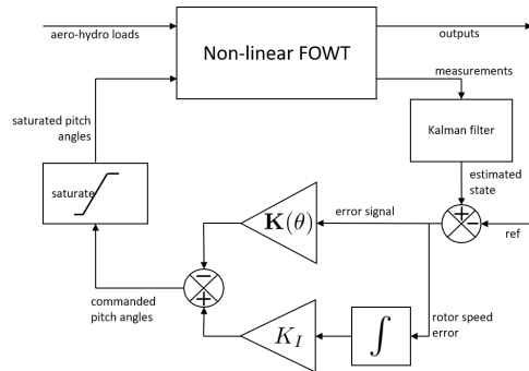
Figure 1. Controller schematic
