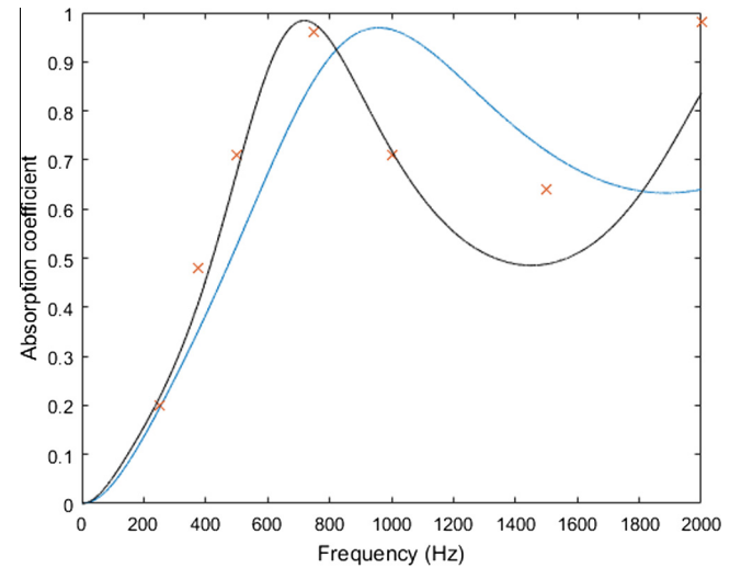
Fig. 9. Predicted absorbance for \alpha_\infty = 2.3 (blue) and \alpha_\infty = 4 (black) with experimental results (red) for medium-density loose shiv. (For interpretation of the references to colour in this figure legend, the reader is referred to the web version of this article.)
