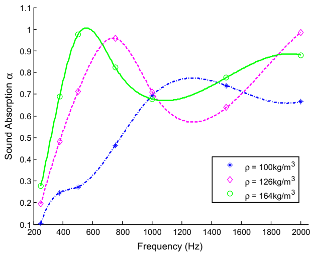
Fig. 4. Sound absorption characteristics of loose hemp shiv, for different levels of compaction.
