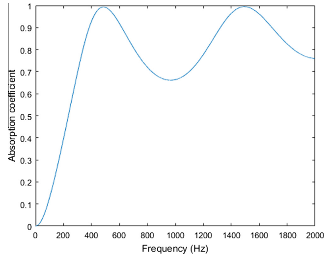
Fig. 8. Absorbance of a sample of loose shiv, from Gle et al.
