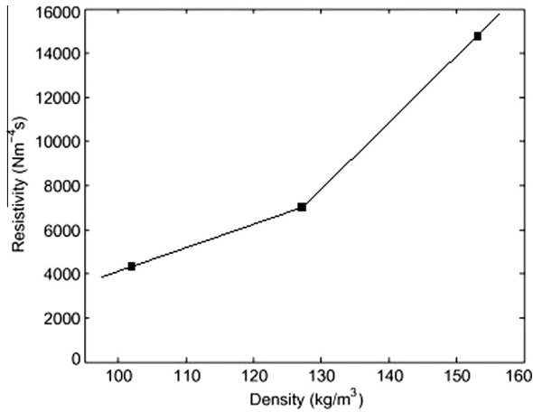
Fig. 7. Relationship between density and airflow resistivity from Gle et al. (linear extrapolation lines added).
