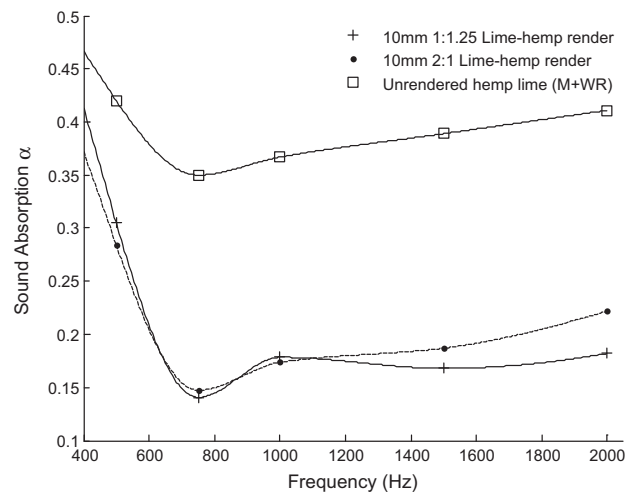
Fig. 6. Sound absorption of rendered hemp-lime concrete walls in the range 500–2000 Hz.
