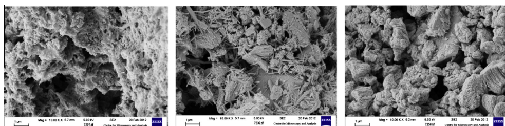
Fig. 2. SEM images of (left) BM, (middle) CM, (right) G binder hemp concrete matrices.
