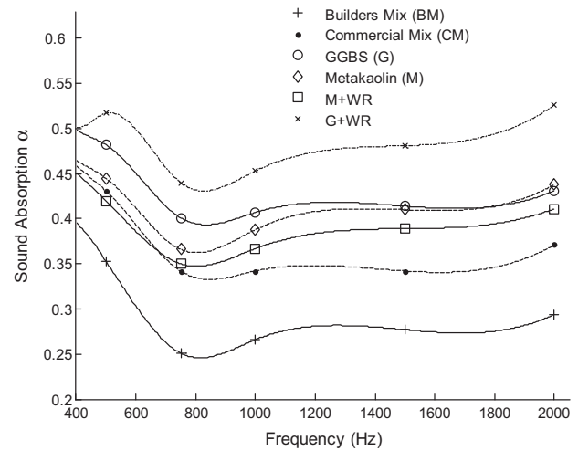
Fig. 5. Sound absorption of hemp-lime concrete walls with different binders in the range 500–2000 Hz.
