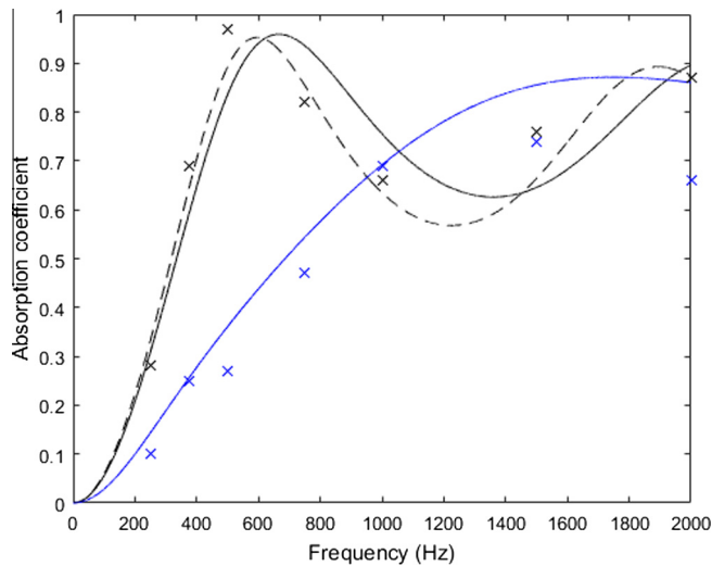
Fig. 10. Low-density shiv ( \alpha_{\infty} = 1 , blue) and high-density shiv ( \alpha_{\infty} = 4 , solid black, and \alpha_{\infty} = 5 , dashed black). (For interpretation of the references to colour in this figure legend, the reader is referred to the web version of this article.)
