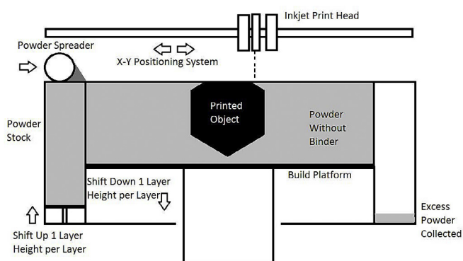
Fig. 1. Representation of the Binder Jetting Process, adapted from Gibson et al., 2010.
