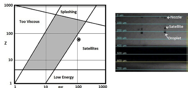
Fig. 5. Left: Interactive Jettability Model (redrawn from the online interactive tool developed by Abbott (2016)) indicating potential for satellite droplet formation given the calculated Z value for an ink with xanthan gum. Right: Evidence of satellite droplets when using the Dimatix Drop Watcher on an ink formulation. The increments on the left hand side indicate distance from the nozzle and can be used to calculate droplet speed whilst using the real time movie function.
