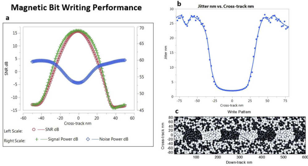
Fig. 5. (a) Sample signal (green) and noise power (blue) used to calculate SNR (red) in the cross-track direction for the case of pure Au ( n=0.06 ) used for the metallic components of the NFT. (b) Jitter plotted along the cross-track position. (c) Corresponding write pattern on media with white grains pointed up, black grains down and gray area non-magnetic material.
