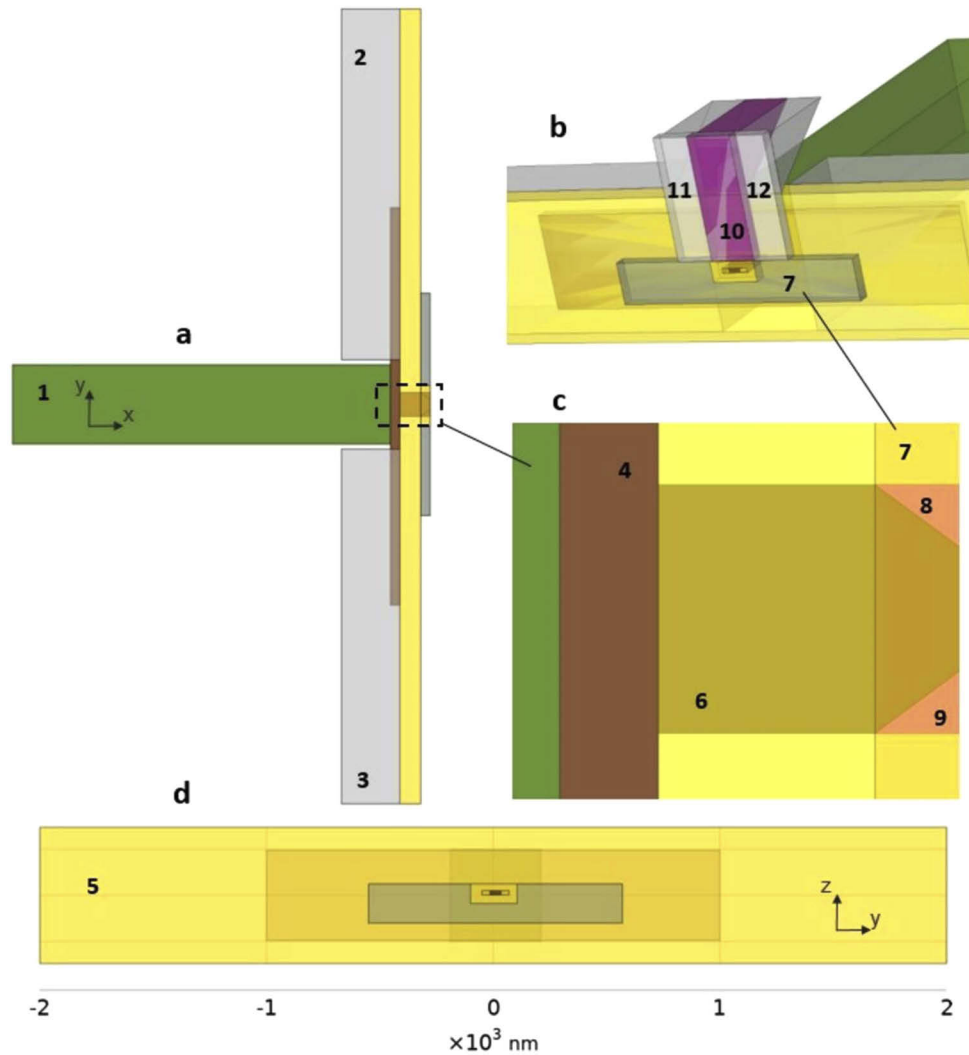
Fig. 6. (a, b, c, d) General, to-scale schematic of fully integrated photonic and plasmonic waveguides with corresponding heatsink additions and other components (numbered). Corresponding dimensions are listed in Table 3 along with material parameters in Table 4. The air-bearing (ABS) section of the MIM (7) may have a hard encasement (optional gray region) in lieu of extended Au or Au alloy. The entire structure is cladded in \text{SiO}_2 .
