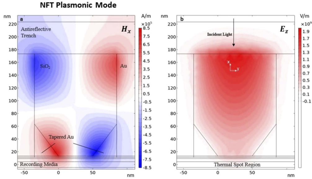
Fig. 3. Planar cross-section [similar to Fig. 2(b)] taken thru the center of insulator layer of the MIM resonator showing excitation of an antisymmetric SP mode with the magnetic field component ( H_x ) in (a) and the electric field component ( E_z ) in (b) which both dominate in magnitude compared to other components. The 0-point on the x-axis is the same 0-point in Fig. 4 while the 0-point on the y-axis corresponds to the center of the magnetic recording layer.
