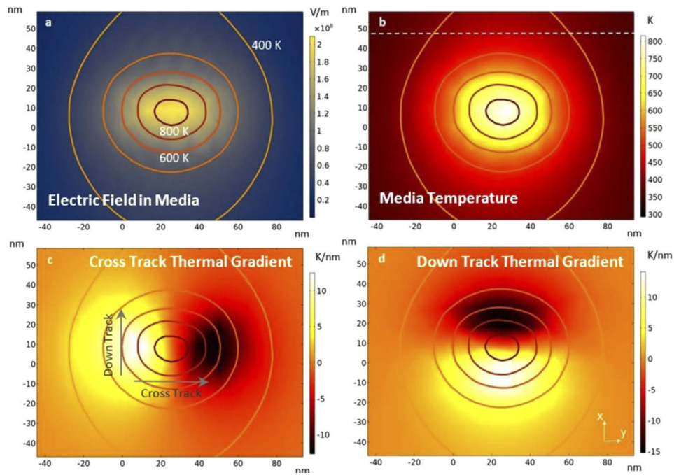
Fig. 4. Planar cross-section taken from the center of the magnetic media layer showing profiles for the normalized electric field (a), the temperature (b), along with the cross (c) and down (d) track temperature gradients. All profiles have the same temperature contours superimposed on them. The position of the NFT's insulator (corner) is marked by the 0-point and the position of the tip of the write pole is marked with the dashed line shown in (b).
