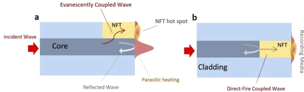
Fig. 1. (a) Schematic demonstrating the evanescent coupling of a dielectric waveguide mode with a plasmonic NFT mode. The evanescent tail of the mode within the dielectric core is the source of excitation of the plasmonic mode. The rest of the energy may be reflected back to the laser or transmitted to the recording medium causing unwanted heating and possible damage away from the bit-writing region. Hence, additional components need to be added to avoid parasitic heating (red peaks). (b) Directly coupling the photonic mode within the core to the NFT allows energy to be dissipated via heatsinking of the device while reducing the amount of the reflected wave which reaches the recording media.
