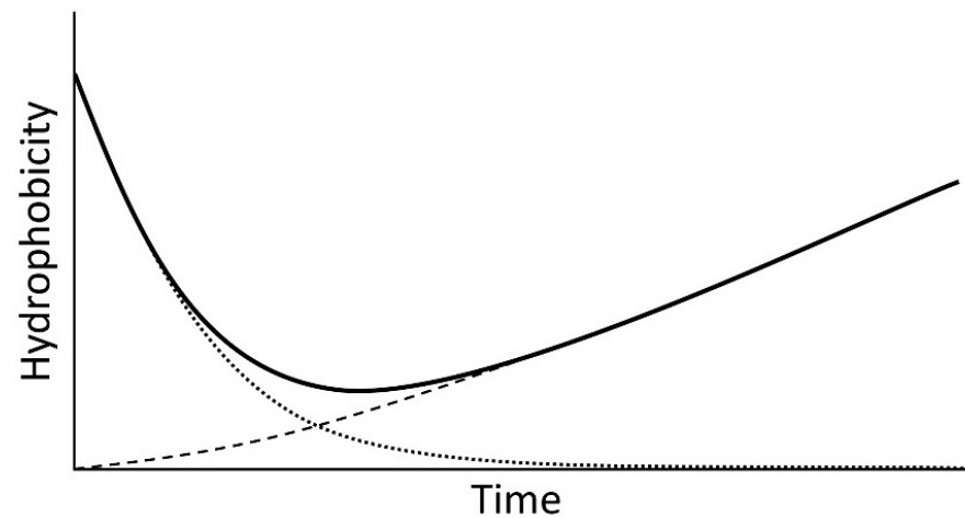
Figure 6. Hypothesized long-term changes in soil water repellence [83]. Solid line: overall response; dotted line: short-term changes generated from fire; dashed line: long-term changes induced by increased biotic activity.
