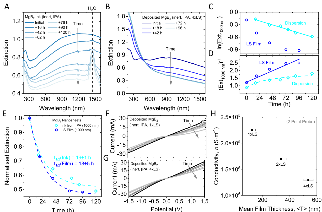
Figure 5. Nanomaterial stability. (A, B) Change in the extinction of liquid exfoliated MgB 2 nanoplatelets in dispersion (A) and after thin film deposition on optical glass (B) as a function of time exposed to ambient conditions. In both cases, a systematic decrease in the overall response is observed for all wavelengths above 450 nm, while the signal below 450 nm undergoes changes in the spectral profile and shows an increased optical density in the UV region, which is indicative of oxide formation. Further, a peak that can be attributed to water forms over time in the nanosheet ink. (C, D) Kinetic plots for rate law analysis of the extinction measurements shown in panels (A, B). Panel (C) shows the change in the natural logarithm of the optical density at 1000 nm, and panel (D) shows the inverse optical density at 1000 nm as a function of time. While the lines indicate a reasonable agreement with a first-order rate law for the dispersed nanomaterial (C) and a second-order rate law for the deposited material (D), the analysis is not unambiguous and is discussed in further detail in the SI. (E) Change in the extinction of the nanosheet ink and thin film at 1000 nm as a function of time. The data can be described by an empirical exponential fit, which allows determination of the material's half-life. The data for both individual data sets agrees well, and fitting suggests a nanomaterial half-life of 19 \pm 1 h and 18 \pm 5 h for the nanosheet ink and thin film, respectively. (F, G) I – V characteristics as a function of time for two sets of samples measured after deposition of a single layer (F) and after deposition of 4 layers (G). In both cases, similar systematic changes are observed: the initial ohmic response changes to a more rectifying transport behavior, which is consistent with the formation of an oxide layer. (H) Conductivity of the same MgB 2 films measured as a function of the mean film thickness determined by profilometry at different points across the substrate. A decrease in the conductivity is observed with increasing film thickness, which is counterintuitive, and may be attributed to surface oxidation of the nanomaterial during the processing steps.
