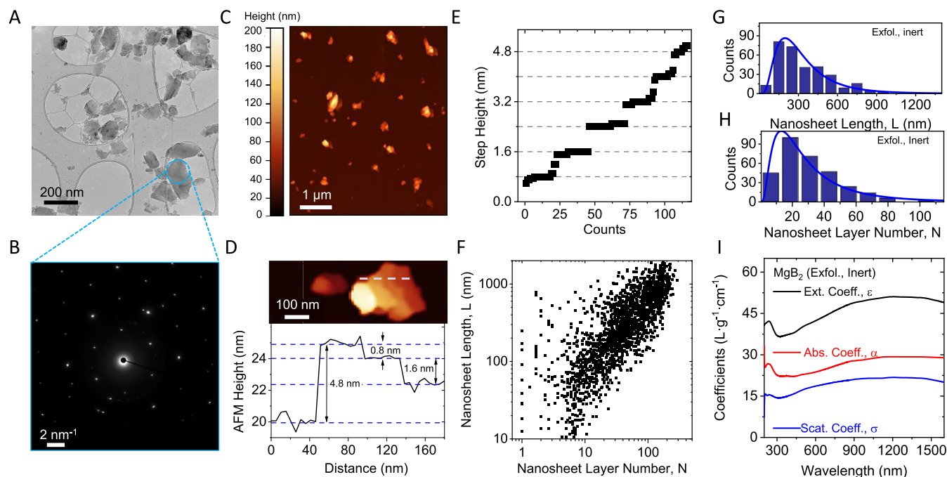
Figure 3. Quantitative characterization of MgB 2 nanoplatelets prepared under inert conditions. (A) Bright-field TEM image of drop cast MgB 2 nanoplatelets. A distribution of different sizes is observed, similar to the nanomaterials observed in the SEM. (B) SAED for the triangular particle in panel (A). The probed region is indicated by the dashed circle and demonstrates the reasonable crystallinity of the nanomaterial. (C) Overview AFM image of MgB 2 nanosheets. Particles of a similar size and shape to those seen in TEM are observed. (D, E) Conversion of the apparent AFM height into the LPE MgB 2 layer number using line profiles on nanoparticles with suitable steps and terraces. An example is shown in panel (D), while the statistical analysis of suitable steps is presented in panel (E). The data are sorted in ascending order, revealing discrete steps of \sim 0.8 nm. (F) Scatter plot of the overall nanosheet size and thickness distribution measured using statistical AFM. The data includes the size and thickness of over 1500 nanoparticles with an average length/thickness aspect ratio of \sim 12.9 . (G, H) Histograms of the lateral nanosheet size (G) and the layer number (H) from statistical analysis of line profiles on individual nanosheets. (I) Optical extinction (black), absorbance (red), and scattering (blue) coefficient spectra for MgB 2 nanoparticles exfoliated under inert conditions.
