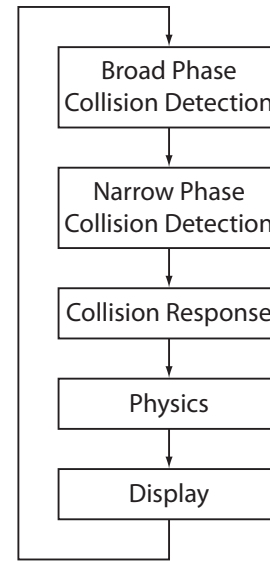
Figure 6: The software application's central program loop.
