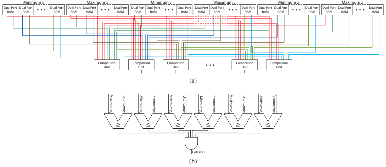
Figure 4: (a) The comparator module. (b) The implementation of each comparison unit.
