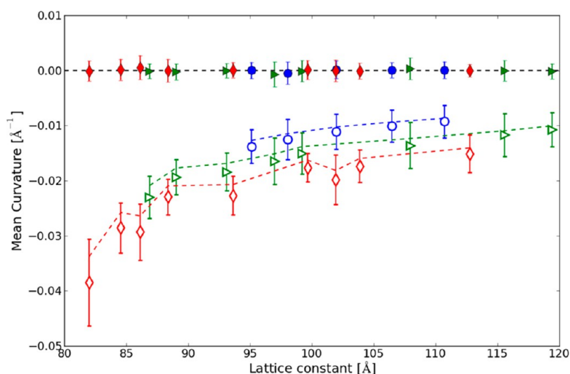
Figure 1. Mean curvature of the membrane midplane (full symbols) and interface (empty symbols), averaged over the unit cell, are shown as a function of the lattice constant for different lipids (blue circles, 7.7 MAG; green right triangles, 7.9 MAG; and red diamonds, 9.9 MAG). The dashed lines are the theoretical estimates from eq 7 as described in the text. The error bars measure the width of the distributions of the mean curvatures.
