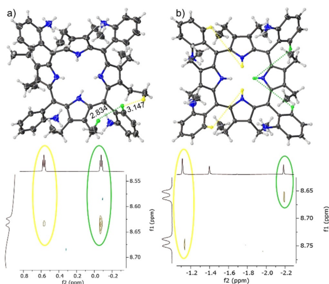
Figure 7. The key examples of ^1\text{H} - ^1\text{H} ROESY correlations of P1-BSA : a) in \uparrow\uparrow\uparrow the ortho - to \text{CH}_3 correlation strength dependent on the distance ( \text{\AA} ) shown by the \alpha_4 - P1-BSA crystal structure; b) illustration of \uparrow\uparrow\downarrow atropisomer highlighting the long-distance ortho - to N-H correlation.
