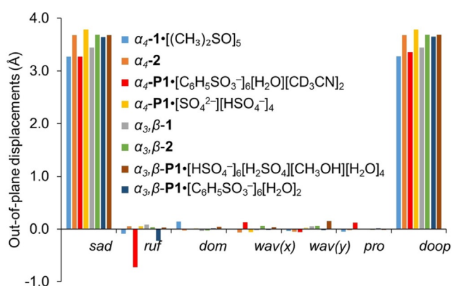
Figure 11. Illustration of the out-of-plane normal-coordinate structural decomposition results for the \uparrow\uparrow\uparrow\uparrow and \uparrow\uparrow\uparrow\downarrow atropisomers of free base 1, Ni II 2 and protonated P1 with H 2 SO 4 and BSA forms.
