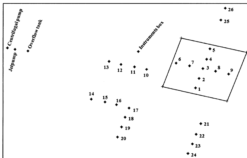
Figure 4 – Surface settlement plates and stand pipes distribution
