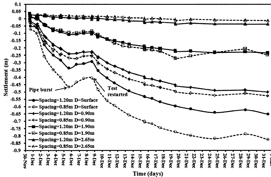
Figure 5 – Ground settlement at different depths for both spacing subareas
