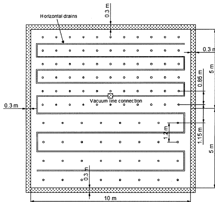
Figure 3 - Horizontal drains arrangement
