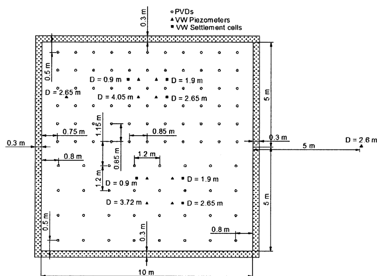
Figure 2 - PVD and subsurface instrumentation arrangement
