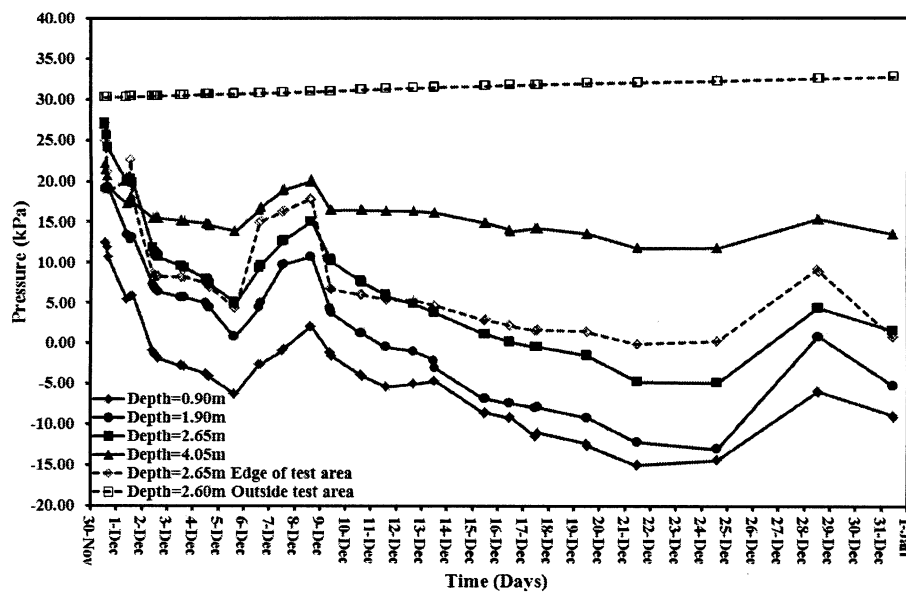
Figure 6 – Pore-water pressure variation for 0.85m PVD spacing subarea
