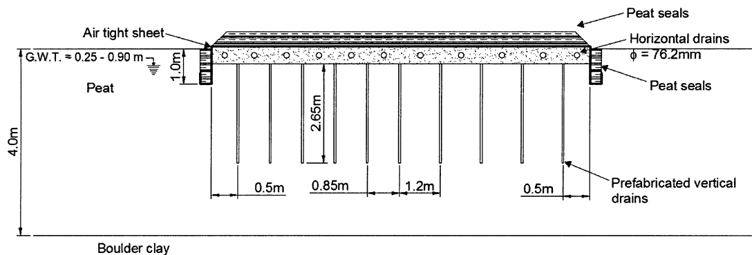
Figure 1 - Cross section of TCD/NRA vacuum preloading field trial
