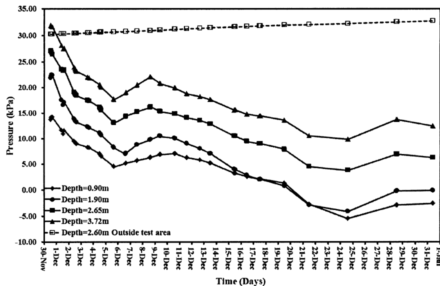
Figure 7 – Pore-water pressure variation for 1.20m PVD spacing subarea
