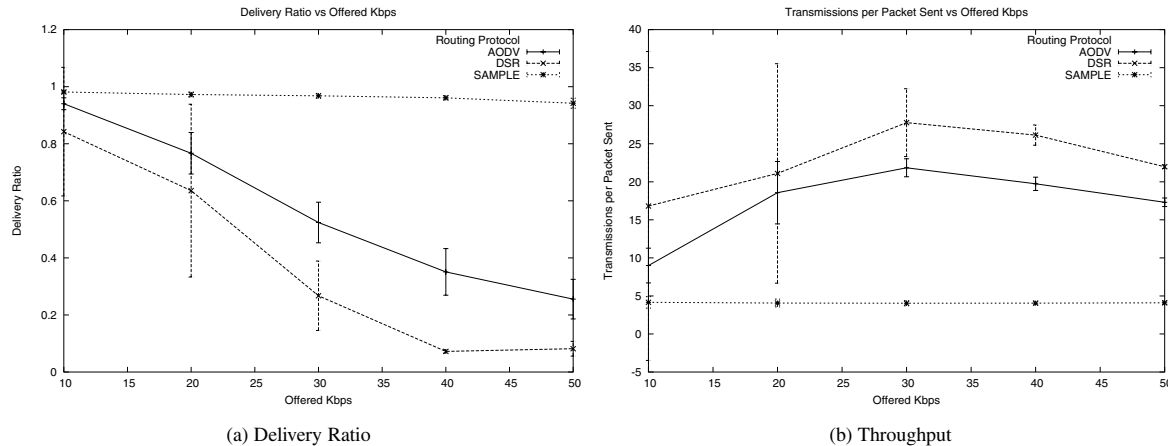
Figure 3. SAMPLE Performance with Varying Load. 64 byte packets
