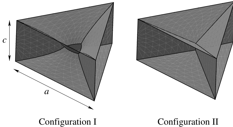
Fig. 1: Surface Evolver simulations of the equilibrium arrangements of soap films in a wire frame in the shape of a triangular prism. Configuration I with the triangular face in the centre is unstable for an axial ratio c/a > 0.487 .
