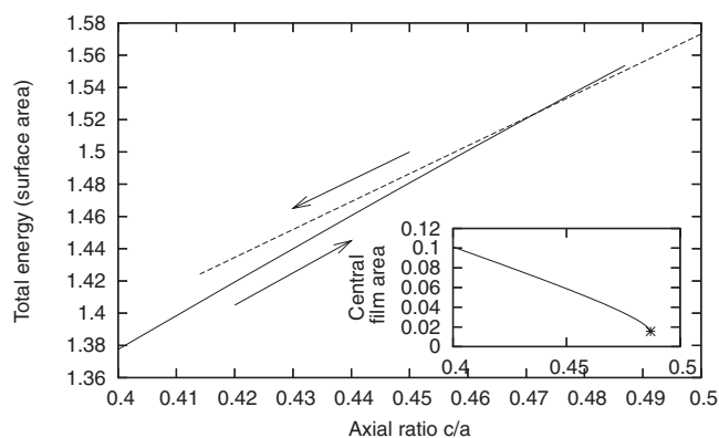
Fig. 3: Surface Evolver calculations show that there are two stable configurations for 0.413 < c/a < 0.487 (solid line: configuration I, dashed line: configuration II). The inset shows that the area of the triangular face of configuration I is non-zero at the point of instability, c/a = 0.487 . There should also be an unstable equilibrium solution for c/a < 0.487 , but this is not determined by the present calculations. (In the simulations a was kept constant, a = 1 .)
