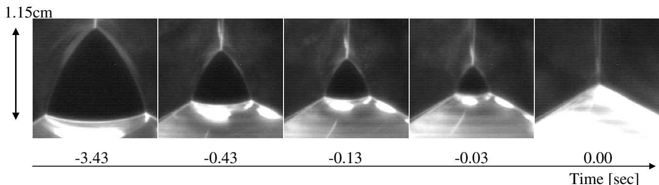
Fig. 4: Snapshots of the vanishing triangular face of configuration I. Note the acceleration of the rate of decrease in area. (The photographs correspond to run 1 of fig. 5.)
