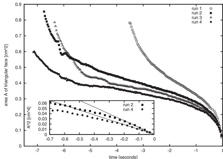
Fig. 5: Experimental data for the decrease in area A of the central triangular face of the unstable configuration I (fig. 1) with time. The face was created by blowing against one of the vortices the central Plateau border of configuration II for a frame with axial ratio c/a \simeq 0.5 , where a = 6.2 cm. (A rescaling of the minimum area of the triangular face of fig. 3 by a^2 gives A = 0.594 .) Run 1 to 4 correspond to soap films that have been allowed to drain for an increasing amount of time (up to three minutes), before the experiment was performed. The time origin of the data has been shifted so that the vanishing of the triangular face occurs at time equals zero for all runs. The inset shows that the square of the area of the triangle shrinks linearly close to the disappearance of the face.
