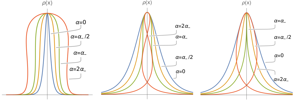
Figure 1: Left: Case B, \mu = 0 , \alpha_- = -32 , displaying formation of shockwave solution for negative \alpha . Centre: Boundary case of B and C, \mu = -1/4 , \alpha_- = -8 , example of competing shockwave and narrowing behaviours creating a double-loop solution. Right: Case C, \mu = -0.6 , \alpha_- = -2.76817 , soliton is becoming singular at \alpha_- , after which it forms a loop.
